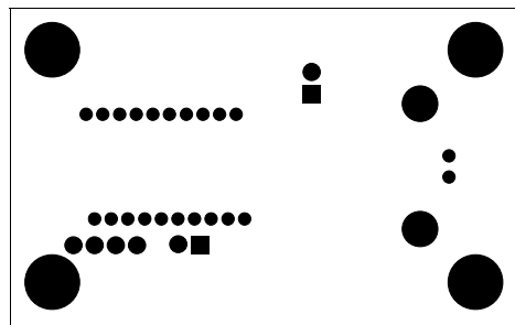
Bottom Solder Mask
