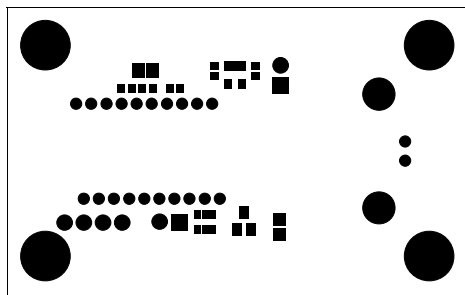
Top Solder Mask
