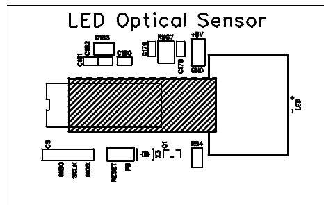
Top Silkscreen
