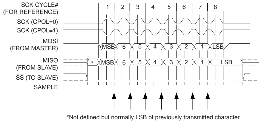
Figure 40. SPI Transfer Format with CPHA = 1
