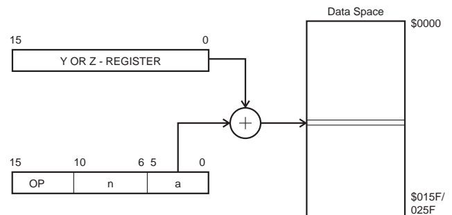
Figure 12. Data Indirect with Displacement
