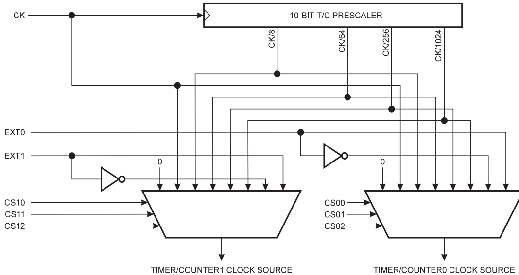
Figure 28. Prescaler for Timer/Counter0 and 1
