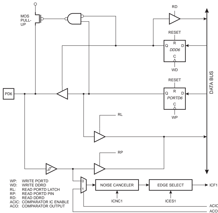
Figure 61. PORTD Schematic Diagram (Pin PD6)
