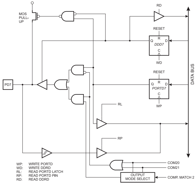
Figure 62. PORTD Schematic Diagram (Pin PD7)
