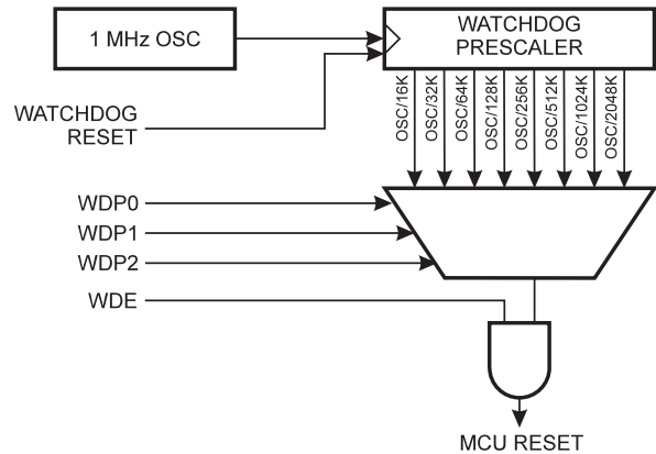
Figure 36. Watchdog Timer
