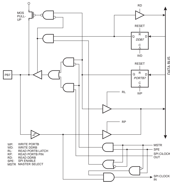
Figure 53. PORTB Schematic Diagram (Pin PB7)
