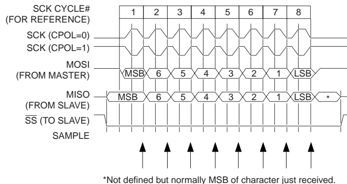
Figure 39. SPI Transfer Format with CPHA = 0
