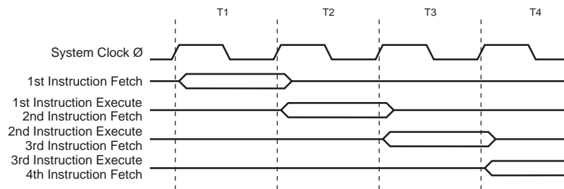
Figure 19. The Parallel Instruction Fetches and Instruction Executions
