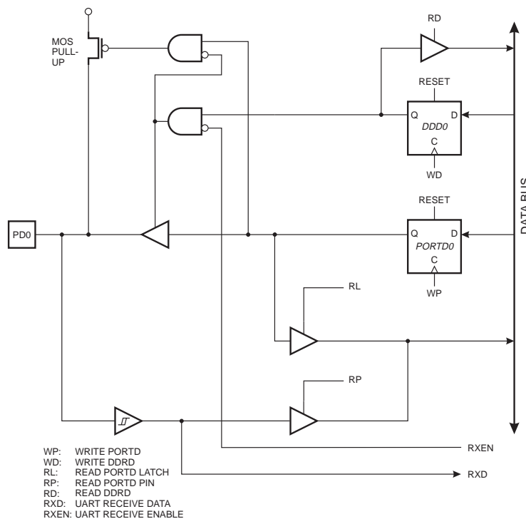
Figure 57. PORTD Schematic Diagram (Pin PD0)
