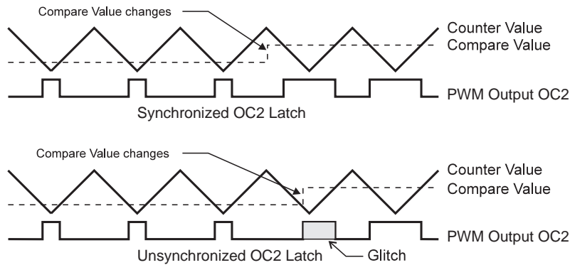
Figure 35. Effects of Unsynchronized OCR Latching
