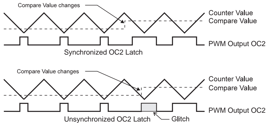
Figure 33. Effects of Unsynchronized OCR1 Latching
