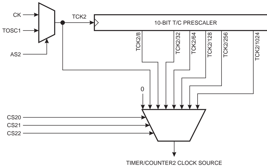
Figure 29. Timer/Counter2 Prescaler
