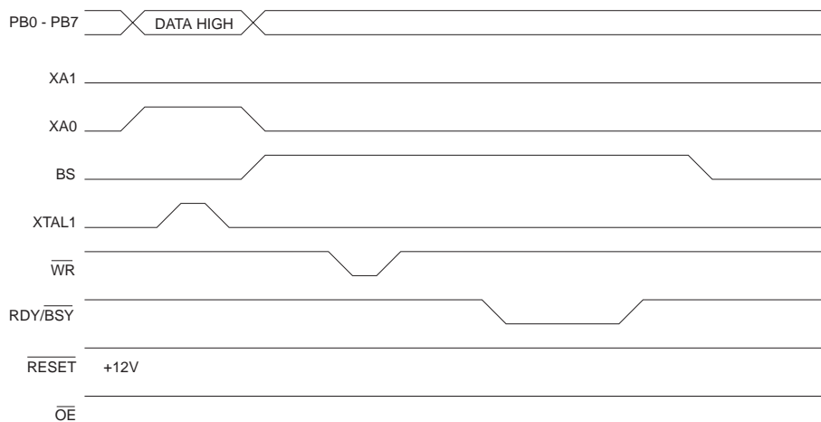
Figure 65. Programming Flash High Byte
