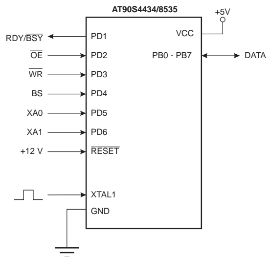
Figure 63. Parallel Programming
