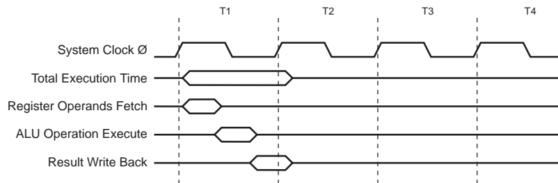
Figure 20. Single Cycle ALU Operation
