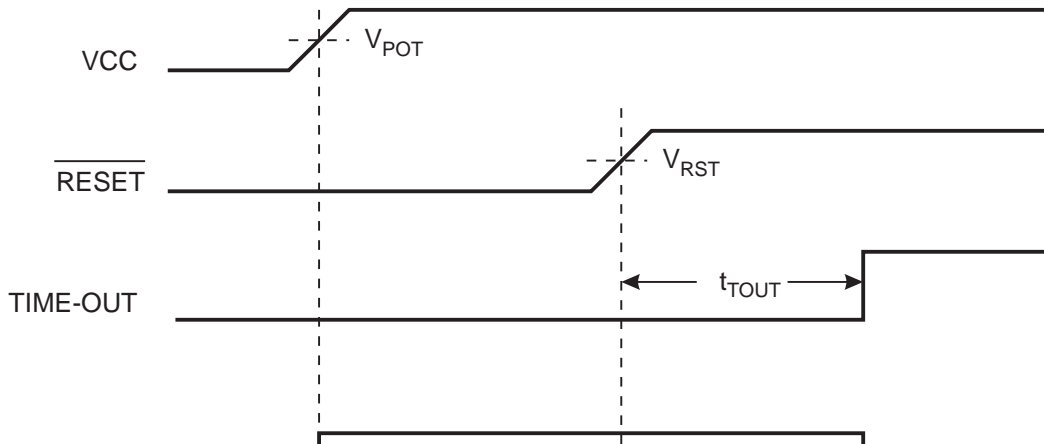
Figure 25. MCU Start-Up, \overline{\text{RESET}} Controlled Externally
