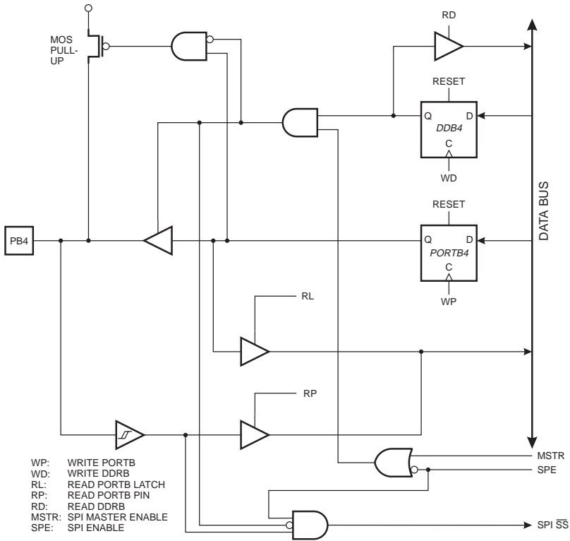
Figure 50. PORTB Schematic Diagram (Pin PB4)
