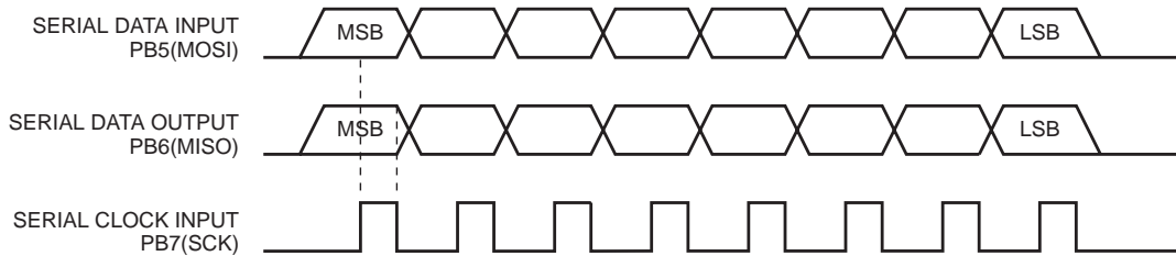
Figure 68. Serial Programming Waveforms
