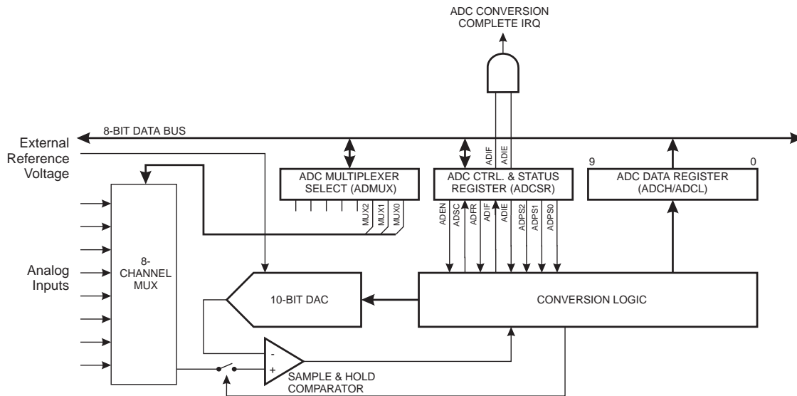
Figure 45. Analog to Digital Converter Block Schematic
