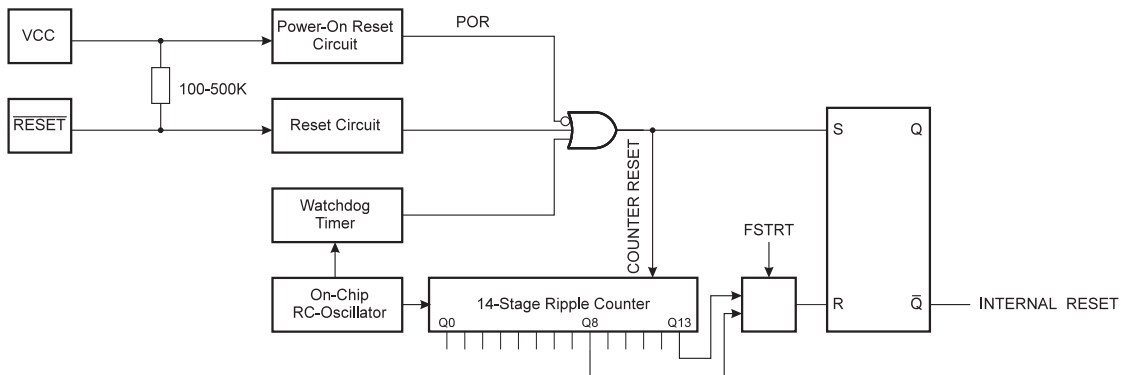
Figure 22. Reset Logic
