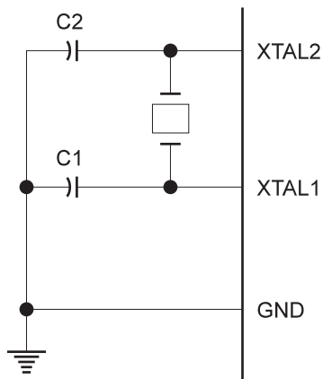
Figure 1. Oscillator Connections
