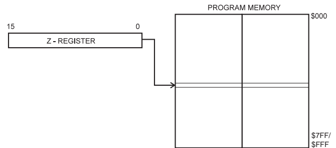
Figure 17. Indirect Program Memory Addressing
