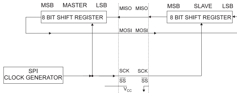
Figure 38. SPI Master-Slave Interconnection
