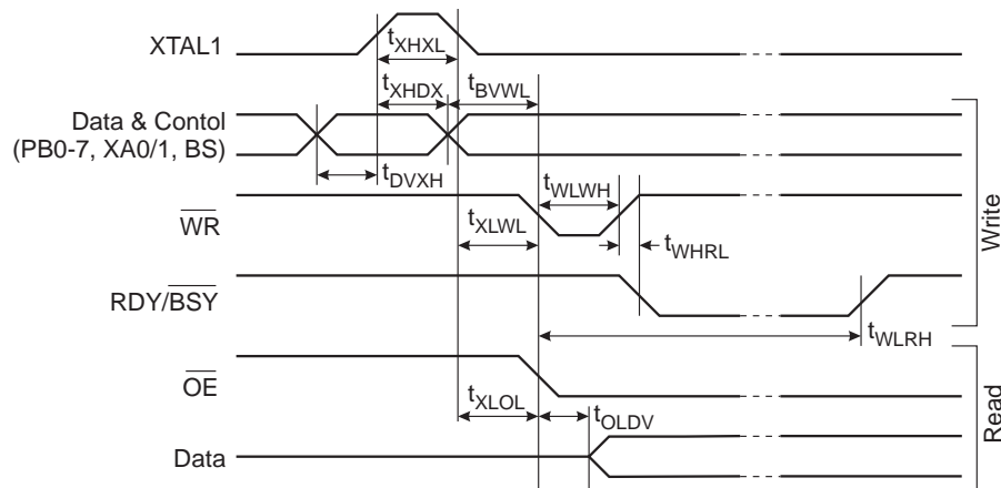
Figure 66. Parallel Programming Timing
