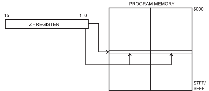
Figure 16. Code Memory Constant Addressing
