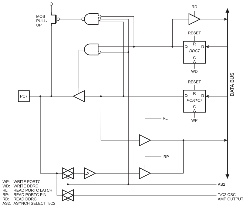
Figure 56. PORTC Schematic Diagram (Pins PC7)
