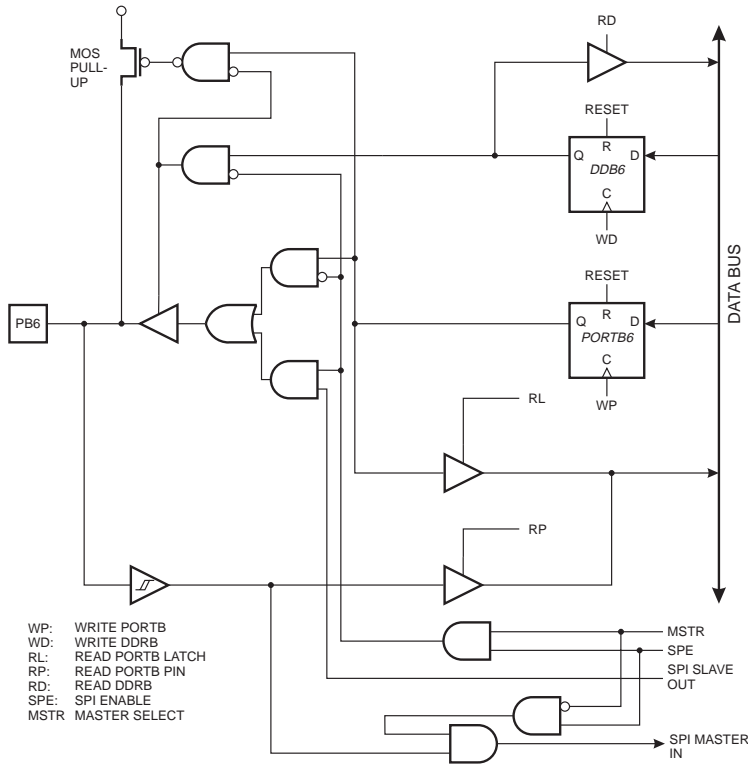
Figure 52. PORTB Schematic Diagram (Pin PB6)
