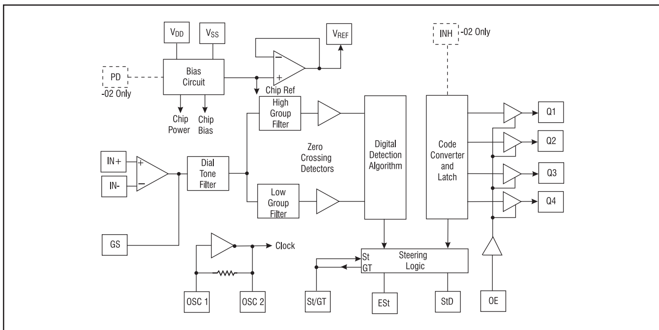
Figure 2 Block Diagram
