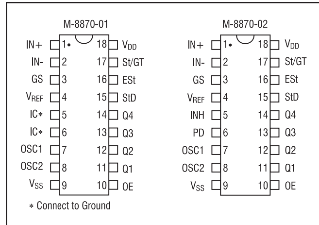
Figure 1 Pin Connections
