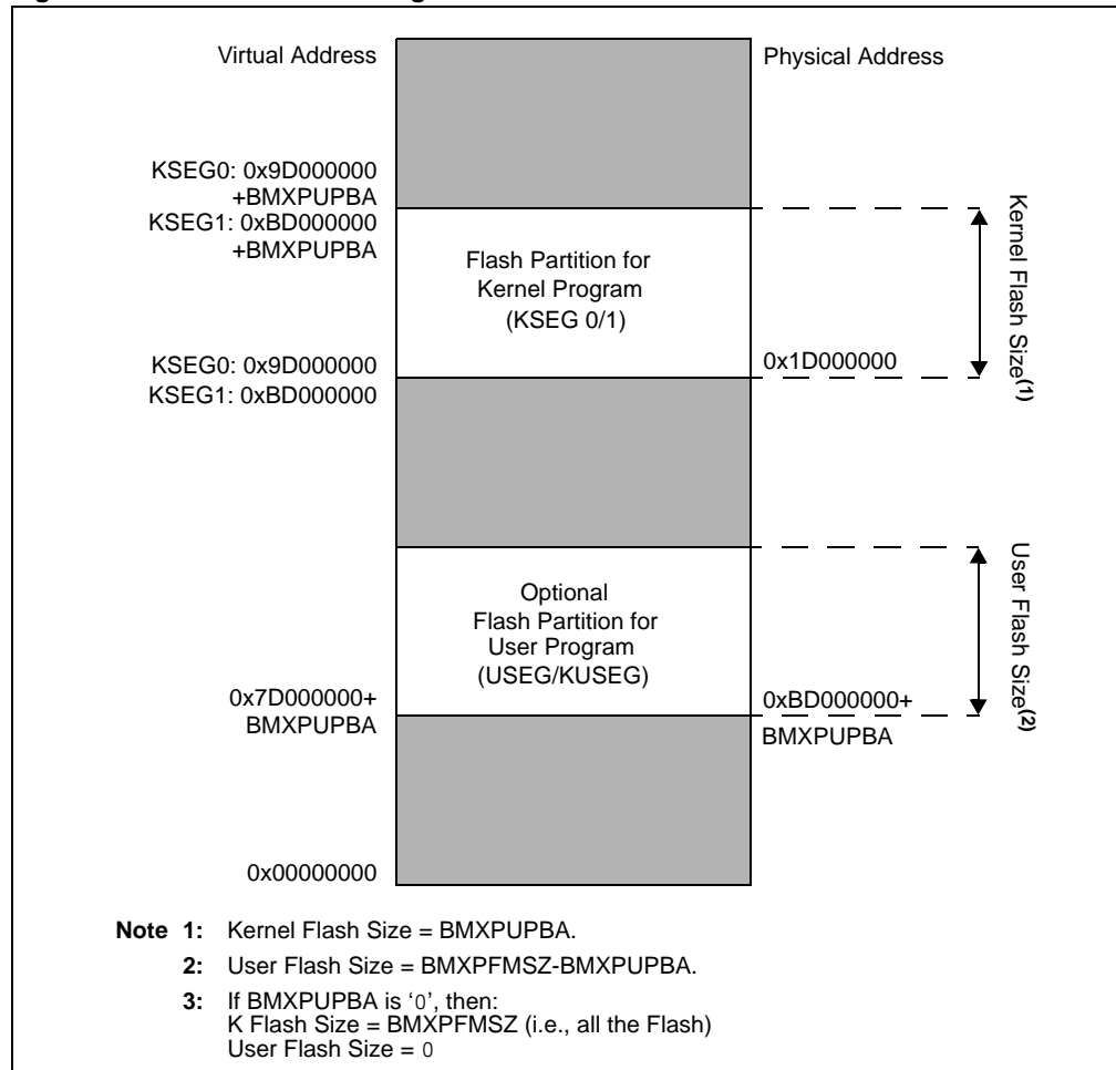
Figure 3-3: Flash Partitioning
