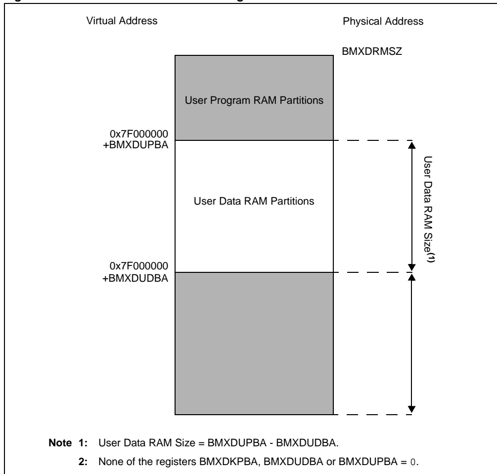
Figure 3-8: User Data RAM Partitioning
