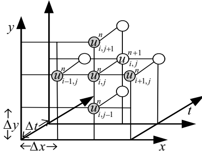
Fig. 1. FD scheme graphical representation
