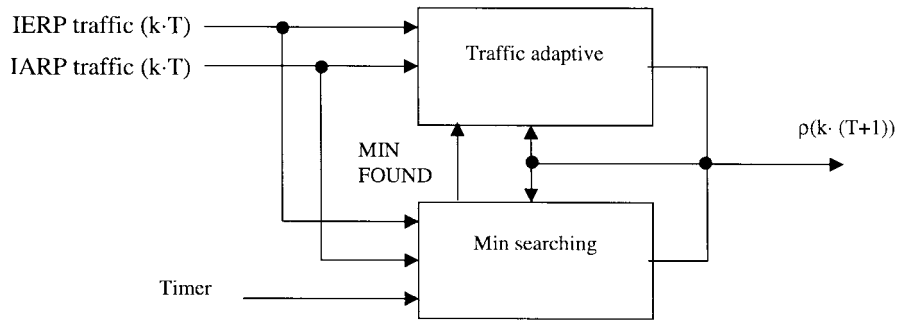
Fig. 12. A hybrid min search/traffic adaptive zone radius estimator.
