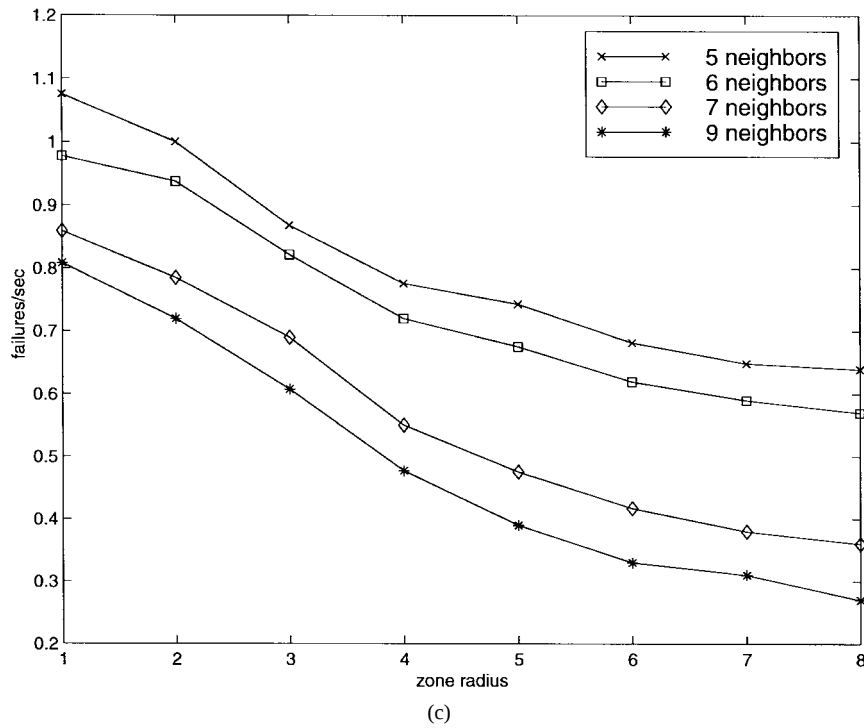
Fig. 8. (Continued.) Route failure rate traffic (normalized to node velocity). (c) N = 1000 nodes.
