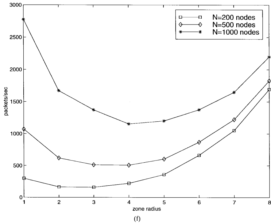
Fig. 9. (Continued.) ZRP traffic per node (6.0 neighbors, v = 0.5 neighbors/s). (e) R_{\text{route\_usage}} \ll R_{\text{route\_failure}} . (f) R_{\text{route\_usage}} \gg R_{\text{route\_failure}} .
