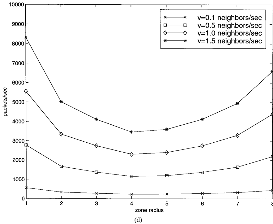
Fig. 9. (Continued.) ZRP traffic per node ( N = 1000 nodes, d = 6.0 neighbors). (c) R_{\text{route\_usage}} \ll R_{\text{route\_failure}} . (d) R_{\text{route\_usage}} \gg R_{\text{route\_failure}} .
