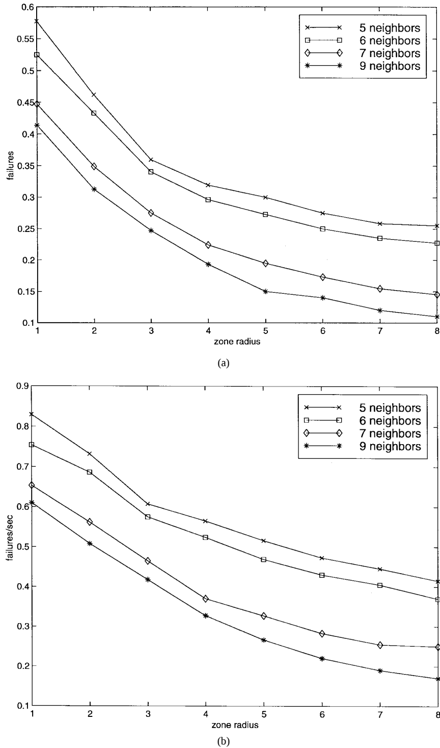
Fig. 8. Route failure rate traffic (normalized to node velocity). (a) N = 1000 nodes. (b) N = 500 nodes.
