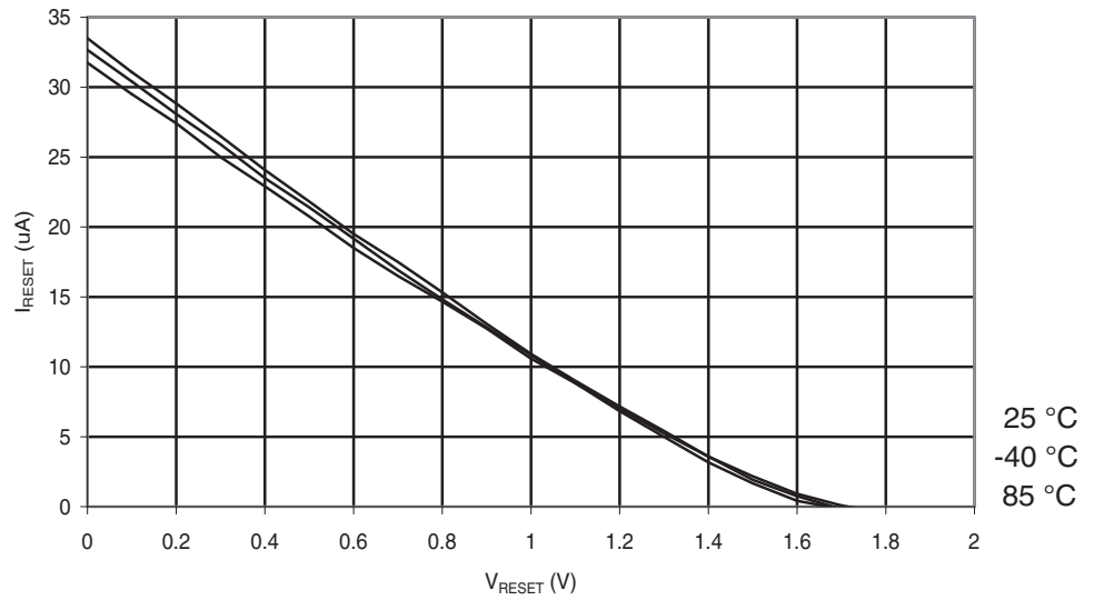
Figure 29-214. ATmega644A: Reset Pull-up Resistor Current vs. Reset Pin Voltage ( V_{CC} = 1.8V ).
