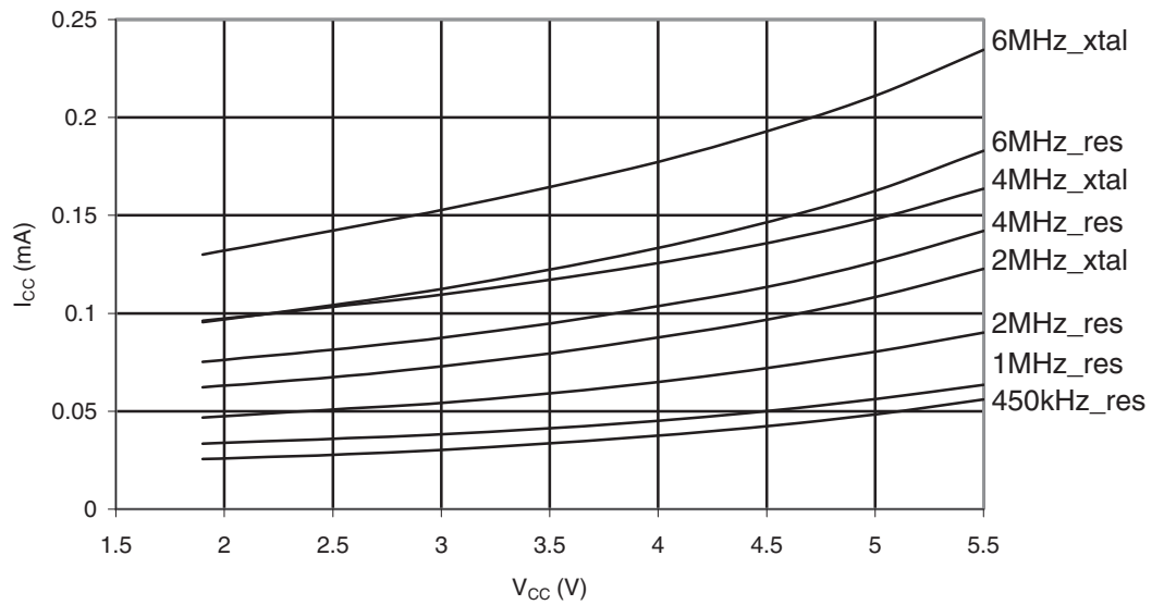
Figure 29-308. ATmega1284: Standby Supply Current vs. V_{CC} (Watchdog Timer Disabled)
