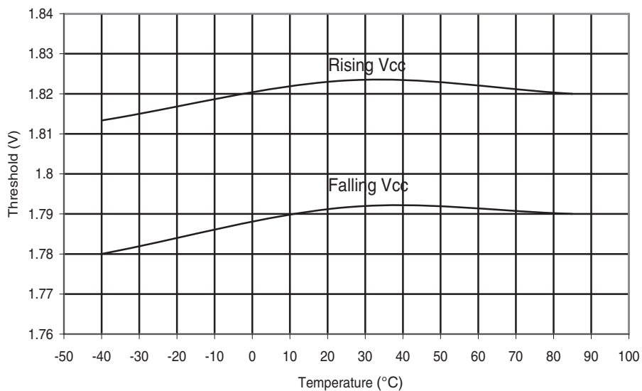
Figure 29-229. ATmega644A: BOD Threshold vs. Temperature ( V_{BOT} = 1.8V )
