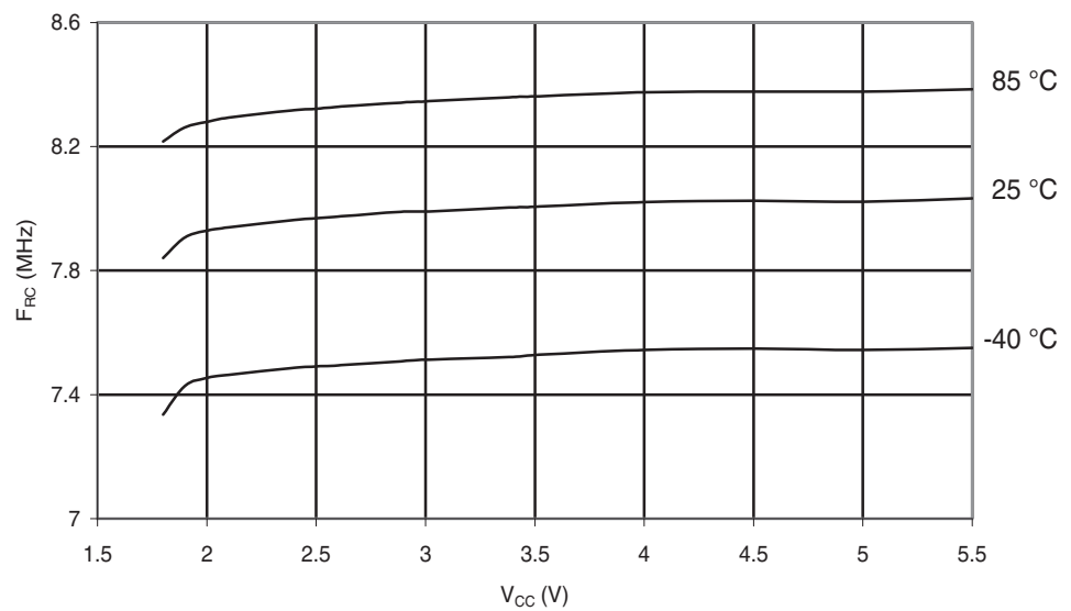
Figure 29-136. ATmega324A: Calibrated 8MHz RC Oscillator vs. V_{CC}
