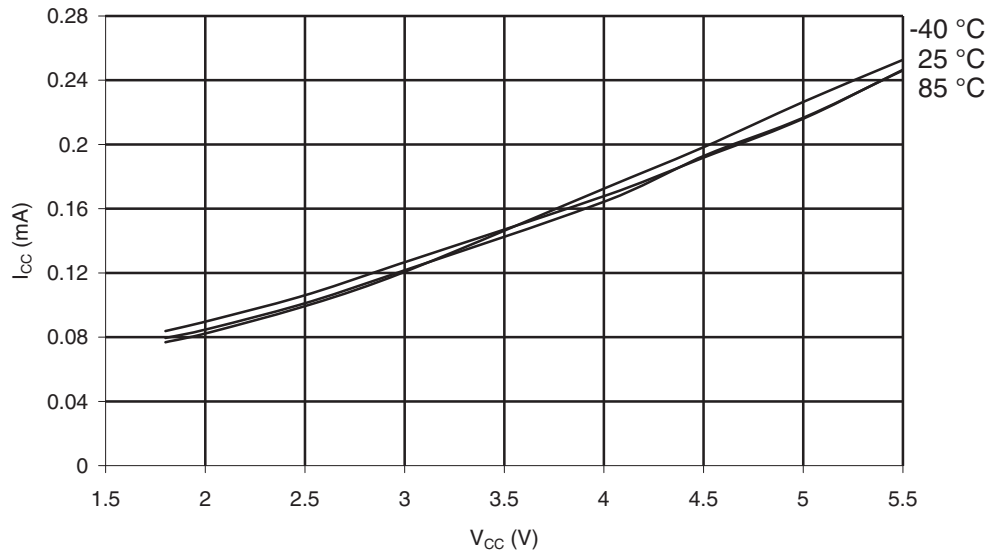
Figure 29-349. ATmega1284P: Active Supply Current vs. V_{CC} (Internal RC Oscillator, 128kHz)
