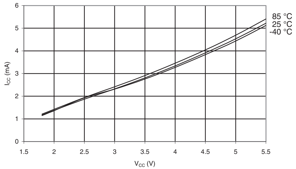
Figure 29-52. ATmega164PA: Active Supply Current vs. V_{CC} (Internal RC Oscillator, 8MHz).
