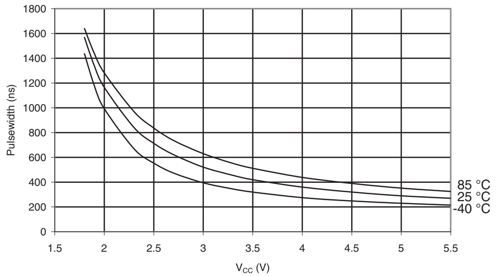
Figure 29-344. ATmega1284: Minimum Reset Pulsewidth vs. V_{CC}
