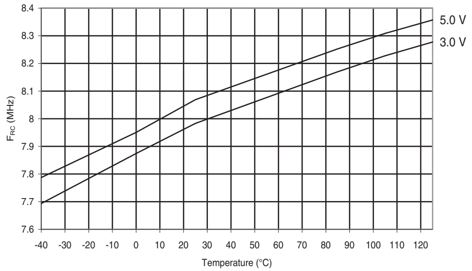
Figure 29-284. ATmega644PA: Calibrated 8MHz RC Oscillator vs. Temperature
