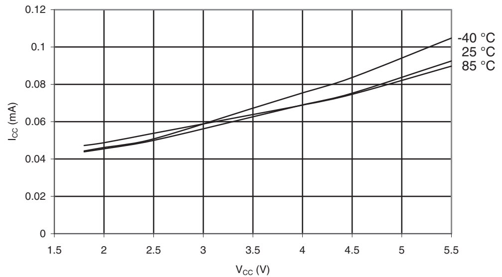
Figure 29-206. ATmega644A: Idle Supply Current vs. V_{CC} (Internal RC Oscillator, 128kHz).
