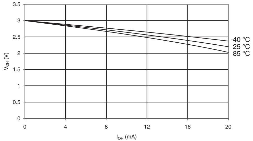
Figure 29-72. ATmega164PA: I/O Pin Output Voltage vs. Source Current ( V_{CC} = 3V ).
