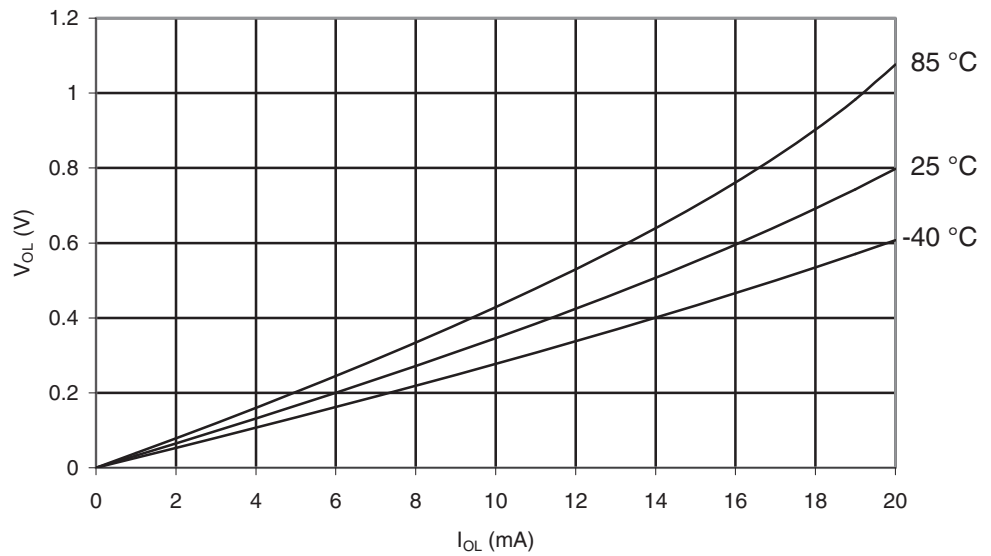
Figure 29-365. ATmega1284P: I/O Pin Output Voltage vs. Sink Current ( V_{CC} = 2.7V )
