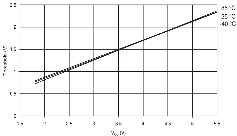
Figure 29-271. ATmega644PA: I/O Pin Input Threshold vs. V_{CC} ( V_{IL} , I/O Pin Read as '0').
