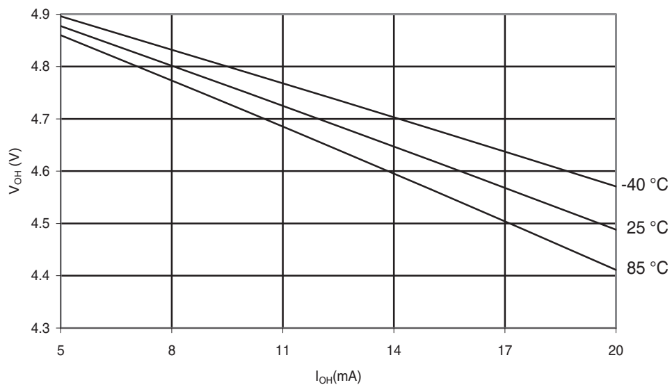
Figure 29-122. ATmega324A: I/O Pin Output Voltage vs. Source Current ( V_{CC} = 5V ).
