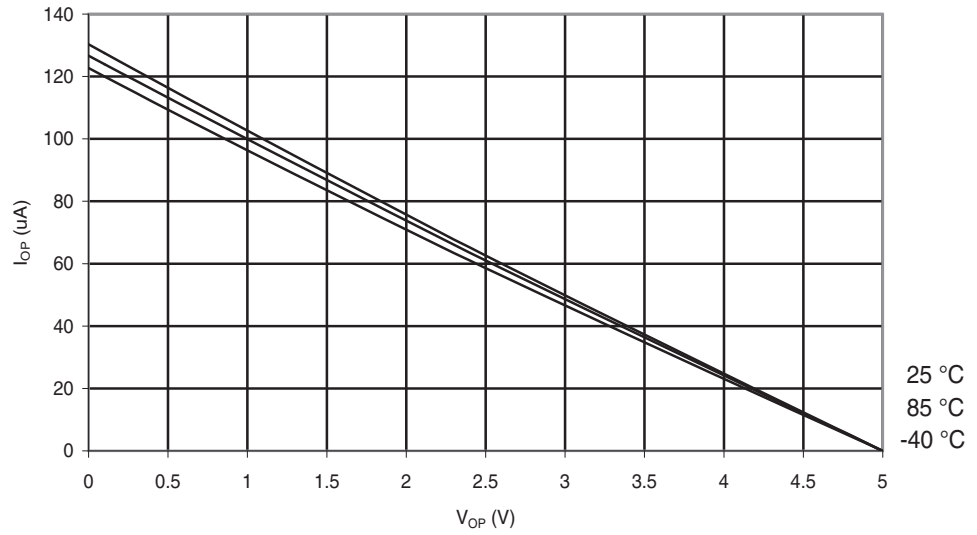
Figure 29-213. ATmega644A: I/O Pin Pull-up Resistor Current vs. Input Voltage ( V_{CC} = 5V ).
