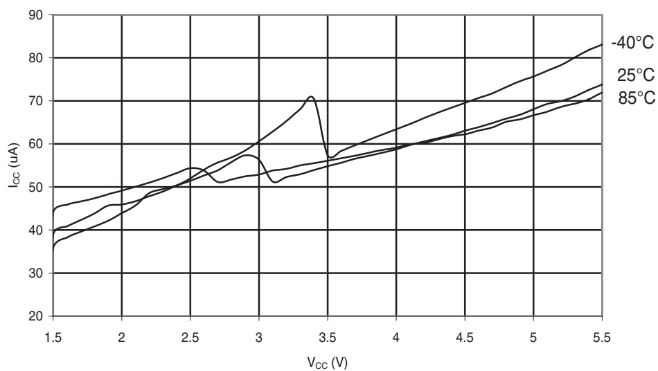
Figure 29-238. ATmega644A: Analog Comparator Current vs. V_{CC}
