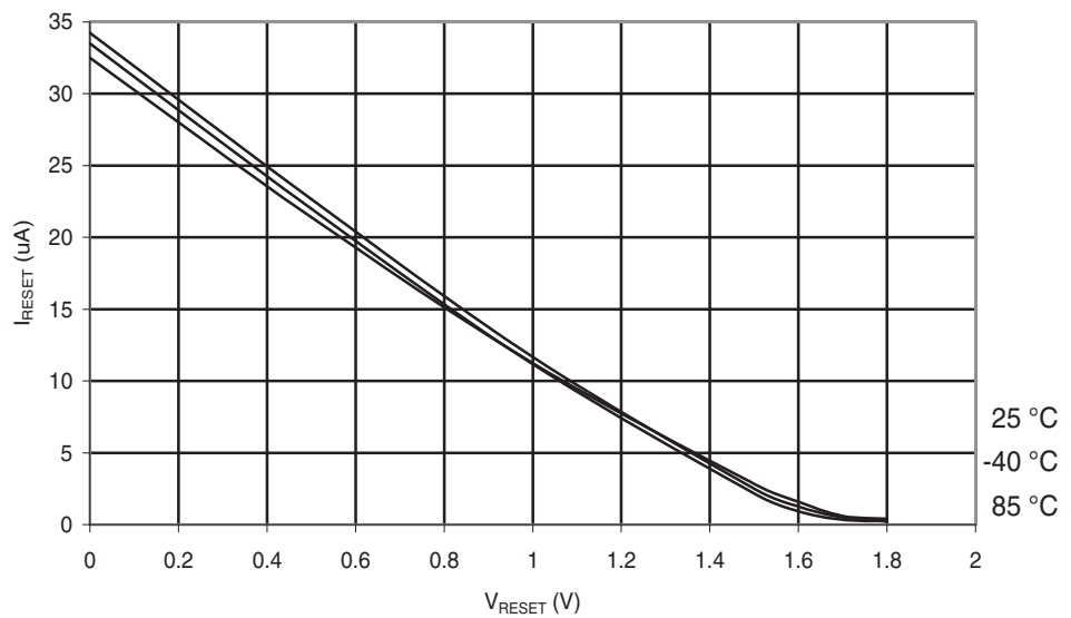
Figure 29-116. ATmega324A: Reset Pull-up Resistor Current vs. Reset Pin Voltage ( V_{CC} = 1.8V ).
