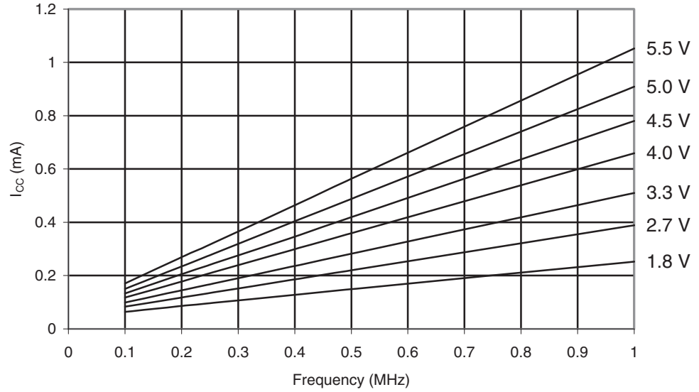
Figure 29-50. ATmega164PA: Active Supply Current vs. Low Frequency (0.1 - 1.0MHz).
