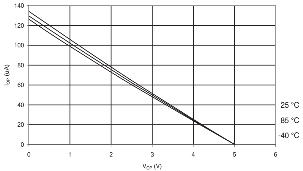
Figure 29-115. ATmega324A: I/O Pin Pull-up Resistor Current vs. Input Voltage ( V_{CC} = 5V ).
