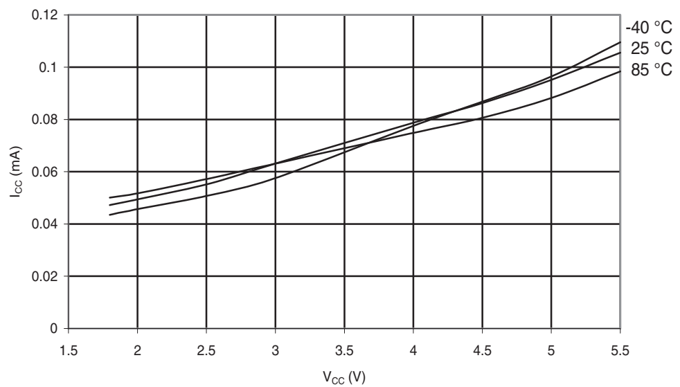
Figure 29-157. ATmega324PA: Idle Supply Current vs. V_{CC} (Internal RC Oscillator, 128kHz).
