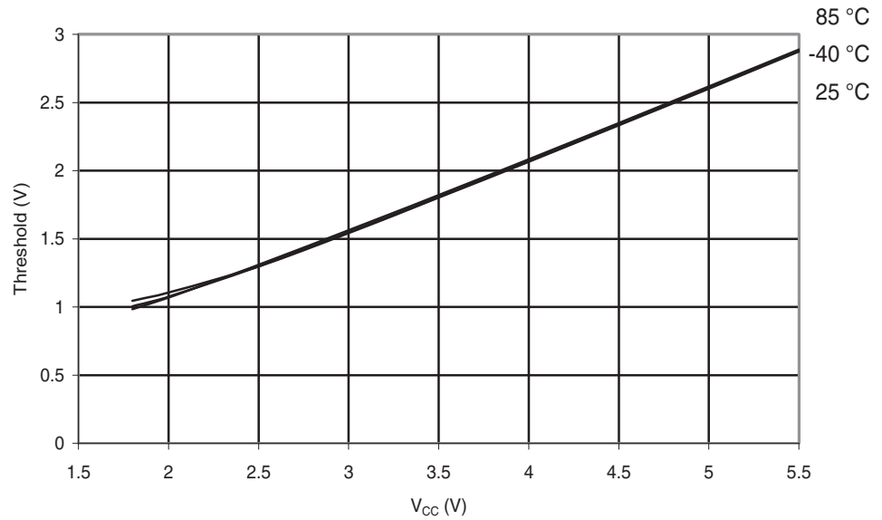
Figure 29-172. ATmega324PA: I/O Pin Input Threshold vs. V_{CC} ( V_{IH} , I/O Pin Read as '1').
