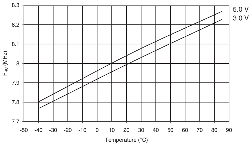
Figure 29-39. ATmega164A: Calibrated 8MHz RC Oscillator vs. Temperature
