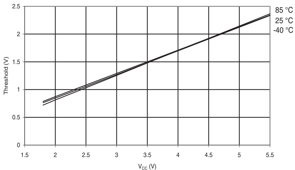
Figure 29-274. ATmega644PA: Reset Pin Input Threshold vs. V_{CC} ( V_{IL} , I/O Pin Read as '0').
