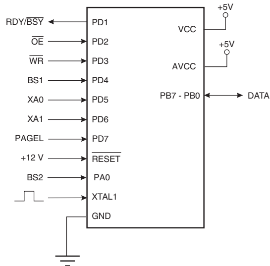
Figure 27-1. Parallel Programming (1)
