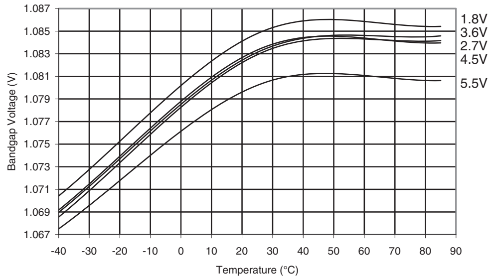
Figure 29-231. ATmega644A: Bandgap Voltage vs. Temperature
