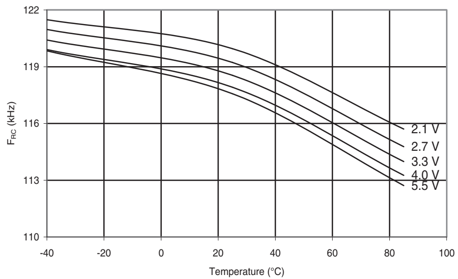
Figure 29-183. ATmega324PA: Watchdog Oscillator Frequency vs. Temperature
