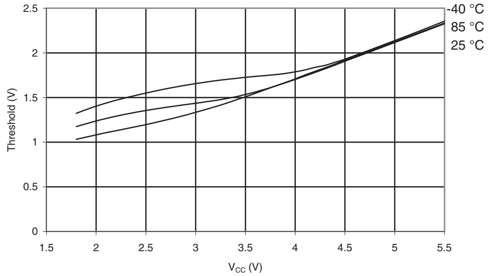
Figure 29-324. ATmega1284: Reset Pin Input Threshold vs. V_{CC} ( V_{IL} , I/O Pin Read as '0')
