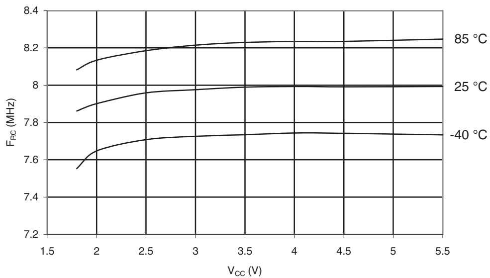
Figure 29-87. ATmega164PA: Calibrated 8MHz RC Oscillator vs. V_{CC}
