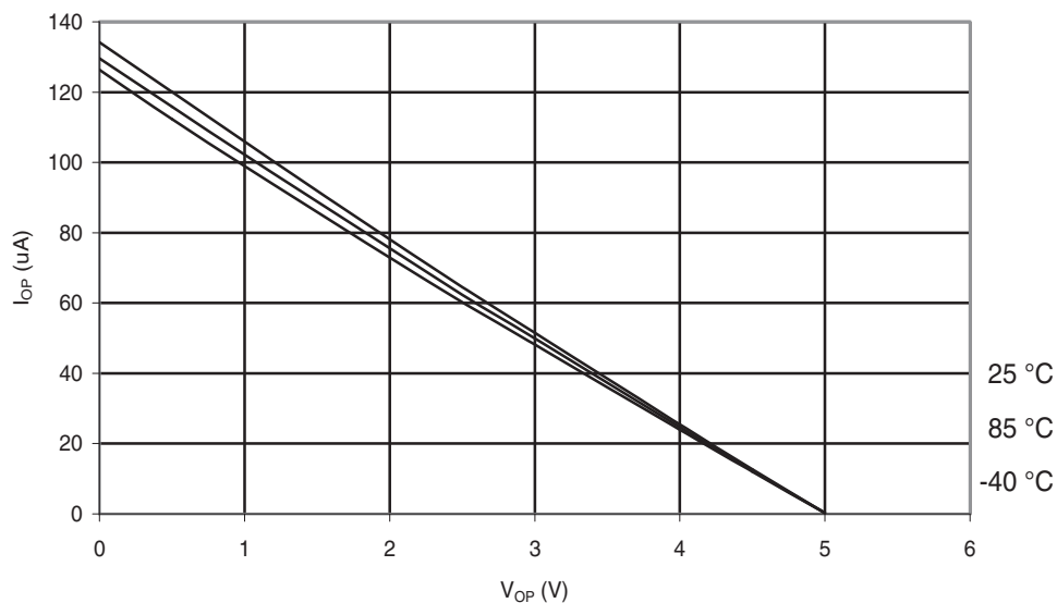
Figure 29-164. ATmega324PA: I/O Pin Pull-up Resistor Current vs. Input Voltage ( V_{CC} = 5V ).
