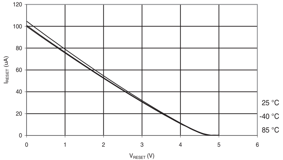
Figure 29-167. ATmega324PA: Reset Pull-up Resistor Current vs. Reset Pin Voltage ( V_{CC} = 5V ).
