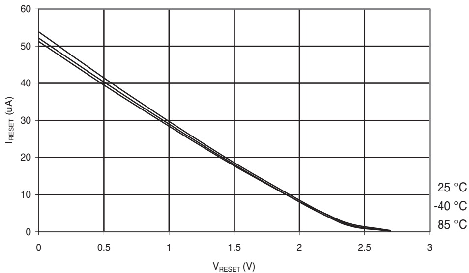
Figure 29-117. ATmega324A: Reset Pull-up Resistor Current vs. Reset Pin Voltage ( V_{CC} = 2.7V ).
