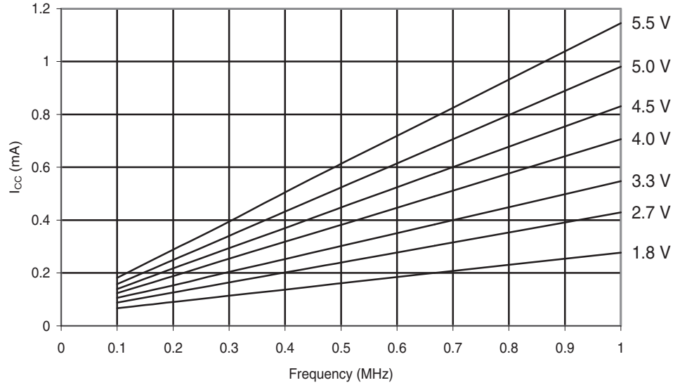
Figure 29-148. ATmega324PA: Active Supply Current vs. Low Frequency (0.1 - 1.0MHz).
