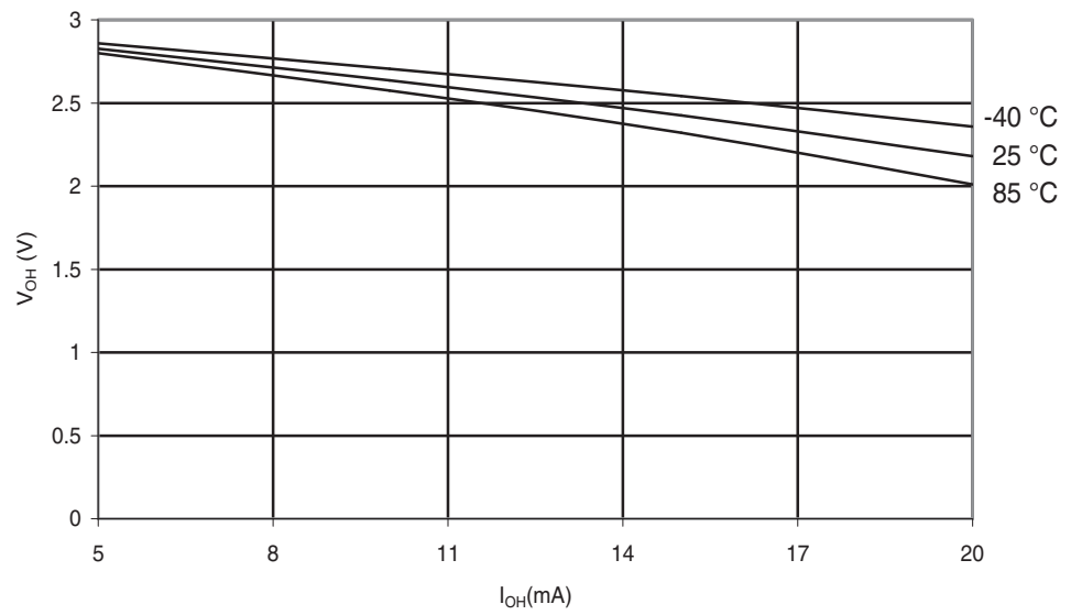
Figure 29-170. ATmega324PA: I/O Pin Output Voltage vs. Source Current ( V_{CC} = 3V ).
