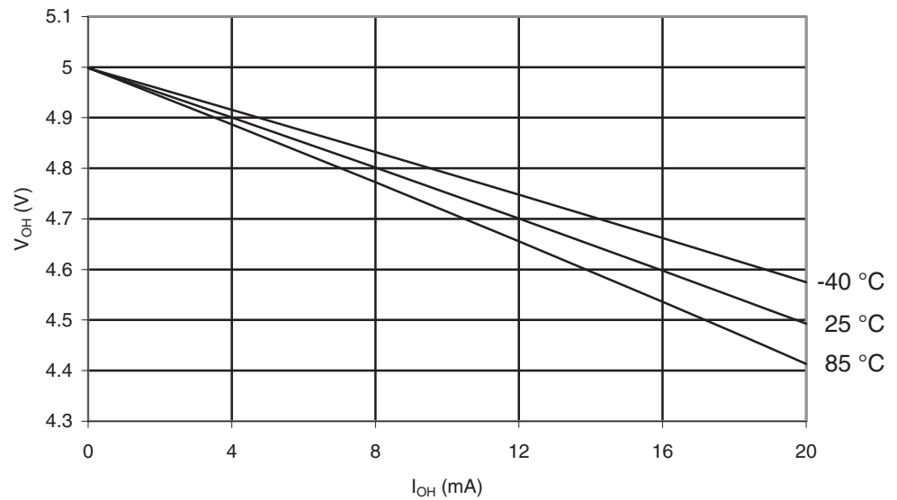
Figure 29-24. ATmega164A: I/O Pin Output Voltage vs. Source Current ( V_{CC} = 5V ).
