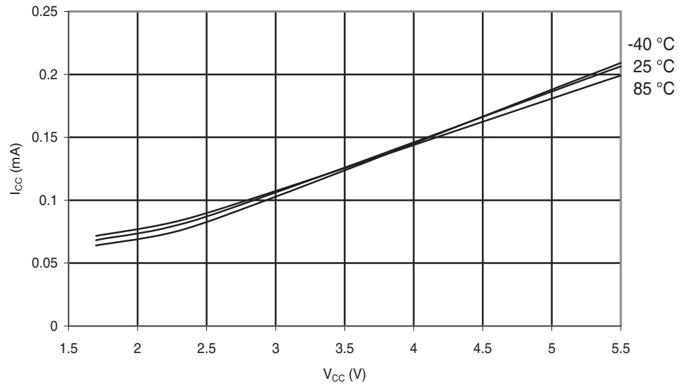
Figure 29-152. ATmega324PA: Active Supply Current vs. V_{CC} (Internal RC Oscillator, 128kHz).
