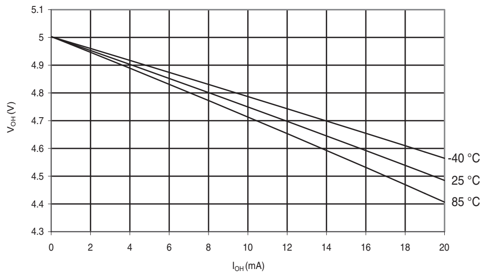
Figure 29-269. ATmega644PA: I/O Pin Output Voltage vs. Source Current ( V_{CC} = 5V ).
