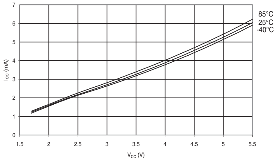
Figure 29-249. ATmega644PA: Active Supply Current vs. V_{CC} (Internal RC Oscillator, 1MHz).
