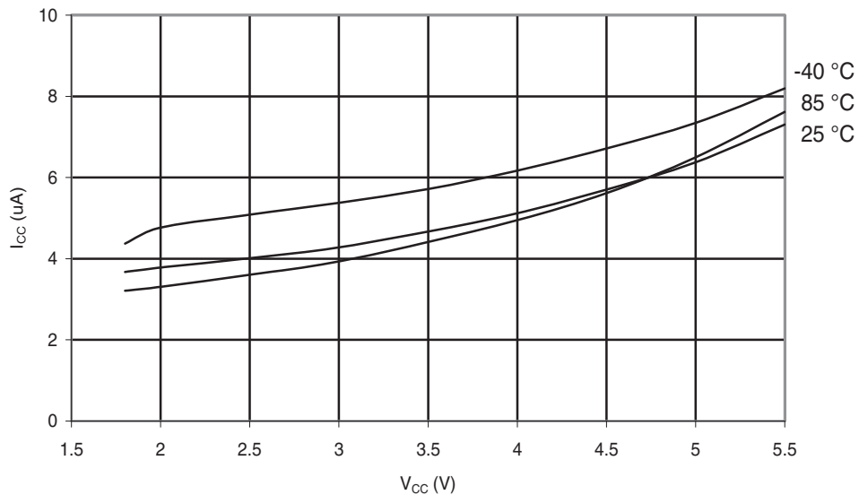
Figure 29-110. ATmega324A: Power-down Supply Current vs. V_{CC} (Watchdog Timer Enabled).
