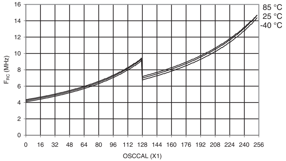
Figure 29-385. ATmega1284P: Calibrated 8MHz RC Oscillator vs. OSCCAL Value
