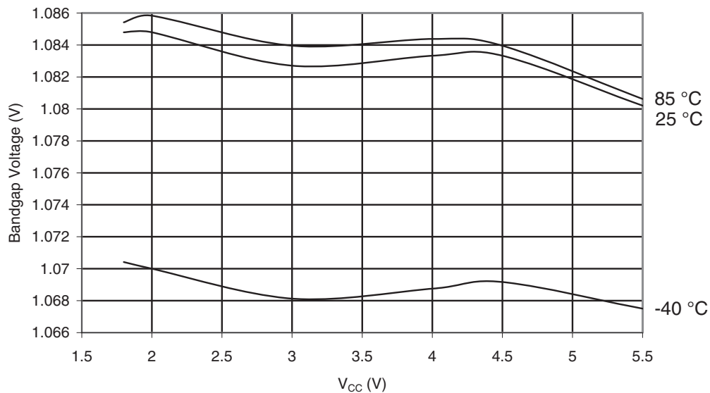
Figure 29-279. ATmega644PA: Calibrated Bandgap Voltage vs. V_{CC}
