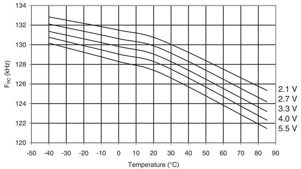
Figure 29-36. ATmega164A: Watchdog Oscillator Frequency vs. Temperature
