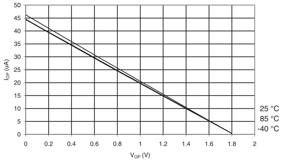
Figure 29-15. ATmega164A: I/O Pin Pull-up Resistor Current vs. Input Voltage ( V_{CC} = 1.8V ).
