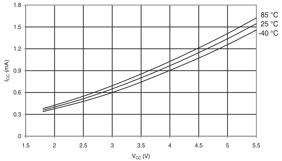
Figure 29-106. ATmega324A: Idle Supply Current vs. V_{CC} (Internal RC Oscillator, 8MHz).
