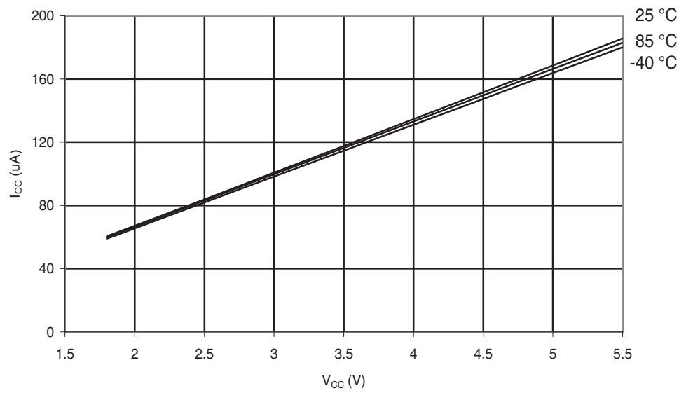
Figure 29-141. ATmega324A: AREF External Reference Current vs. V_{CC}
