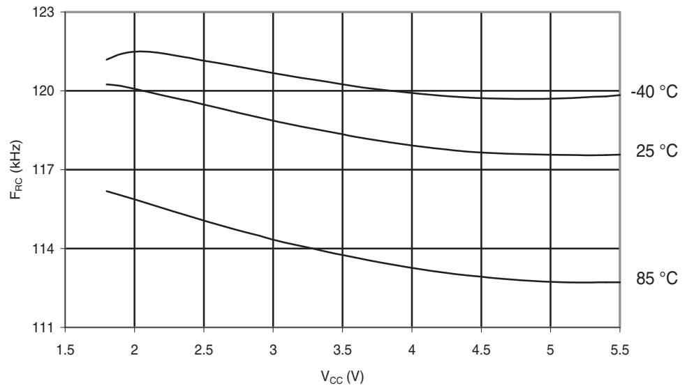
Figure 29-135. ATmega324A: Watchdog Oscillator Frequency vs. V_{CC}
