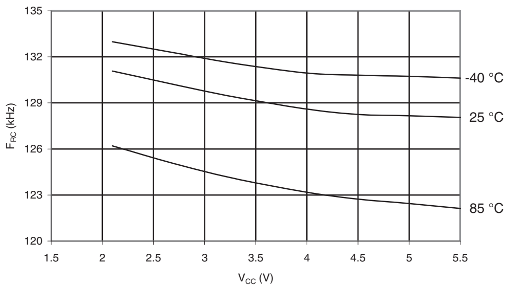
Figure 29-86. ATmega164PA: Watchdog Oscillator Frequency vs. V_{CC}
