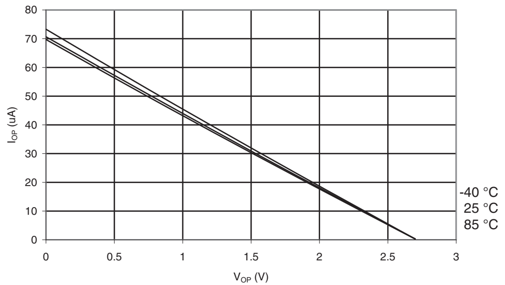
Figure 29-360. ATmega1284P: I/O Pin Pull-up Resistor Current vs. Input Voltage ( V_{CC} = 2.7V )
