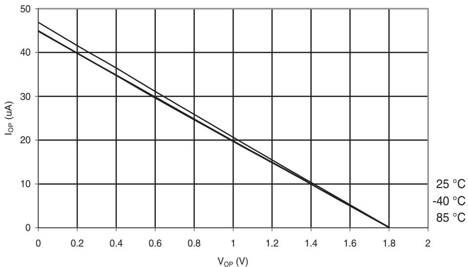
Figure 29-113. ATmega324A: I/O Pin Pull-up Resistor Current vs. Input Voltage ( V_{CC} = 1.8V ).
