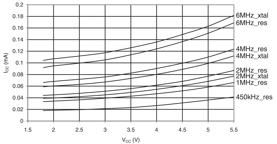
Figure 29-63. ATmega164PA: Standby Supply Current vs. V_{CC} (Watchdog Timer Disabled).
