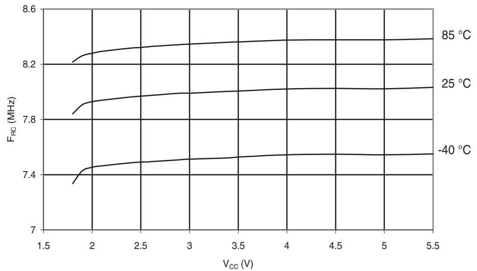
Figure 29-185. ATmega324PA: Calibrated 8MHz RC Oscillator vs. V_{CC}
