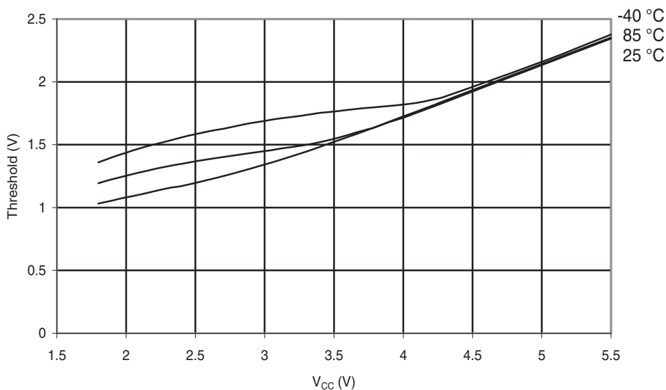
Figure 29-175. ATmega324PA: Reset Pin Input Threshold vs. V_{CC} ( V_{IH} , I/O Pin Read as '1').
