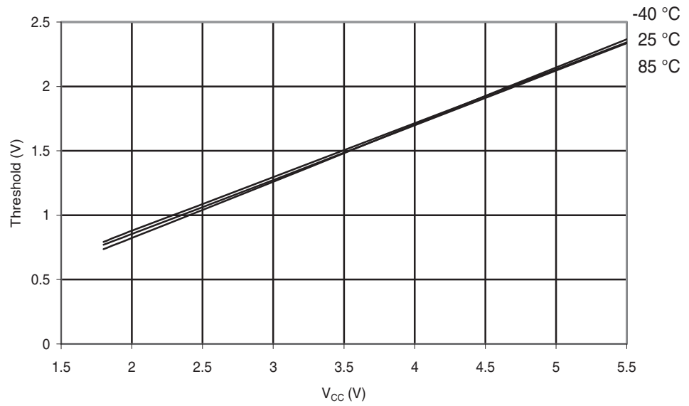
Figure 29-127. ATmega324A: Reset Pin Input Threshold vs. V_{CC} ( V_{IL} , I/O Pin Read as '0').
