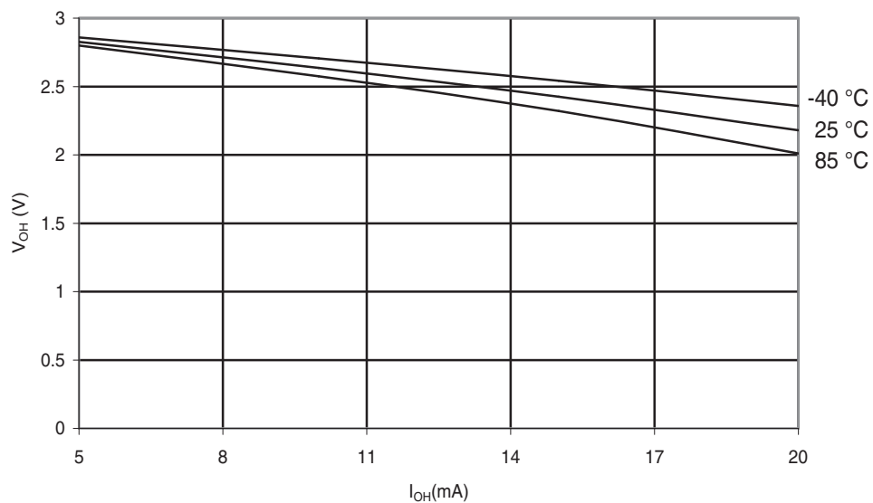
Figure 29-121. ATmega324A: I/O Pin Output Voltage vs. Source Current ( V_{CC} = 3V ).
