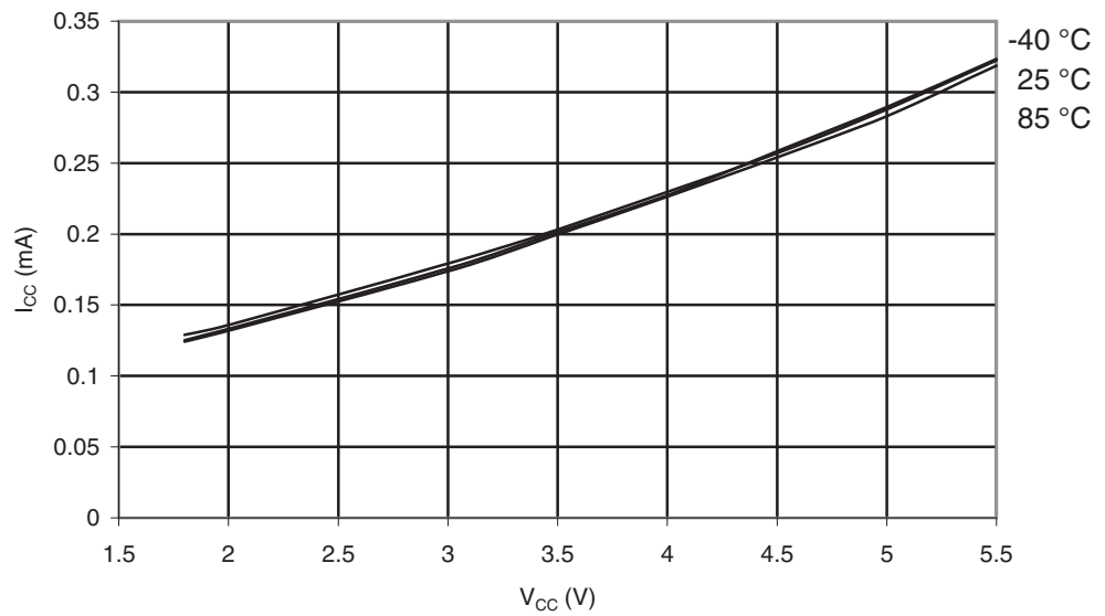
Figure 29-9. ATmega164A: Idle Supply Current vs. V_{CC} (Internal RC Oscillator, 1MHz).
