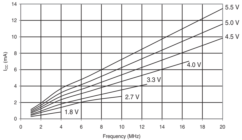
Figure 29-100. ATmega324A: Active Supply Current vs. Frequency (1 - 20MHz).
