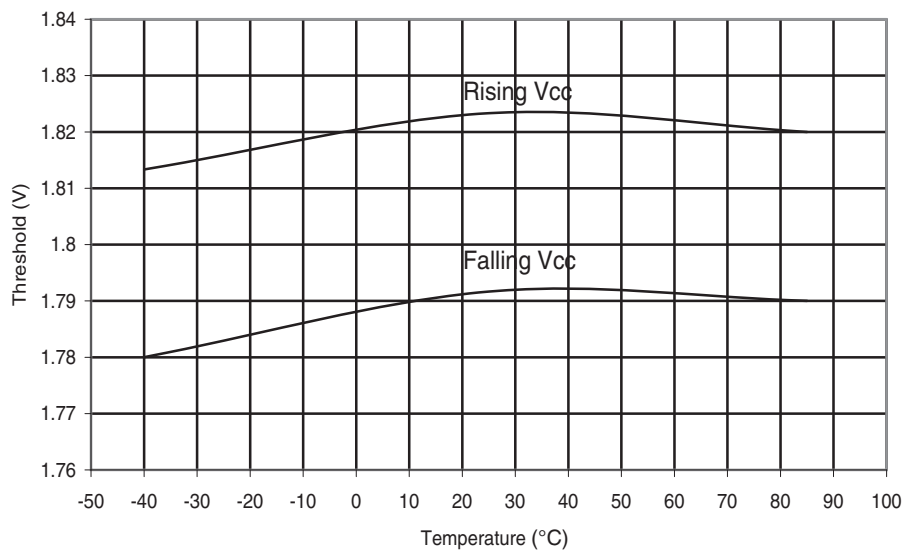
Figure 29-278. ATmega644PA: BOD Threshold vs. Temperature ( V_{BOT} = 1.8V )
