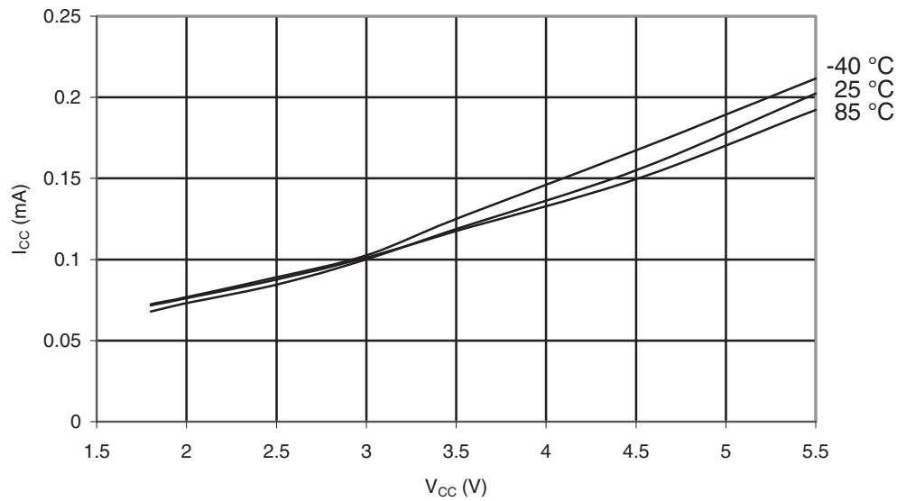
Figure 29-54. ATmega164PA: Active Supply Current vs. V_{CC} (Internal RC Oscillator, 128kHz).
