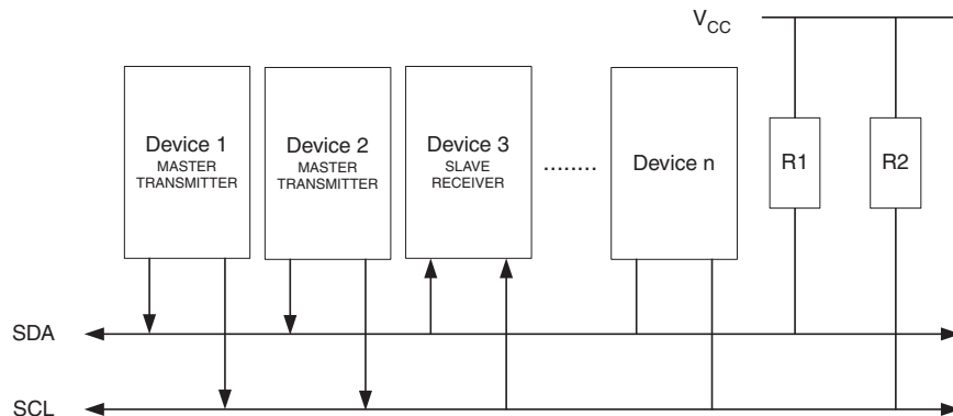
Figure 21-20. An Arbitration Example
