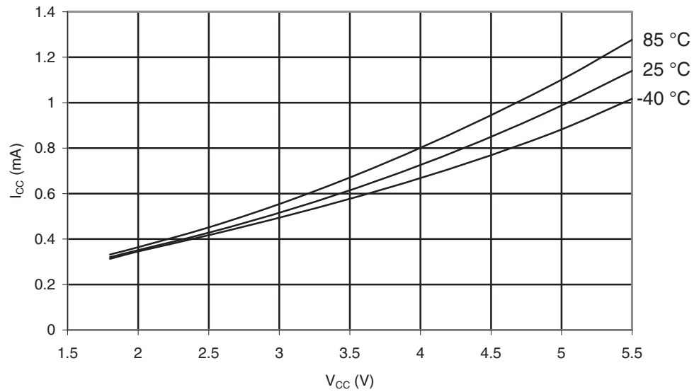
Figure 29-352. ATmega1284P: Idle Supply Current vs. V_{CC} (Internal RC Oscillator, 8MHz)
