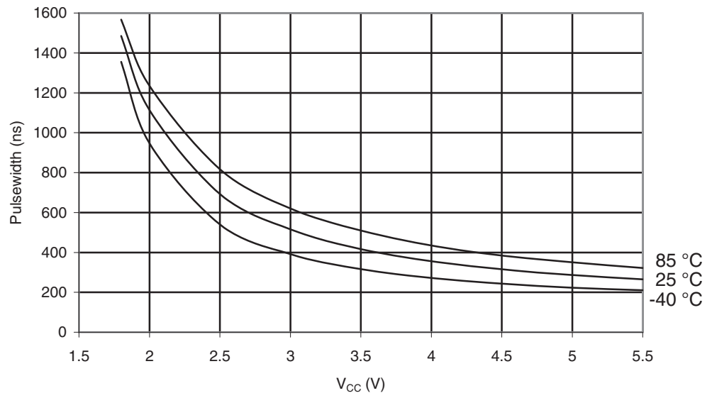
Figure 29-98. ATmega164PA: Minimum Reset Pulsewidth vs. V_{CC}
