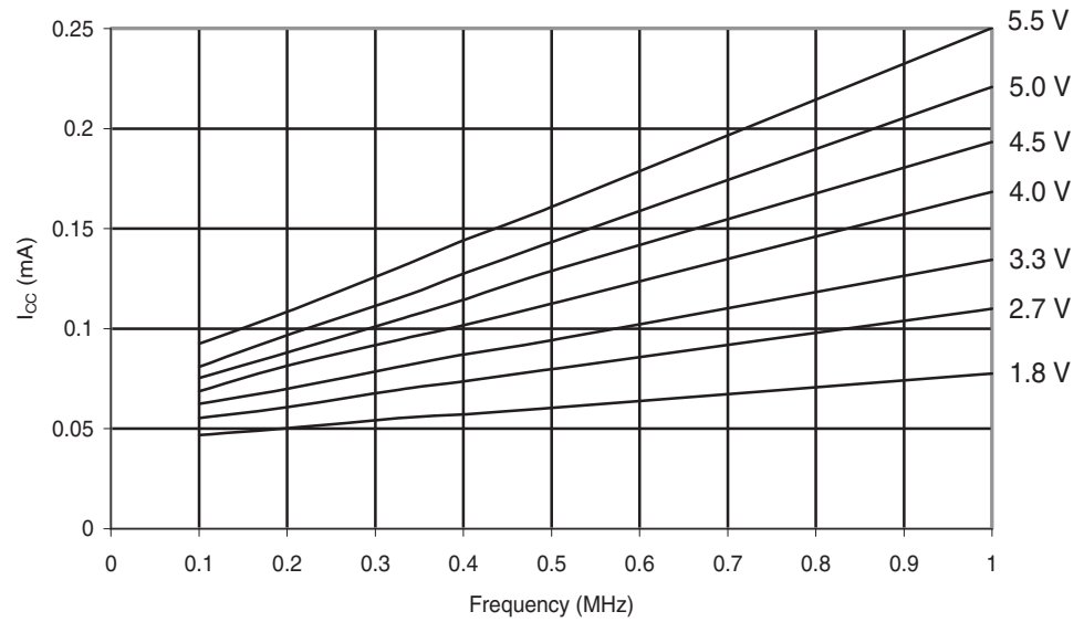
Figure 29-153. ATmega324PA: Idle Supply Current vs. V_{CC} (0.1 - 1.0MHz).
