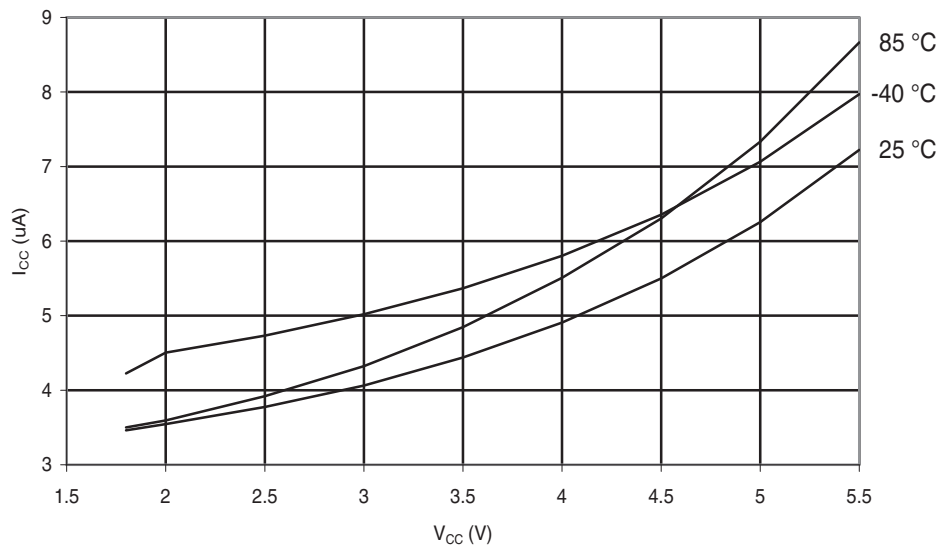
Figure 29-208. ATmega644A: Power-down Supply Current vs. V_{CC} (Watchdog Timer Enabled)
