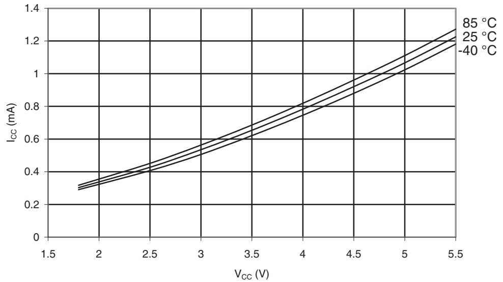
Figure 29-204. ATmega644A: Idle Supply Current vs. V_{CC} (Internal RC Oscillator, 8MHz).
