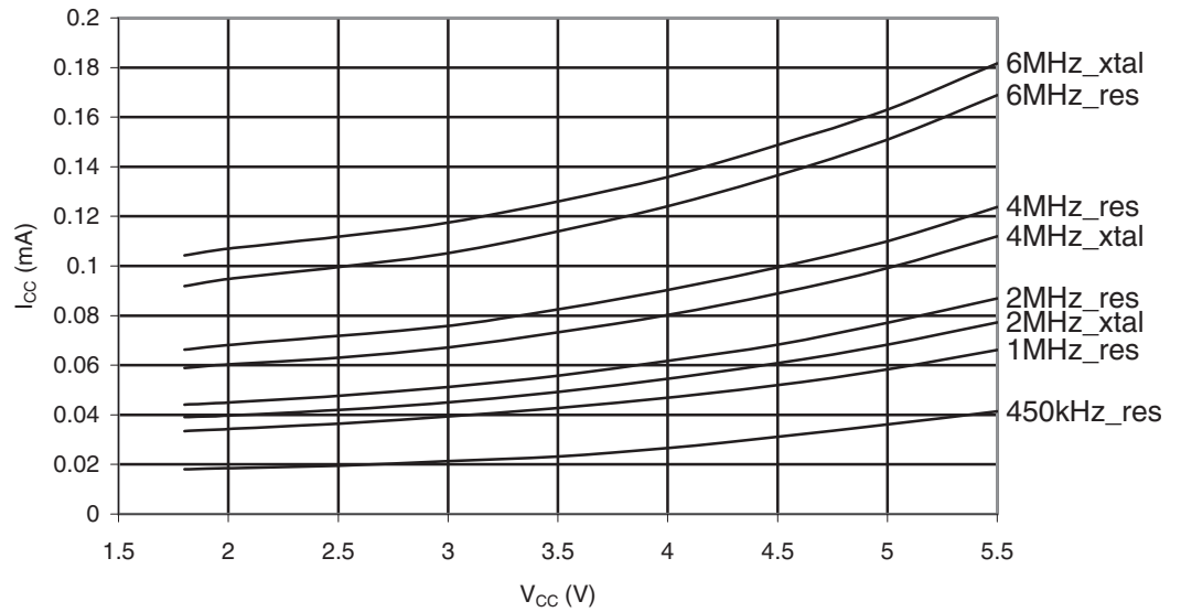
Figure 29-14. ATmega164A: Standby Supply Current vs. V_{CC} (Watchdog Timer Disabled).
