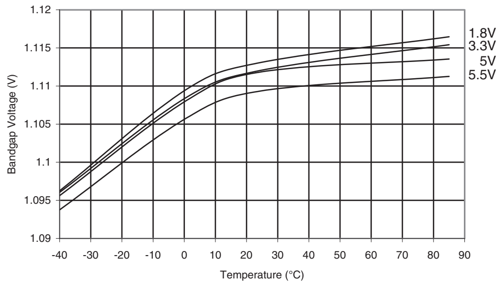
Figure 29-380. ATmega1284P: Bandgap Voltage vs. Temperature
