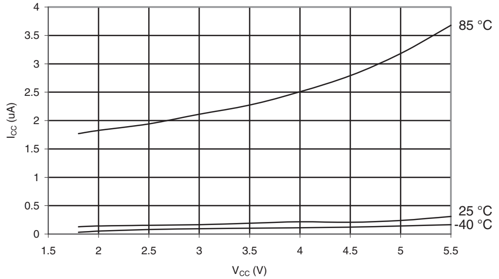
Figure 29-306. ATmega1284: Power-down Supply Current vs. V_{CC} (Watchdog Timer Enabled)
