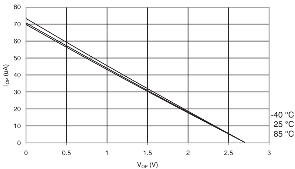
Figure 29-310. ATmega1284: I/O Pin Pull-up Resistor Current vs. Input Voltage ( V_{CC} = 2.7V )
