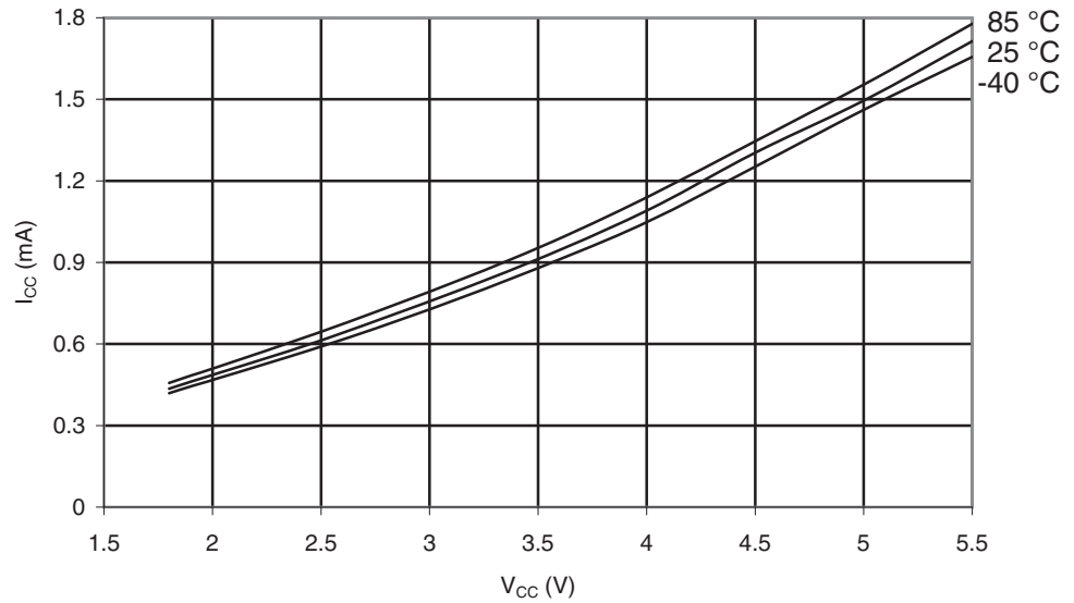
Figure 29-348. ATmega1284P: Active Supply Current vs. V_{CC} (Internal RC Oscillator, 1MHz)
