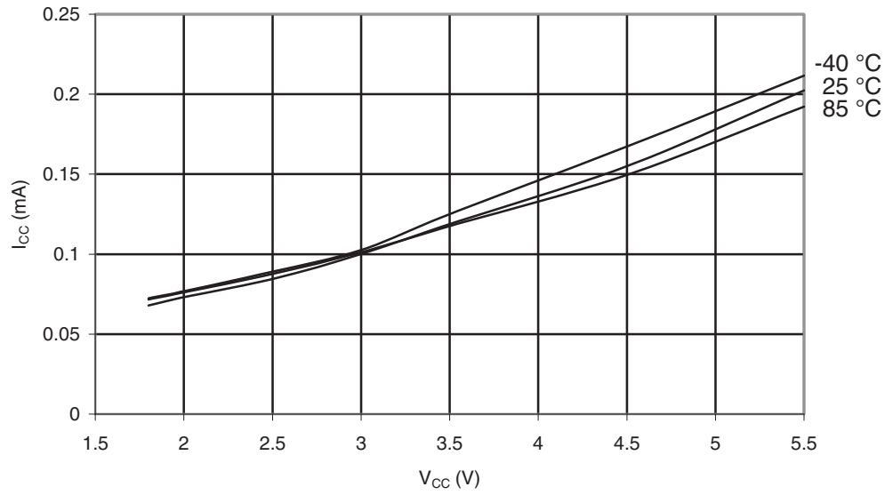
Figure 29-5. ATmega164A: Active Supply Current vs. V_{CC} (Internal RC Oscillator, 128kHz).
