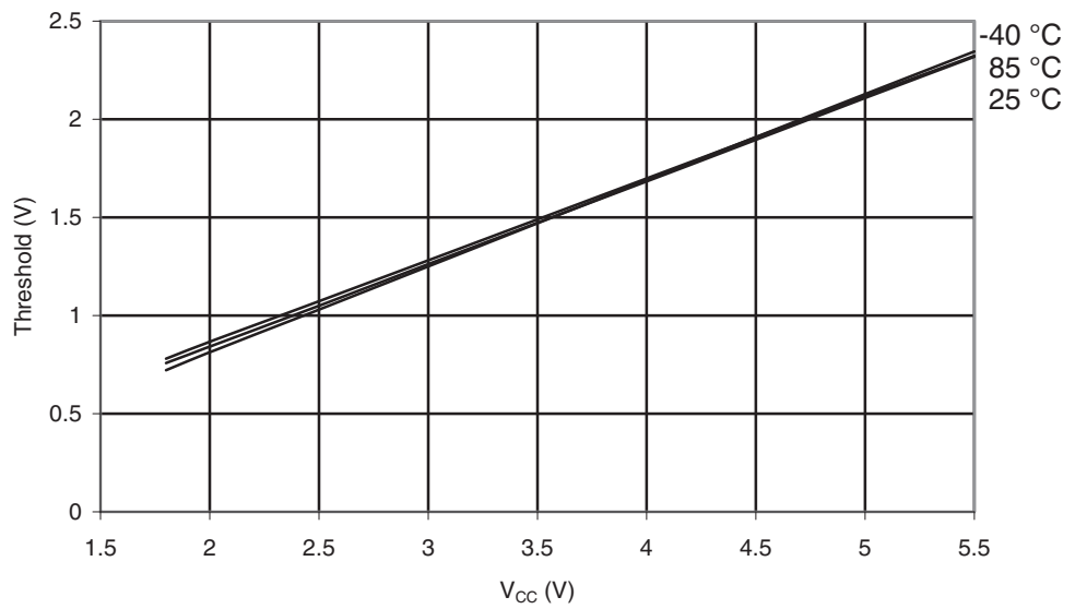
Figure 29-374. ATmega1284P: Reset Pin Input Threshold vs. V_{CC} ( V_{IL} , I/O Pin Read as '0')
