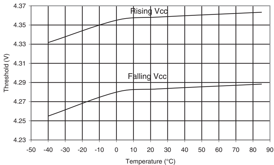
Figure 29-376. ATmega1284P: BOD Threshold vs. Temperature ( V_{BOT} = 4.3V )
