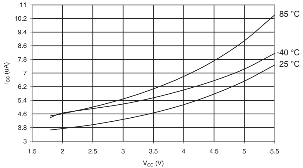
Figure 29-356. ATmega1284P: Power-down Supply Current vs. V_{CC} (Watchdog Timer Enabled)
