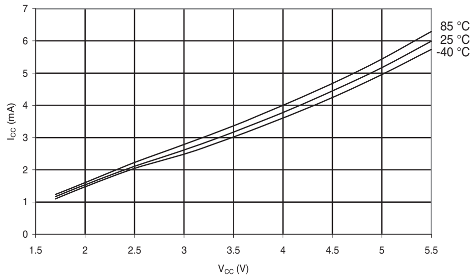
Figure 29-150. ATmega324PA: Active Supply Current vs. V_{CC} (Internal RC Oscillator, 8MHz).
