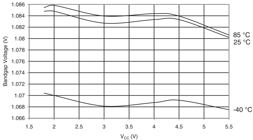
Figure 29-230. ATmega644A: Calibrated Bandgap Voltage vs. V_{CC}
