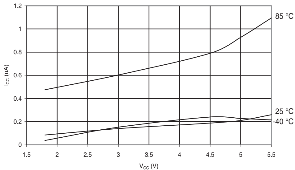
Figure 29-109. ATmega324A: Power-down Supply Current vs. V_{CC} (Watchdog Timer Disabled).
