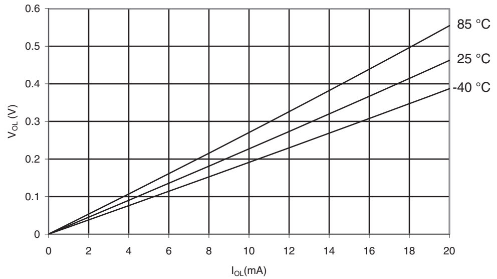
Figure 29-367. ATmega1284P: I/O Pin Output Voltage vs. Sink Current ( V_{CC} = 5V )
