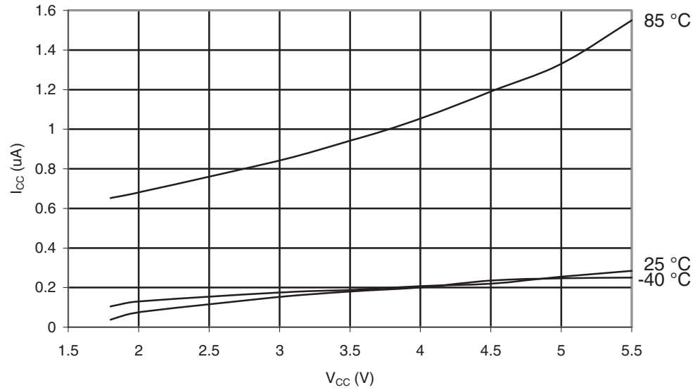
Figure 29-11. ATmega164A: Power-down Supply Current vs. V_{CC} (Watchdog Timer Disabled).
