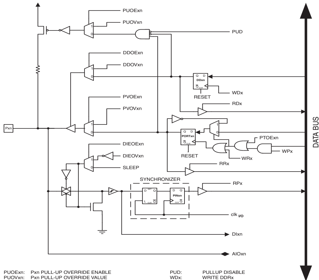
Figure 14-5. Alternate Port Functions (1)
