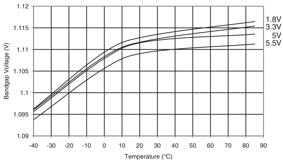
Figure 29-330. ATmega1284: Bandgap Voltage vs. Temperature
