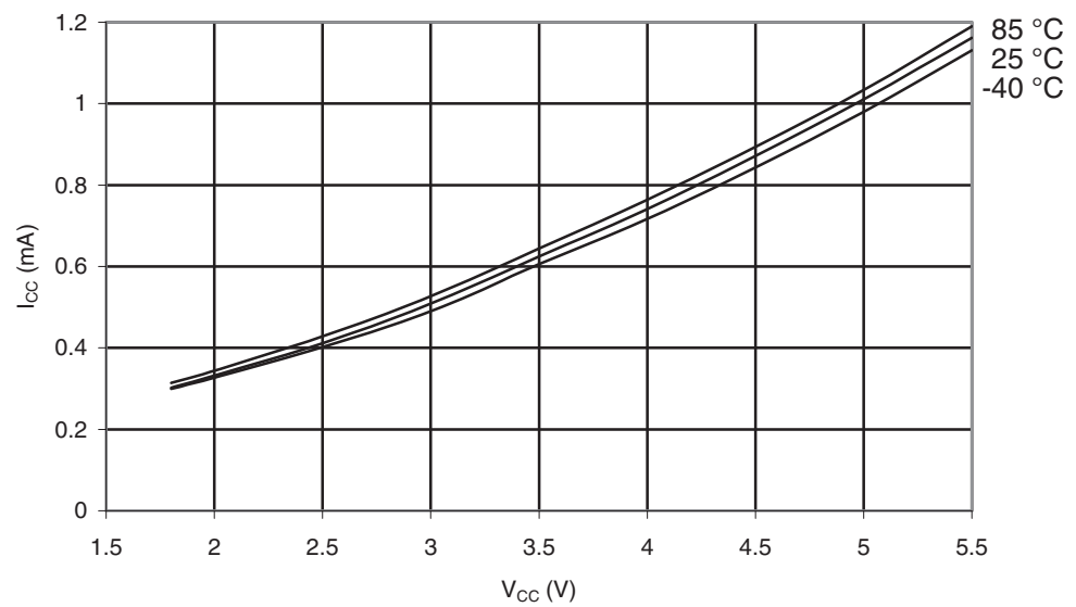
Figure 29-53. ATmega164PA: Active Supply Current vs. V_{CC} (Internal RC Oscillator, 1MHz).
