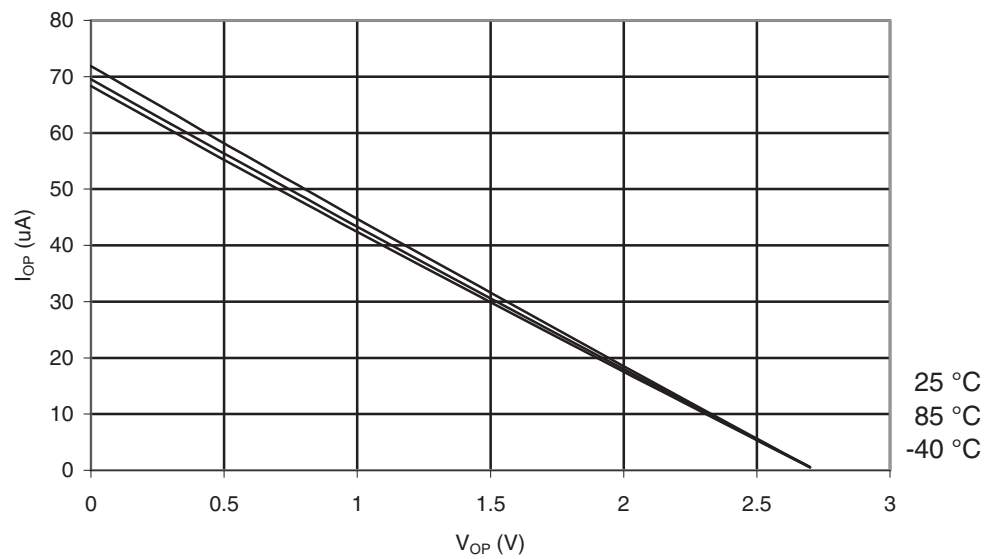
Figure 29-16. ATmega164A: I/O Pin Pull-up Resistor Current vs. Input Voltage ( V_{CC} = 2.7V ).
