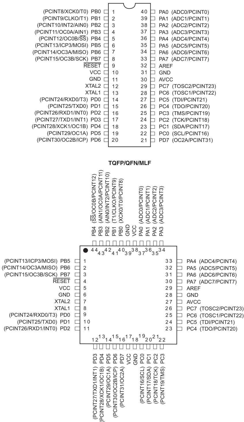
Figure 1-1. Pinout
