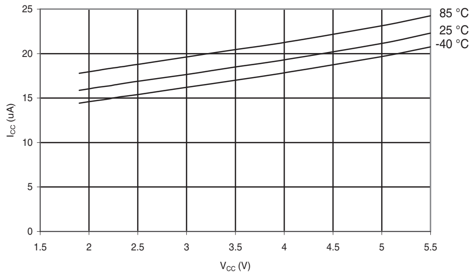
Figure 29-191. ATmega324PA: Brownout Detector Current vs. V_{CC}
