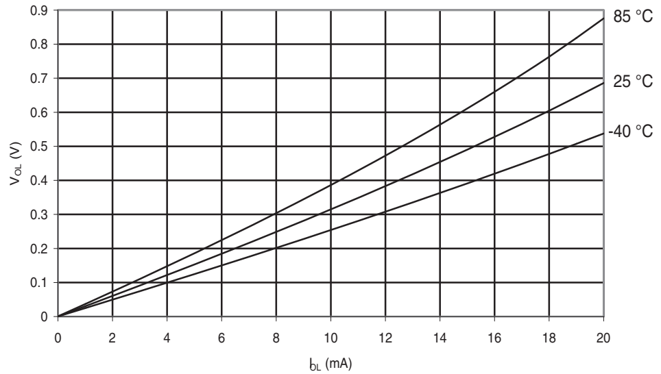
Figure 29-266. ATmega644PA: I/O Pin Output Voltage vs. Sink Current ( V_{CC} = 3V ).
