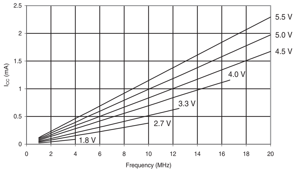
Figure 29-195. ATmega324PA: Reset Supply Current vs. Frequency (1 - 20MHz)
