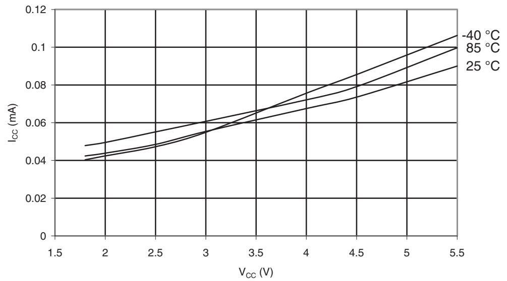
Figure 29-304. ATmega1284: Idle Supply Current vs. V_{CC} (Internal RC Oscillator, 128kHz)
