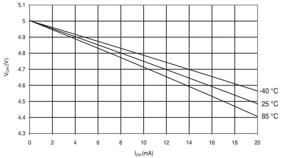
Figure 29-220. ATmega644A: I/O Pin Output Voltage vs. Source Current ( V_{CC} = 5V )
