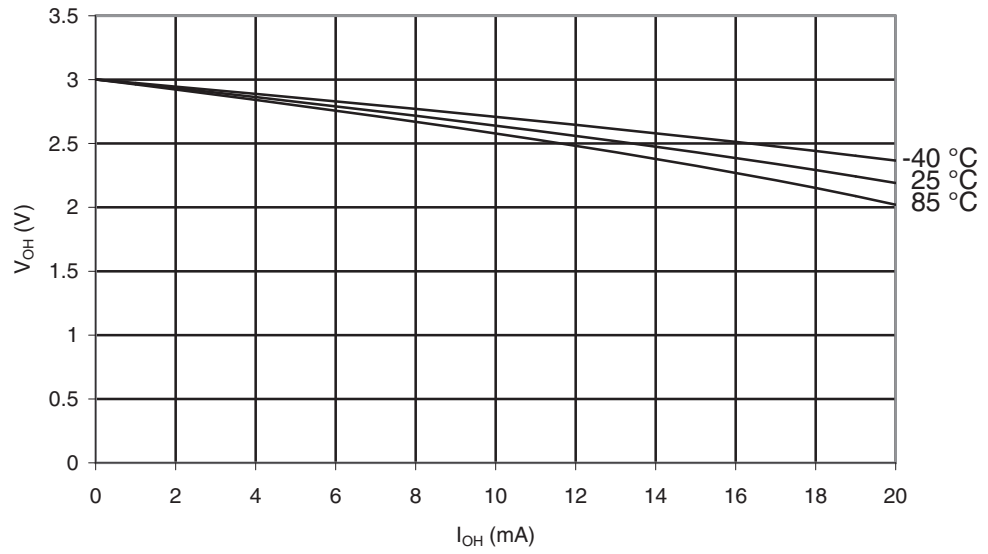
Figure 29-319. ATmega1284: I/O Pin Output Voltage vs. Source Current ( V_{CC} = 3V )
