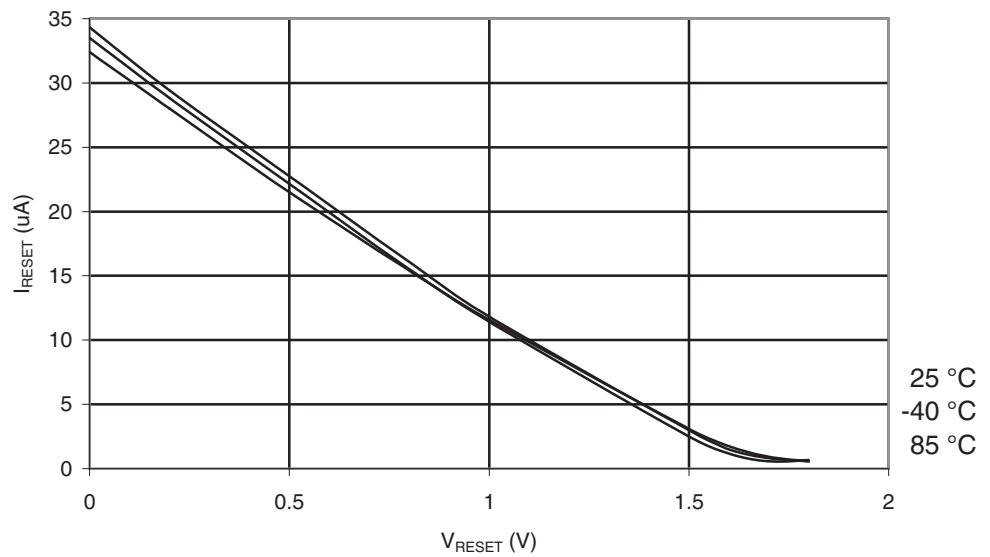
Figure 29-67. ATmega164PA: Reset Pull-up Resistor Current vs. Reset Pin Voltage ( V_{CC} = 1.8V ).
