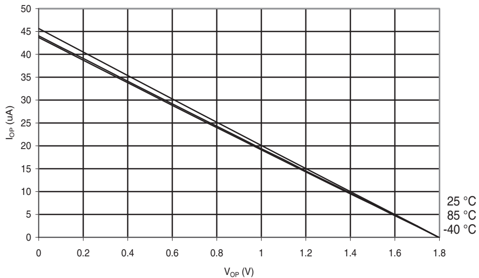
Figure 29-211. ATmega644A: I/O Pin Pull-up Resistor Current vs. Input Voltage ( V_{CC} = 1.8V )
