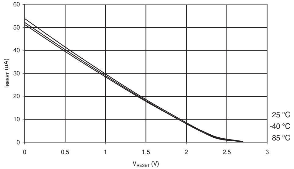
Figure 29-166. ATmega324PA: Reset Pull-up Resistor Current vs. Reset Pin Voltage ( V_{CC} = 2.7V ).
