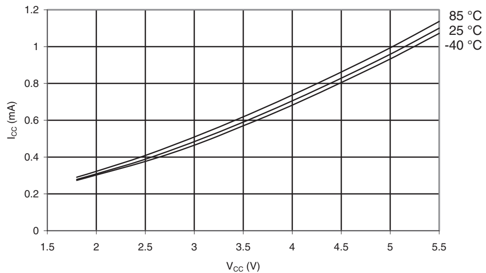
Figure 29-57. ATmega164PA: Idle Supply Current vs. V_{CC} (Internal RC Oscillator, 8MHz).
