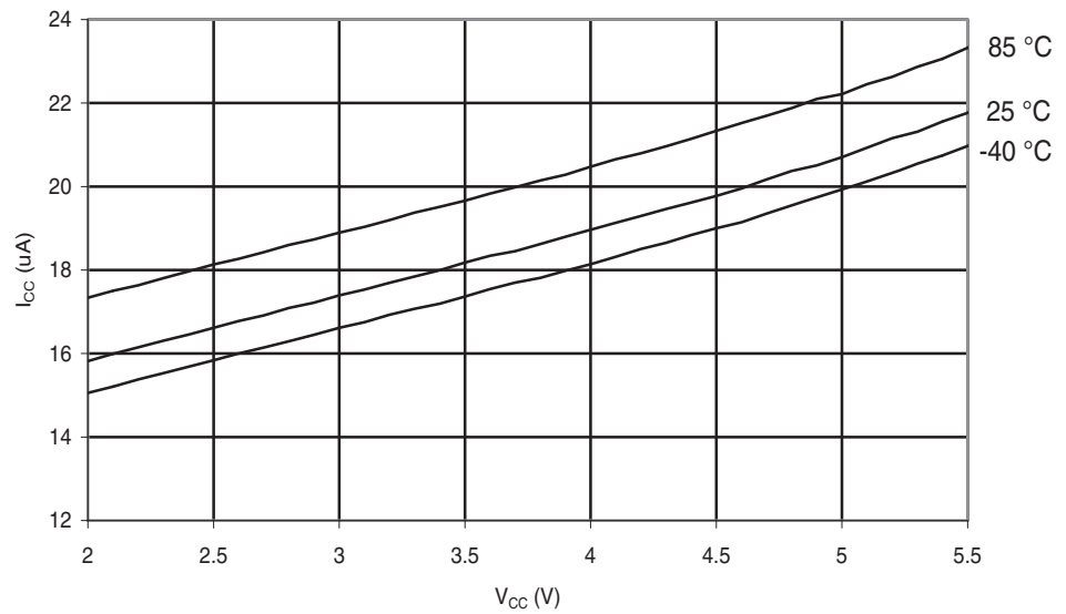
Figure 29-289. ATmega644PA: Brownout Detector Current vs. V_{CC}
