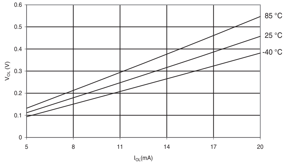
Figure 29-120. ATmega324A: I/O Pin Output Voltage vs. Sink Current ( V_{CC} = 5V ).
