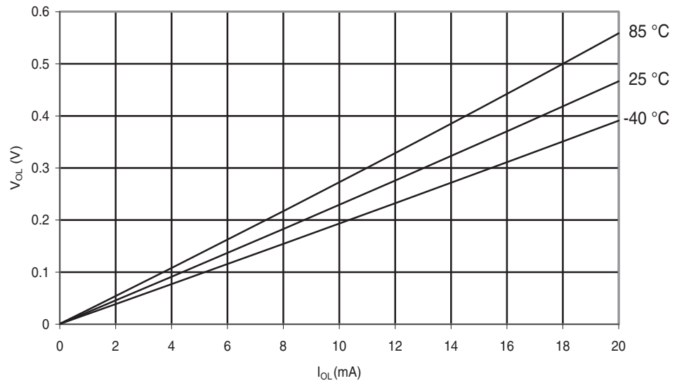
Figure 29-267. ATmega644PA: I/O Pin Output Voltage vs. Sink Current ( V_{CC} = 5V ).
