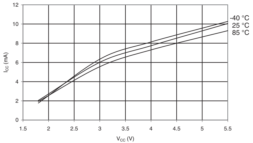
Figure 29-94. ATmega164PA: Programming Current vs. V_{CC}
