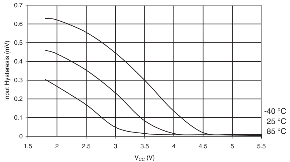
Figure 29-30. ATmega164A: Reset Pin Input Hysteresis vs. V_{CC}
