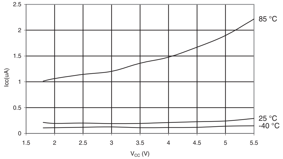
Figure 29-258. ATmega644PA: Power-save Supply Current vs. V_{CC} (Watchdog Timer Disabled and 32kHz Crystal Oscillator Running).
