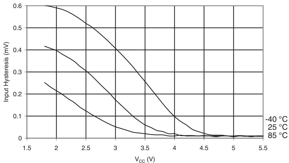
Figure 29-375. ATmega1284P: Reset Pin Input Hysteresis vs. V_{CC}
