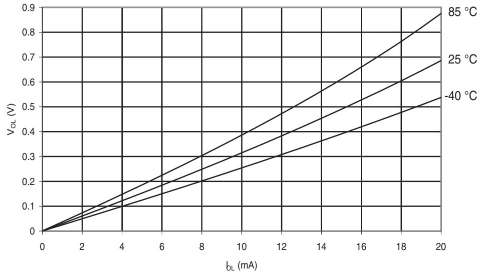
Figure 29-217. ATmega644A: I/O Pin Output Voltage vs. Sink Current ( V_{CC} = 3V ).
