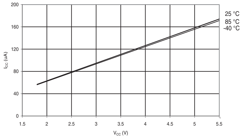
Figure 29-288. ATmega644PA: AREF External Reference Current vs. V_{CC}
