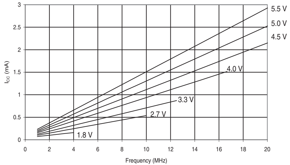
Figure 29-203. ATmega644A: Idle Supply Current vs. V_{CC} (1 - 20MHz).
