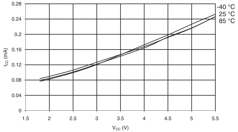
Figure 29-299. ATmega1284: Active Supply Current vs. V_{CC} (Internal RC Oscillator, 128kHz)
