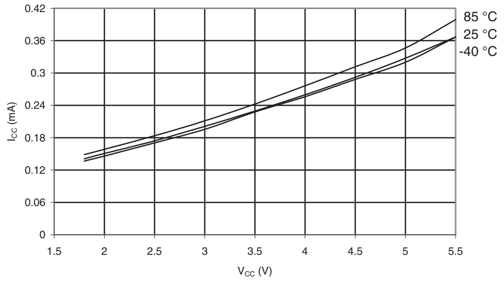
Figure 29-353. ATmega1284P: Idle Supply Current vs. V_{CC} (Internal RC Oscillator, 1MHz)
