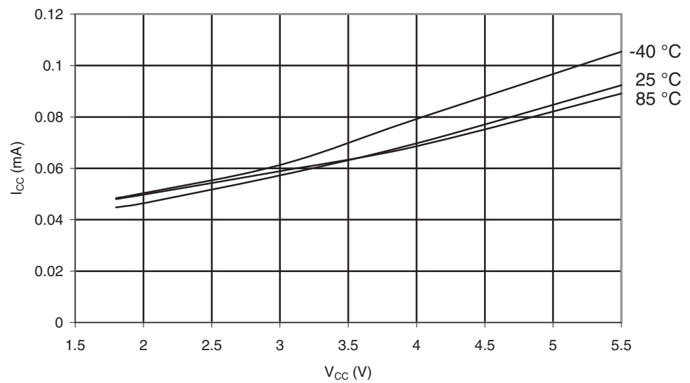
Figure 29-10. ATmega164A: Idle Supply Current vs. V_{CC} (Internal RC Oscillator, 128kHz).
