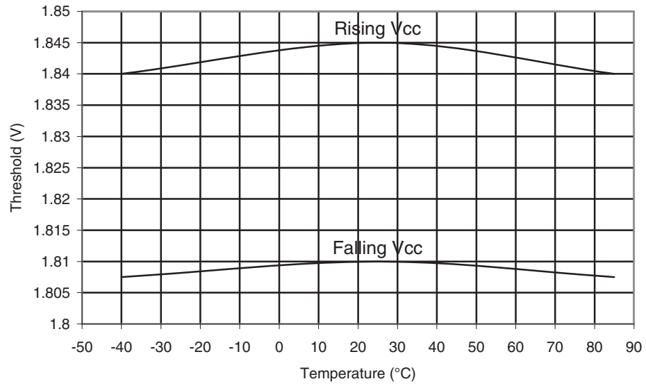
Figure 29-33. ATmega164A: BOD Threshold vs. Temperature ( V_{BOT} = 1.8V )
