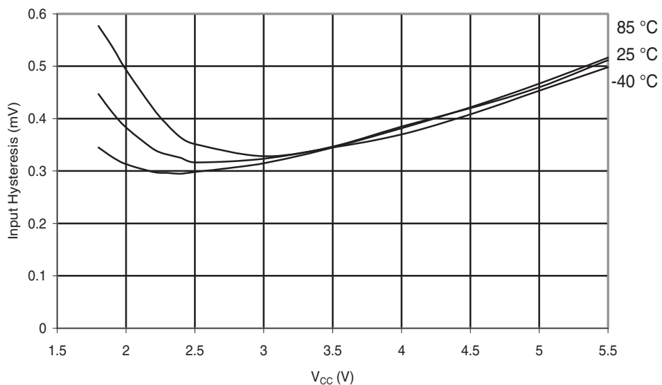
Figure 29-125. ATmega324A: I/O Pin Input Hysteresis vs. V_{CC}
