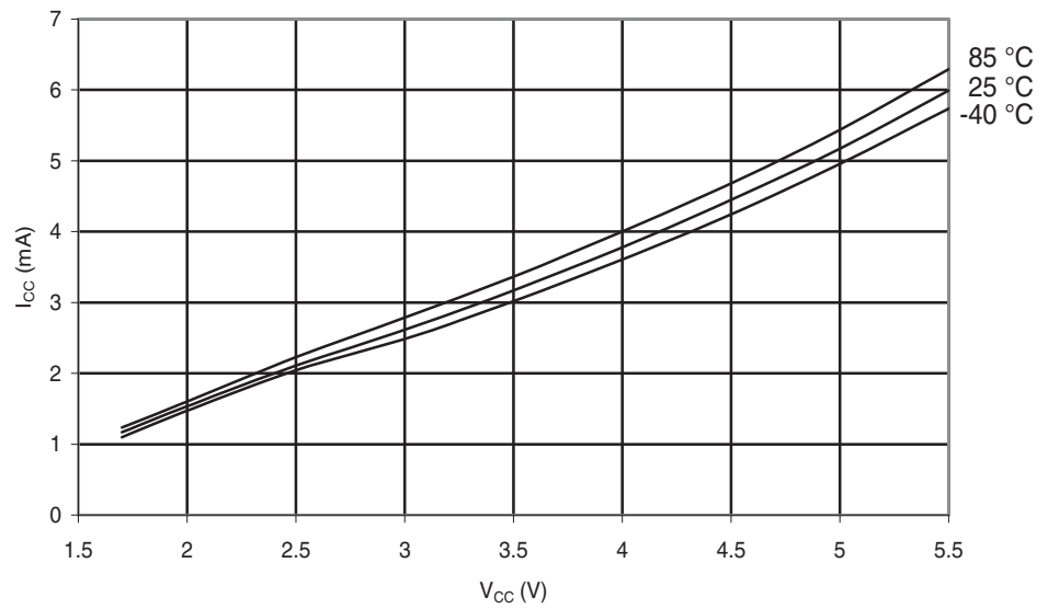
Figure 29-101. ATmega324A: Active Supply Current vs. V_{CC} (Internal RC Oscillator, 8MHz).
