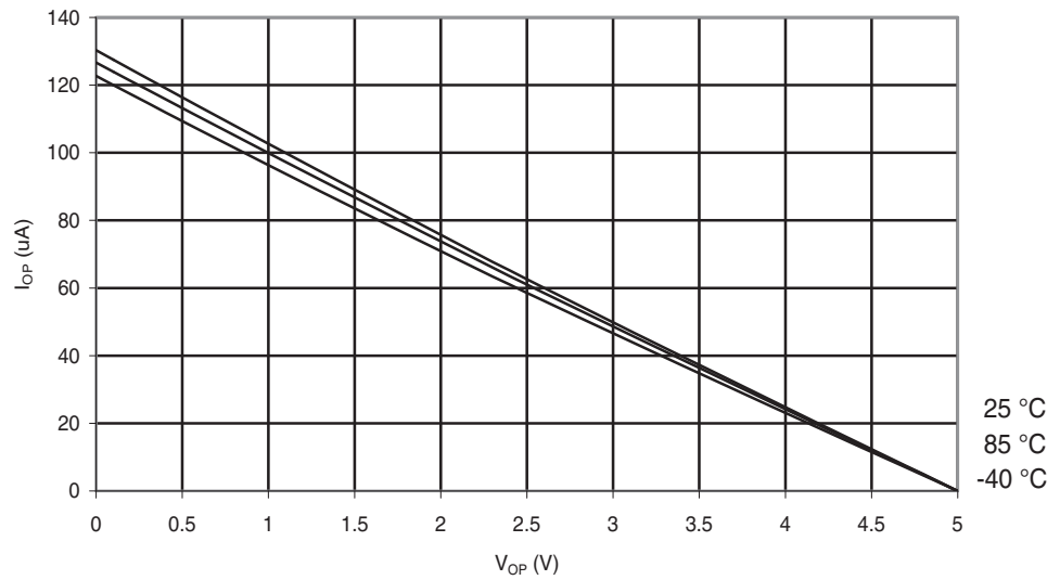
Figure 29-262. ATmega644PA: I/O Pin Pull-up Resistor Current vs. Input Voltage ( V_{CC} = 5V ).
