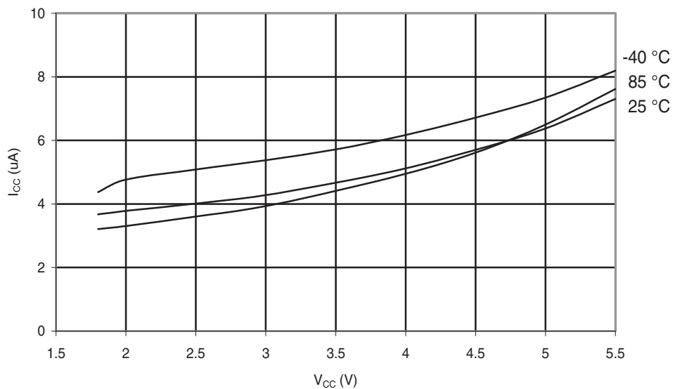
Figure 29-159. ATmega324PA: Power-down Supply Current vs. V_{CC} (Watchdog Timer Enabled).
