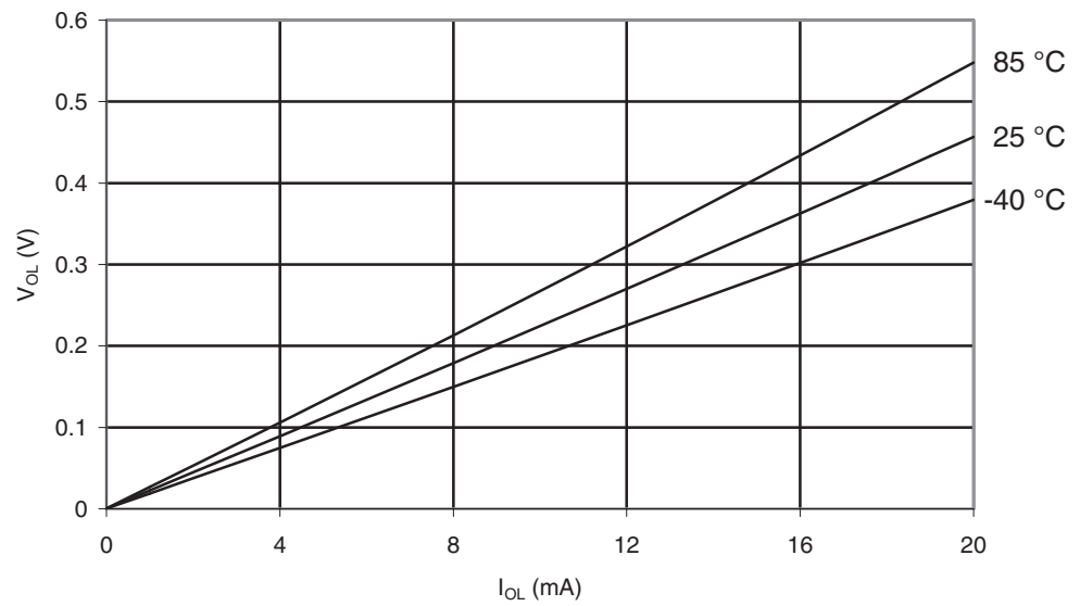
Figure 29-71. ATmega164PA: I/O Pin Output Voltage vs. Sink Current ( V_{CC} = 5V ).
