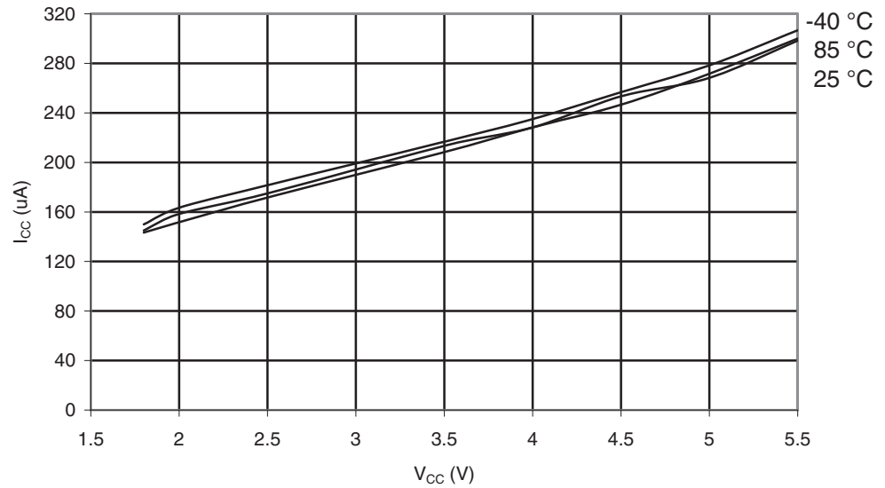
Figure 29-41. ATmega164A: ADC Current vs. V_{CC} (AREF = AV_{CC} )
