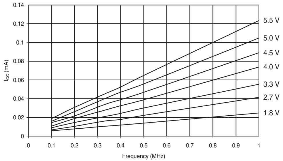
Figure 29-145. ATmega324A: Reset Supply Current vs. Low Frequency (0.1 - 1.0MHz)
