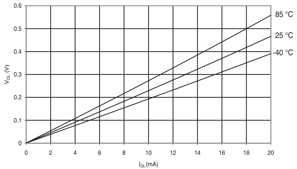
Figure 29-218. ATmega644A: I/O Pin Output Voltage vs. Sink Current ( V_{CC} = 5V ).
