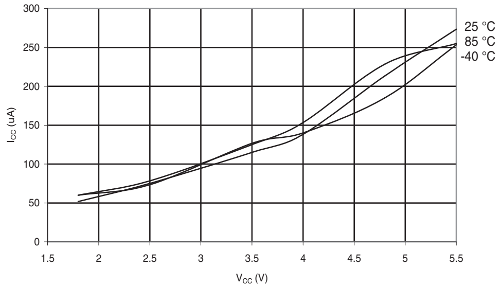
Figure 29-188. ATmega324PA: ADC Current vs. V_{CC} (AREF = AV_{CC} )
