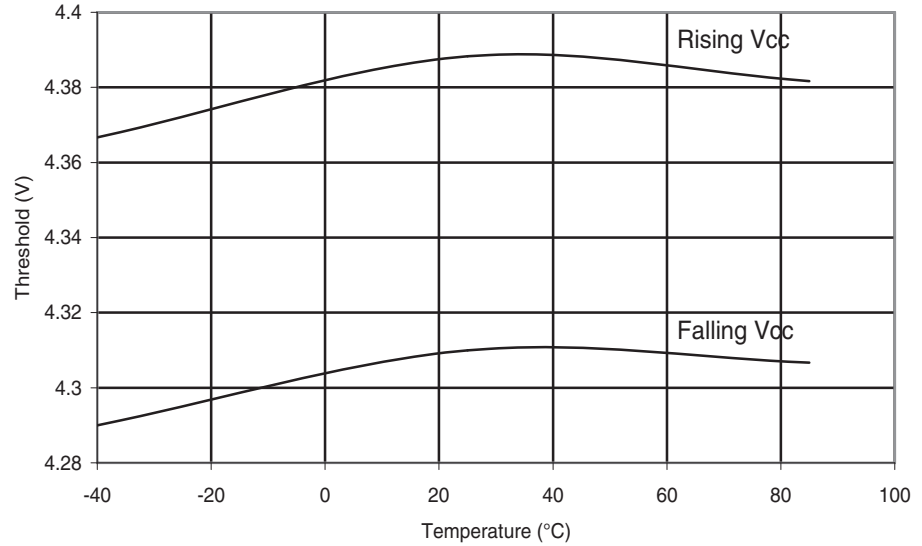
Figure 29-178. ATmega324PA: BOD Threshold vs. Temperature ( V_{BOT} = 4.3V )
