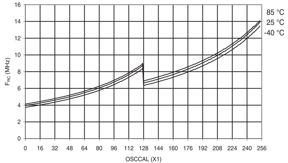
Figure 29-187. ATmega324PA: Calibrated 8MHz RC Oscillator vs. OSCCAL Value
