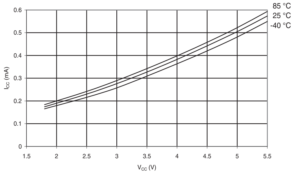
Figure 29-107. ATmega324A: Idle Supply Current vs. V_{CC} (Internal RC Oscillator, 1MHz).
