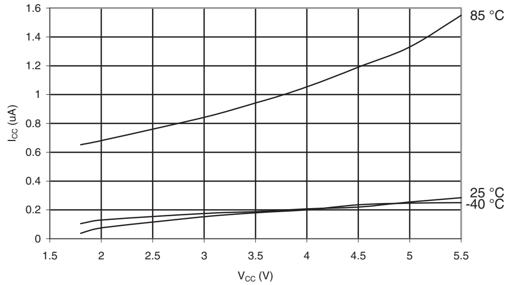
Figure 29-60. ATmega164PA: Power-down Supply Current vs. V_{CC} (Watchdog Timer Disabled).
