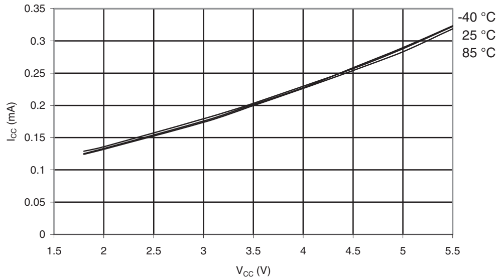
Figure 29-58. ATmega164PA: Idle Supply Current vs. V_{CC} (Internal RC Oscillator, 1MHz).
