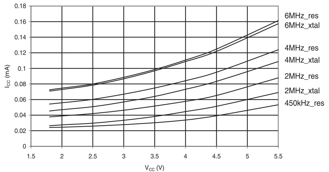
Figure 29-161. ATmega324PA: Standby Supply Current vs. V_{CC} (Watchdog Timer Disabled).
