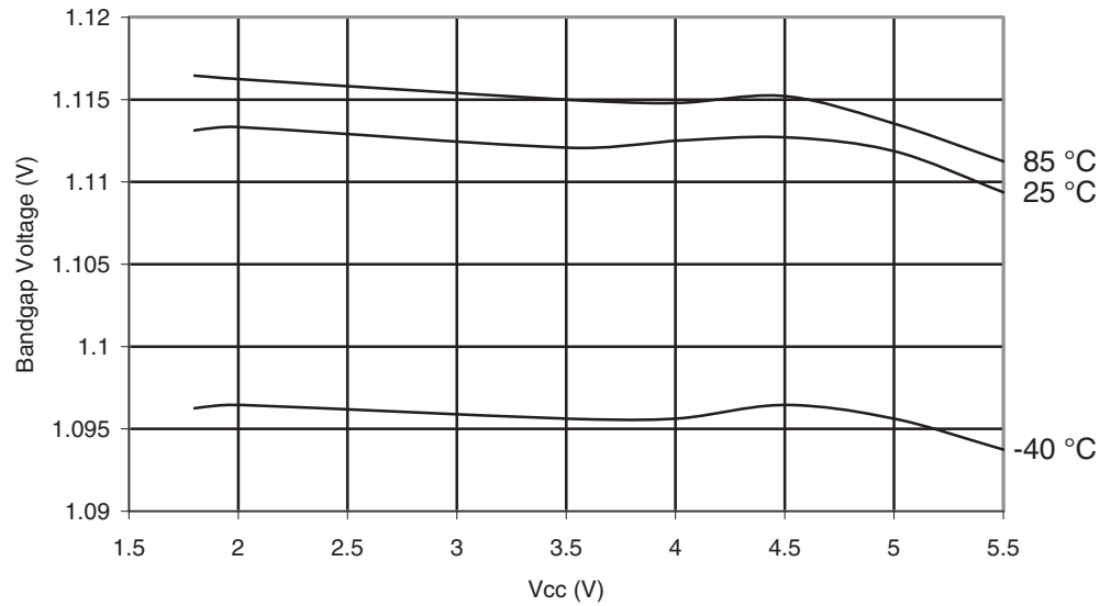
Figure 29-379. ATmega1284P: Calibrated Bandgap Voltage vs. V_{CC}
