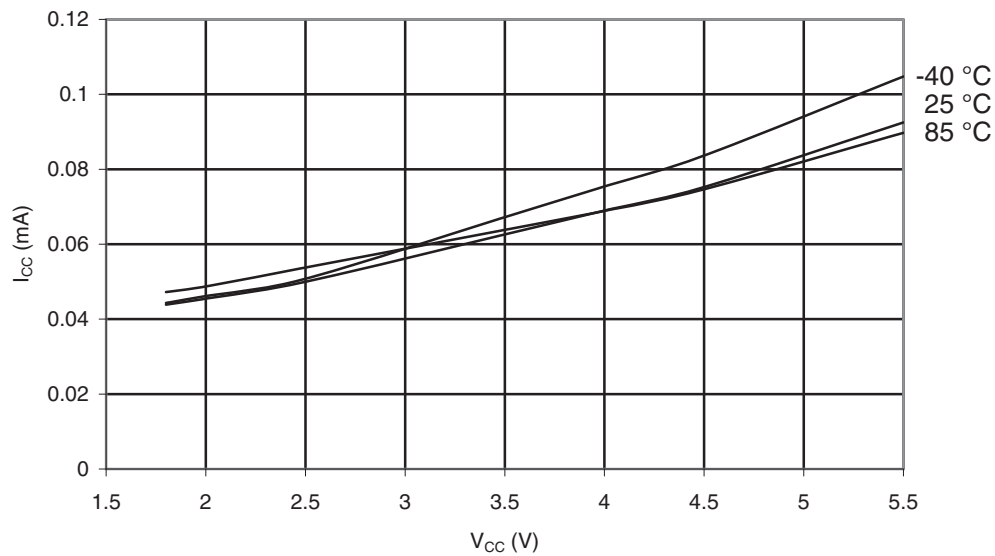
Figure 29-255. ATmega644PA: Idle Supply Current vs. V_{CC} (Internal RC Oscillator, 128kHz).
