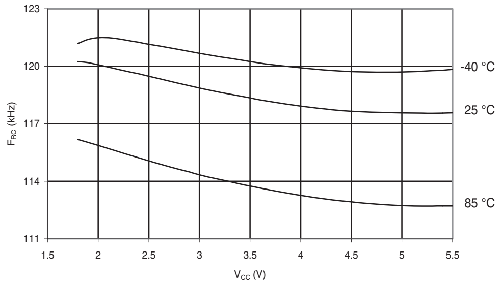
Figure 29-184. ATmega324PA: Watchdog Oscillator Frequency vs. V_{CC}
