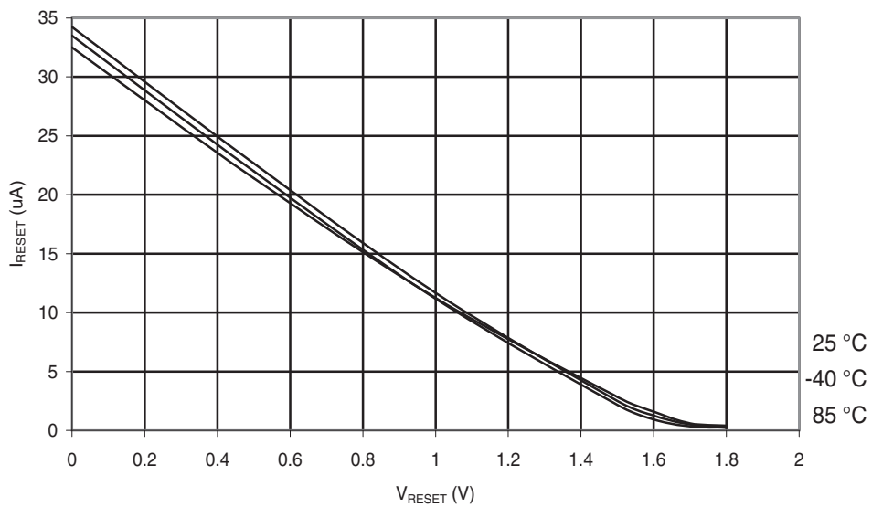
Figure 29-165. ATmega324PA: Reset Pull-up Resistor Current vs. Reset Pin Voltage ( V_{CC} = 1.8V ).
