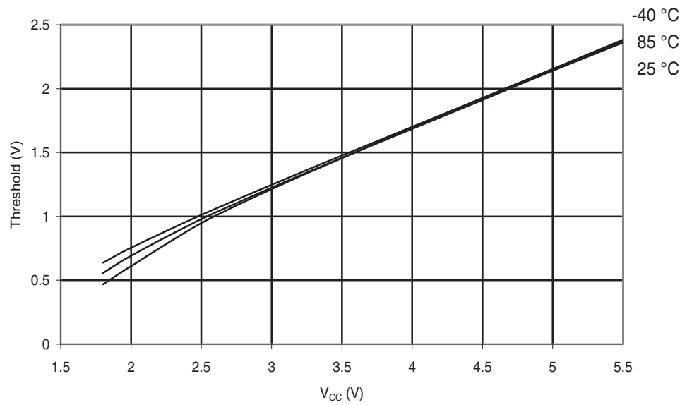
Figure 29-124. ATmega324A: I/O Pin Input Threshold vs. V_{CC} ( V_{IL} , I/O Pin Read as '0').
