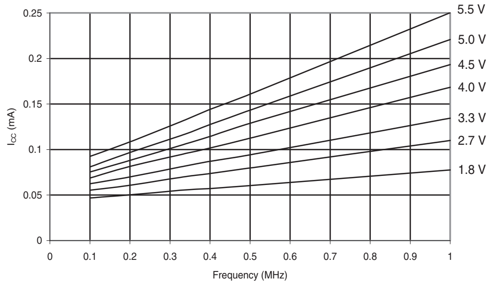
Figure 29-104. ATmega324A: Idle Supply Current vs. V_{CC} (0.1 - 1.0MHz).
