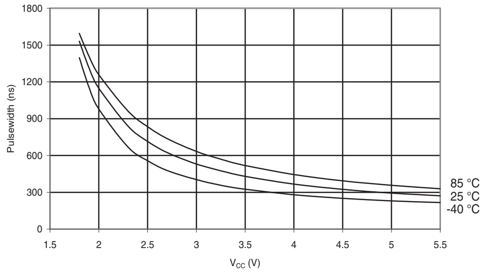
Figure 29-147. ATmega324A: Minimum Reset Pulsewidth vs. V_{CC}
