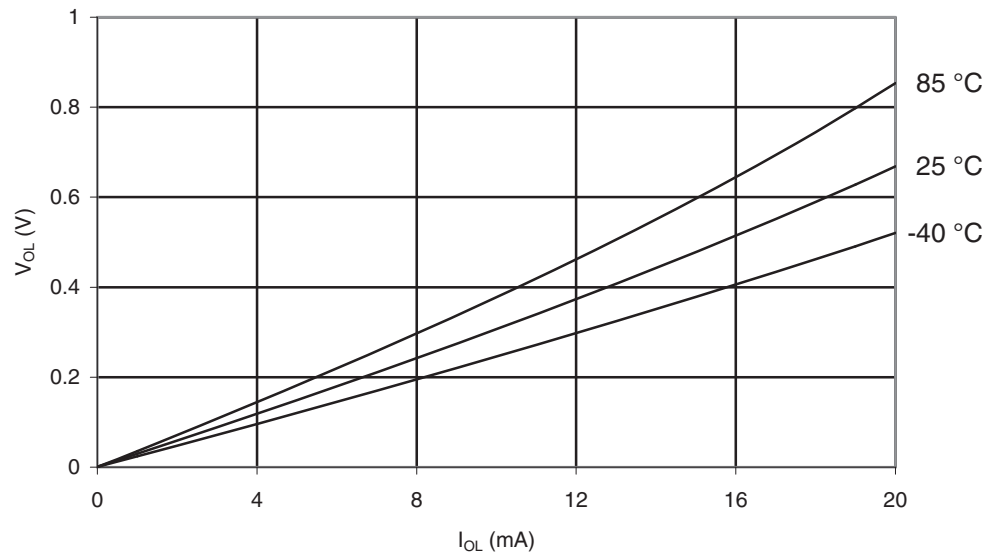
Figure 29-21. ATmega164A: I/O Pin Output Voltage vs. Sink Current ( V_{CC} = 3V ).
