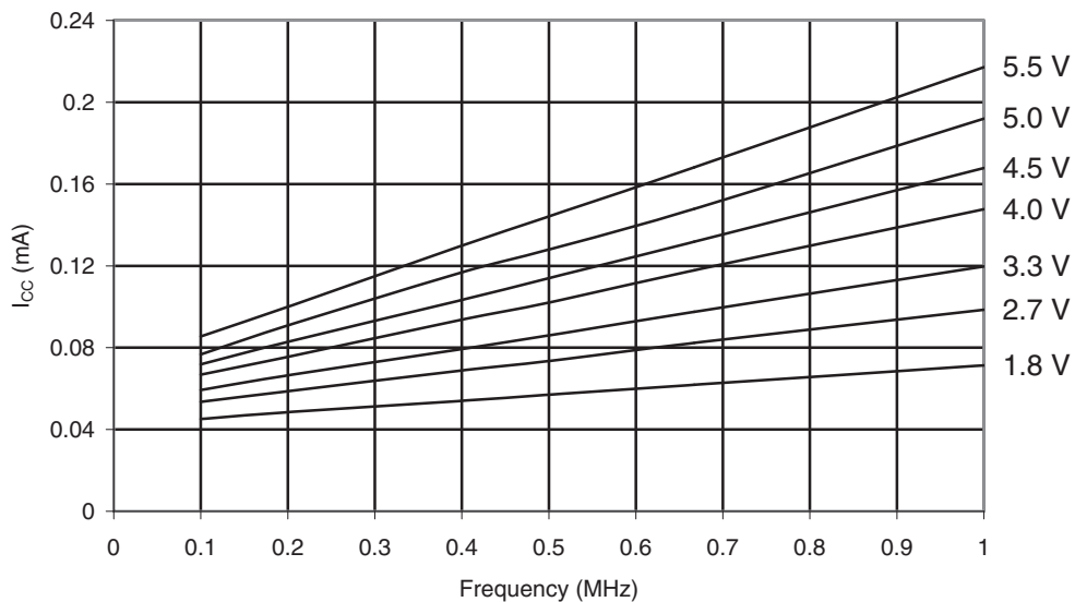
Figure 29-202. ATmega644A: Idle Supply Current vs. V_{CC} (0.1 - 1.0MHz).
