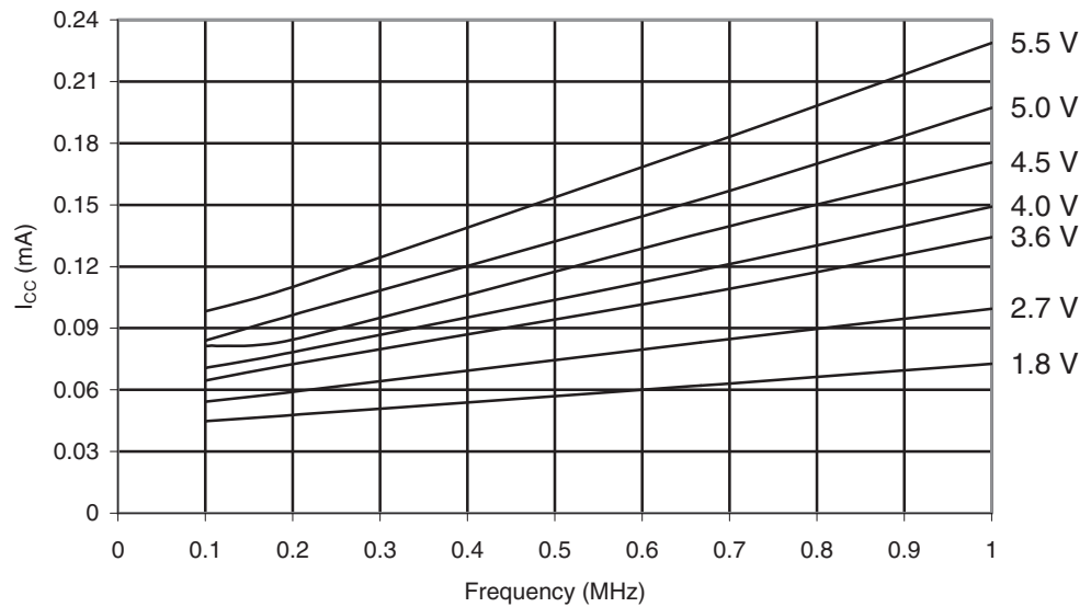
Figure 29-350. ATmega1284P: Idle Supply Current vs. Low Frequency (0.1 - 1.0MHz)
