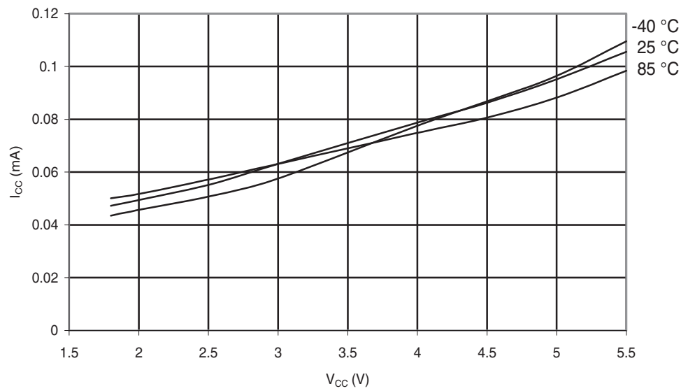
Figure 29-108. ATmega324A: Idle Supply Current vs. V_{CC} (Internal RC Oscillator, 128kHz).
