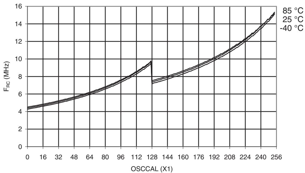
Figure 29-40. ATmega164A: Calibrated 8MHz RC Oscillator vs. OSCCAL Value
