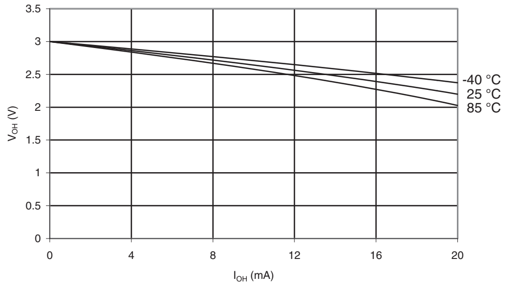
Figure 29-23. ATmega164A: I/O Pin Output Voltage vs. Source Current ( V_{CC} = 3V ).
