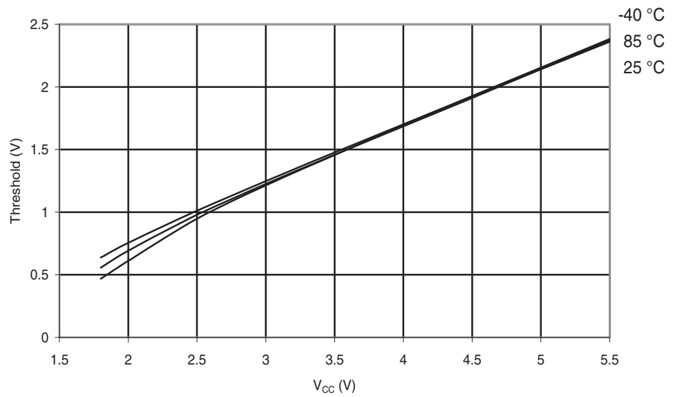
Figure 29-173. ATmega324PA: I/O Pin Input Threshold vs. V_{CC} ( V_{IL} , I/O Pin Read as '0').
