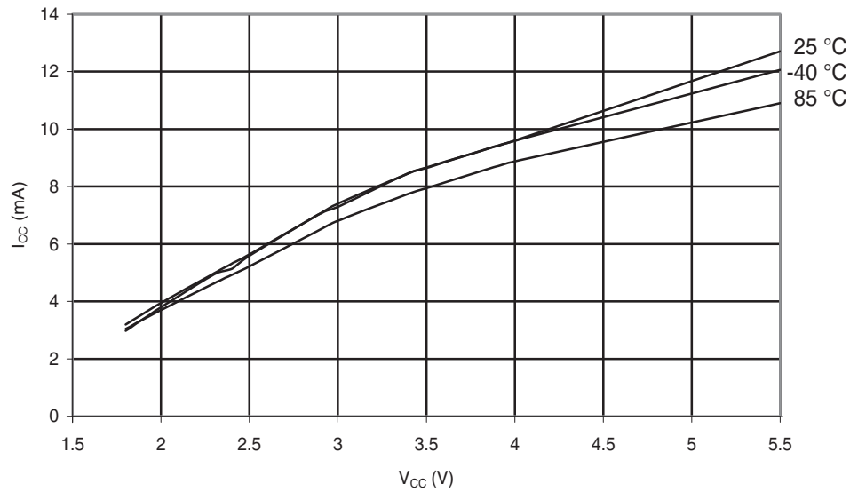
Figure 29-192. ATmega324PA: Programming Current vs. V_{CC}
