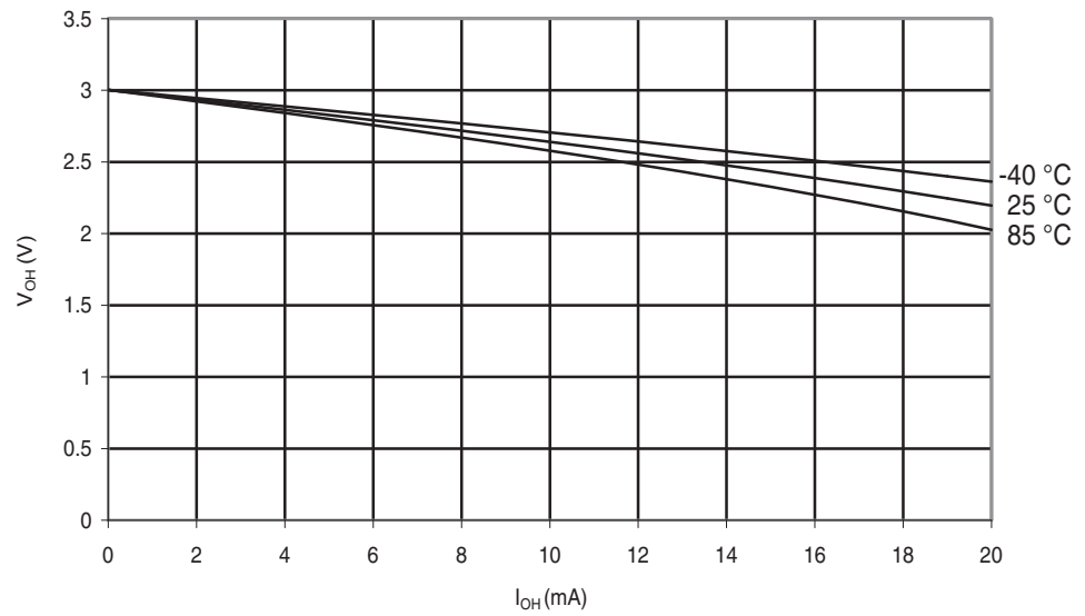
Figure 29-268. ATmega644PA: I/O Pin Output Voltage vs. Source Current ( V_{CC} = 3V ).
