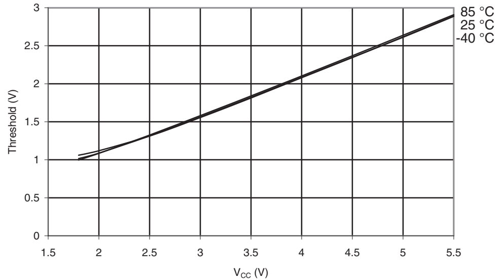
Figure 29-320. ATmega1284: I/O Pin Input Threshold vs. V_{CC} ( V_{IH} , I/O Pin Read as '1')
