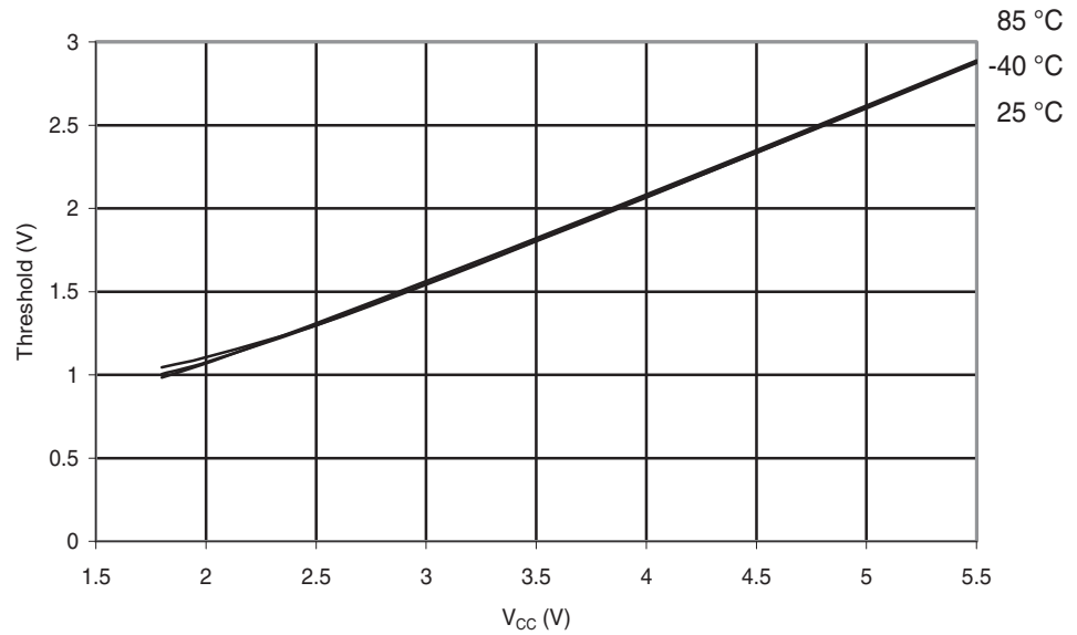
Figure 29-123. ATmega324A: I/O Pin Input Threshold vs. V_{CC} ( V_{IH} , I/O Pin Read as '1').
