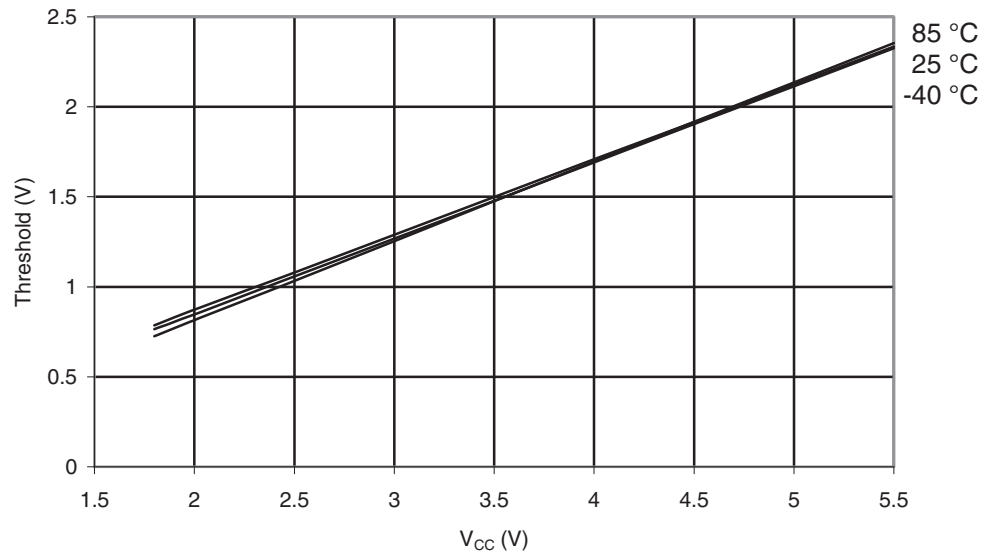
Figure 29-78. ATmega164PA: Reset Pin Input Threshold vs. V_{CC} ( V_{IL} , I/O Pin Read as '0').
