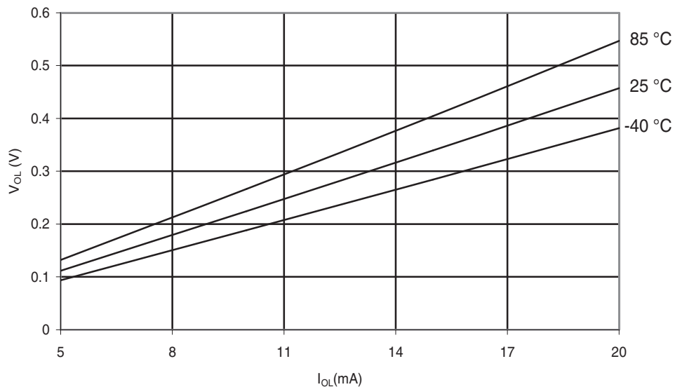
Figure 29-169. ATmega324PA: I/O Pin Output Voltage vs. Sink Current ( V_{CC} = 5V ).
