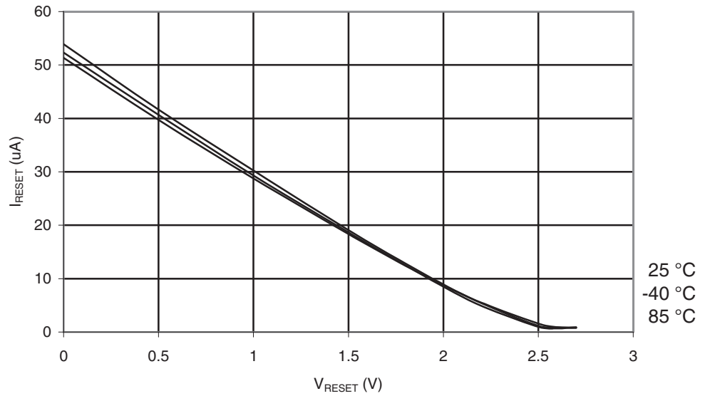
Figure 29-68. ATmega164PA: Reset Pull-up Resistor Current vs. Reset Pin Voltage ( V_{CC} = 2.7V ).
