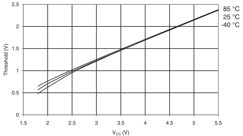
Figure 29-26. ATmega164A: I/O Pin Input Threshold vs. V_{CC} ( V_{IL} , I/O Pin Read as '0').
