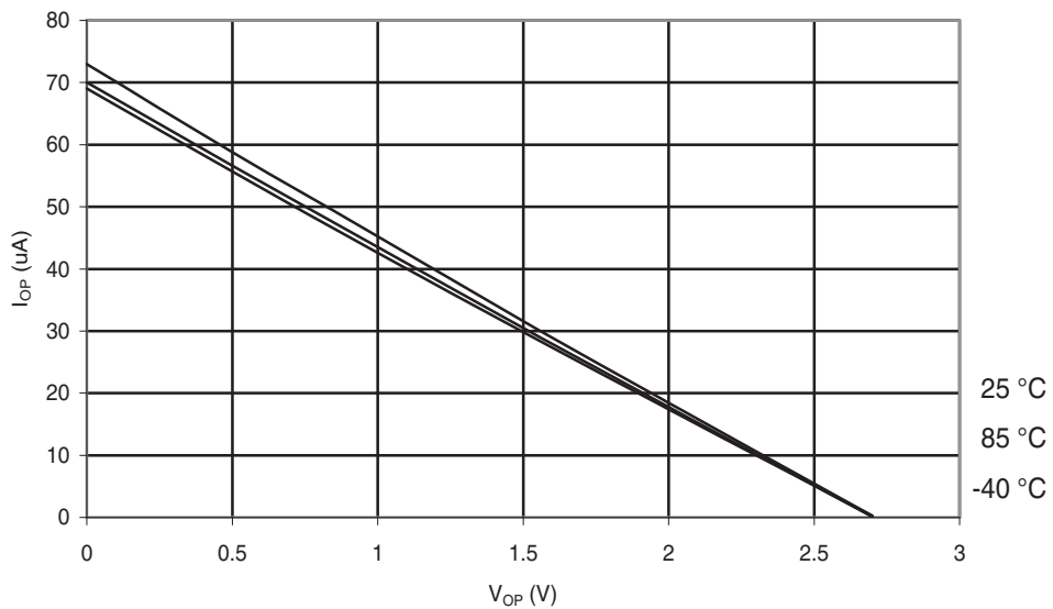
Figure 29-114. ATmega324A: I/O Pin Pull-up Resistor Current vs. Input Voltage ( V_{CC} = 2.7V ).
