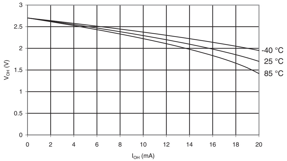
Figure 29-318. ATmega1284: I/O Pin Output Voltage vs. Source Current ( V_{CC} = 2.7V )
