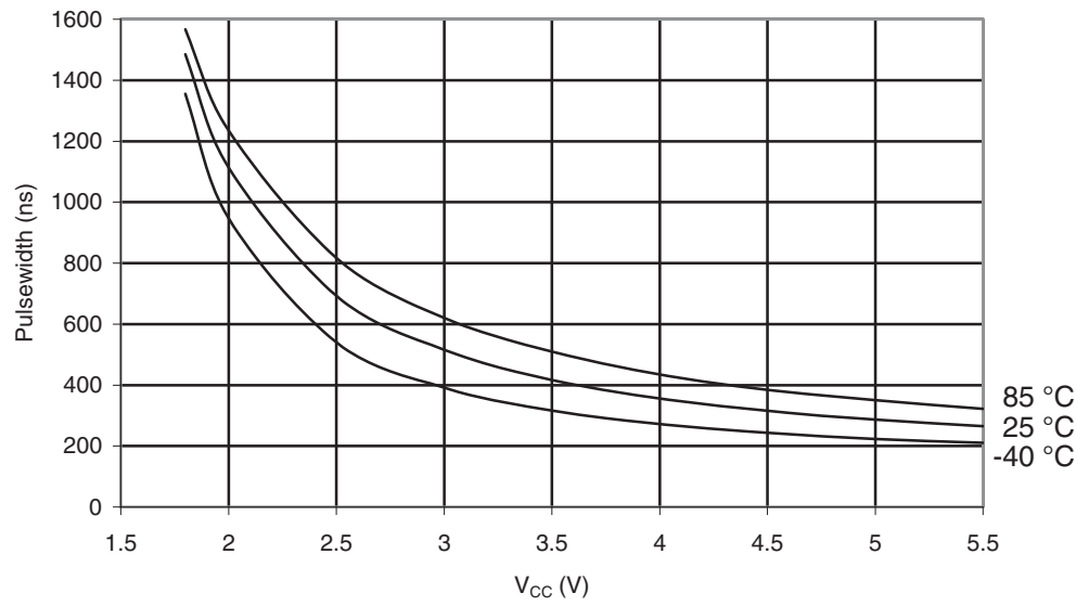
Figure 29-49. ATmega164A: Minimum Reset Pulsewidth vs. V_{CC}
