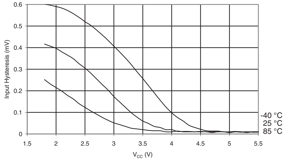
Figure 29-325. ATmega1284: Reset Pin Input Hysteresis vs. V_{CC}
