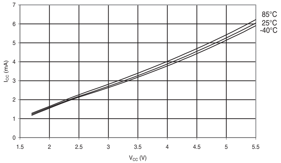
Figure 29-200. ATmega644A: Active Supply Current vs. V_{CC} (Internal RC Oscillator, 1MHz).
