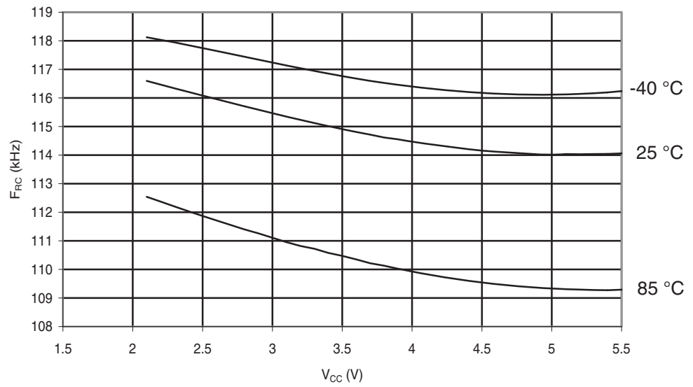
Figure 29-282. ATmega644PA: Watchdog Oscillator Frequency vs. V_{CC}
