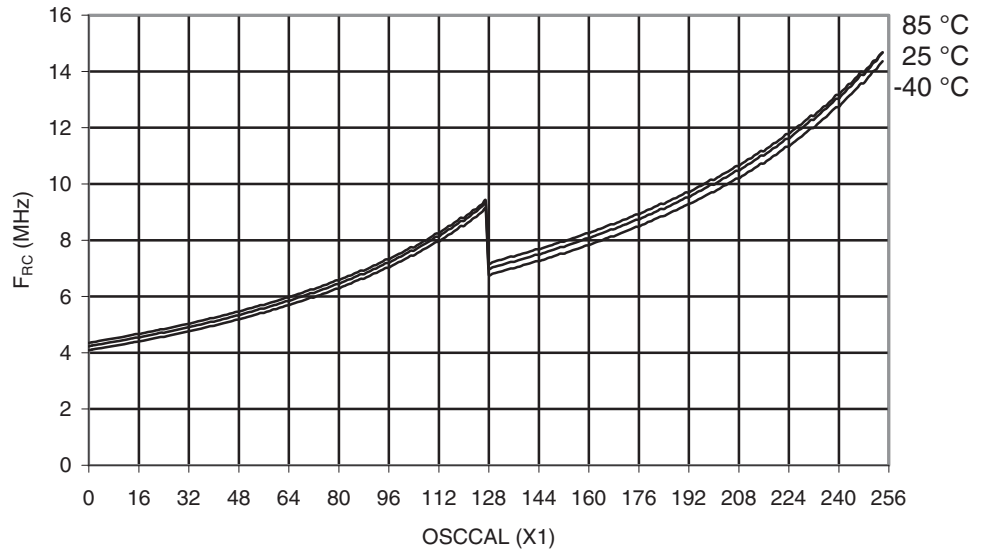
Figure 29-335. ATmega1284: Calibrated 8MHz RC Oscillator vs. OSCCAL Value
