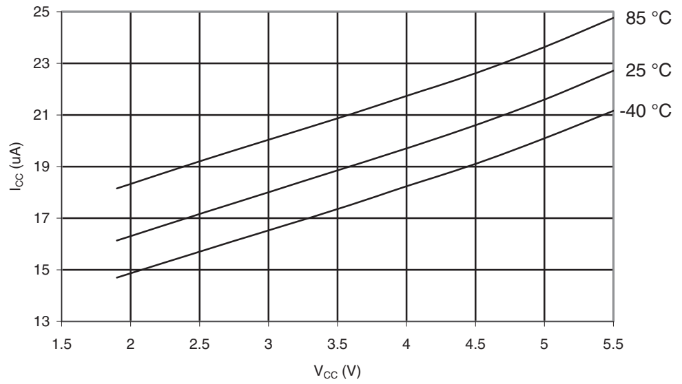
Figure 29-339. ATmega1284: Brownout Detector Current vs. V_{CC}
