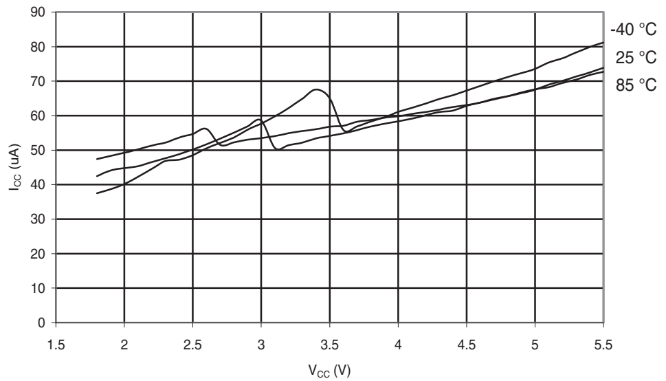
Figure 29-140. ATmega324A: Analog Comparator Current vs. V_{CC}
