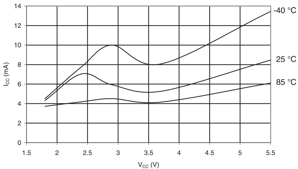
Figure 29-390. ATmega1284P: Programming Current vs. V_{CC}
