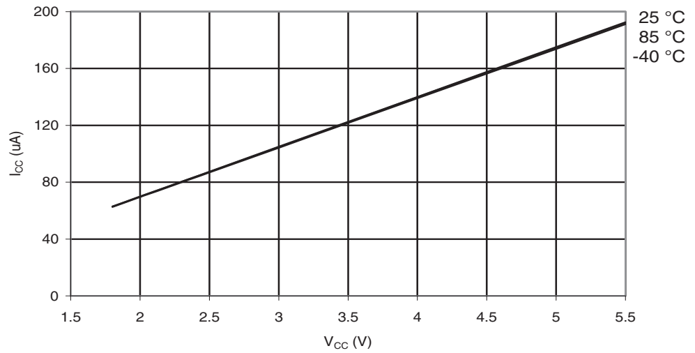
Figure 29-92. ATmega164PA: AREF External Reference Current vs. V_{CC}
