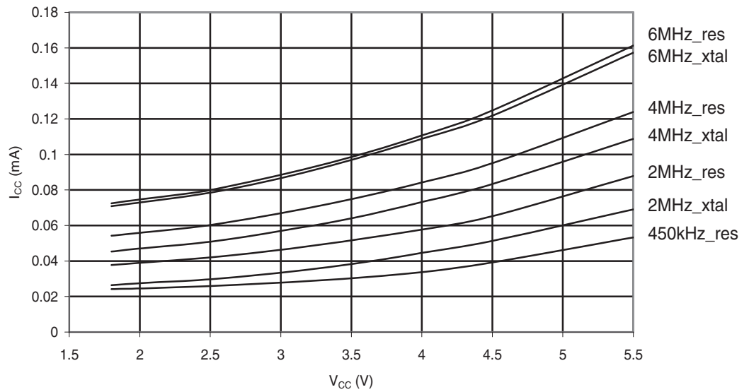
Figure 29-112. ATmega324A: Standby Supply Current vs. V_{CC} (Watchdog Timer Disabled).
