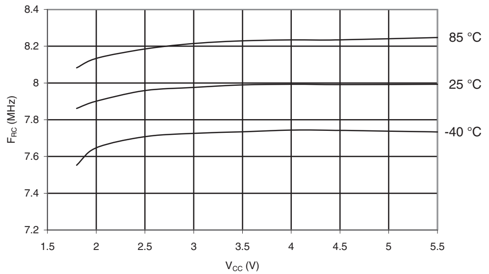
Figure 29-38. ATmega164A: Calibrated 8MHz RC Oscillator vs. V_{CC}
