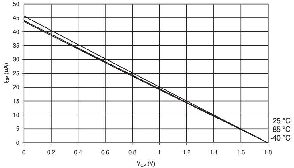
Figure 29-260. ATmega644PA: I/O Pin Pull-up Resistor Current vs. Input Voltage ( V_{CC} = 1.8V ).
