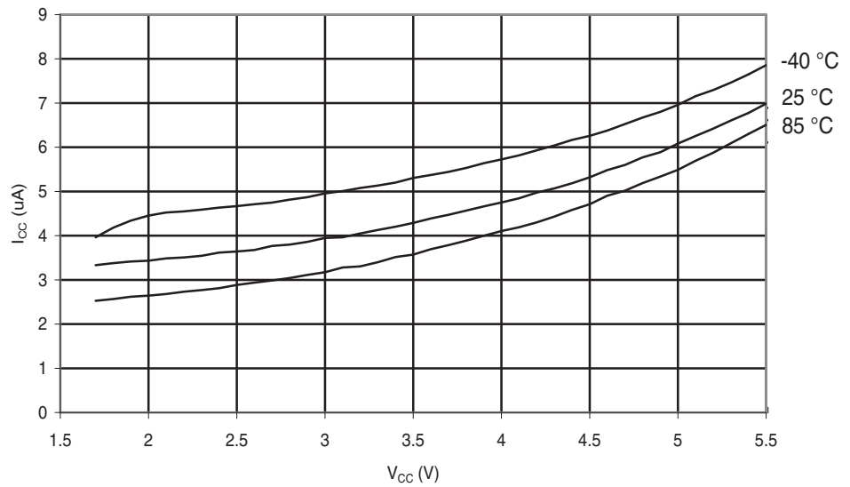
Figure 29-242. ATmega644A: Watchdog Timer Current vs. V_{CC}
