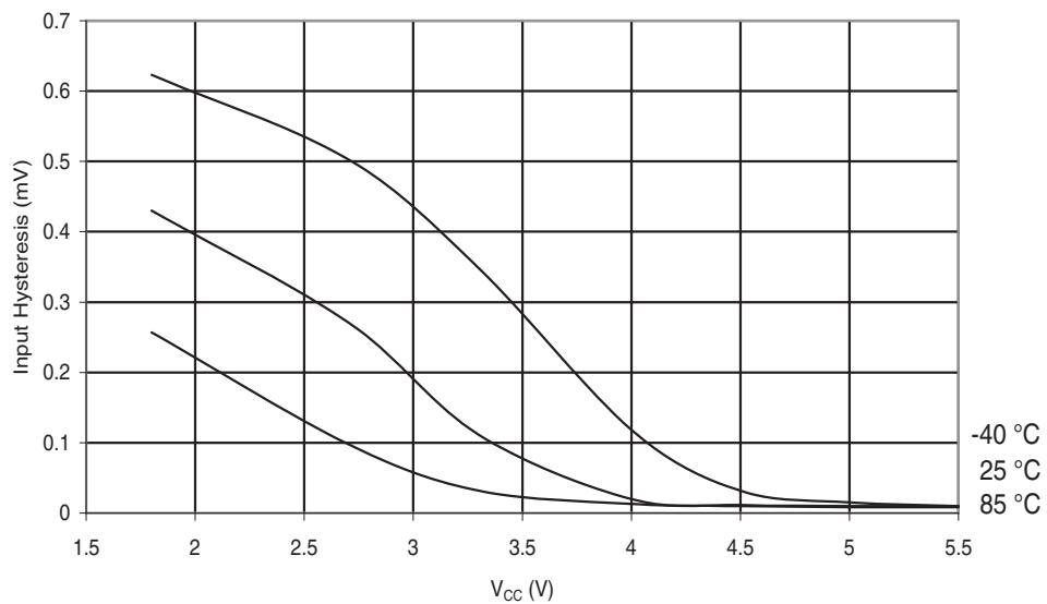
Figure 29-275. ATmega644PA: Reset Pin Input Hysteresis vs. V_{CC}
