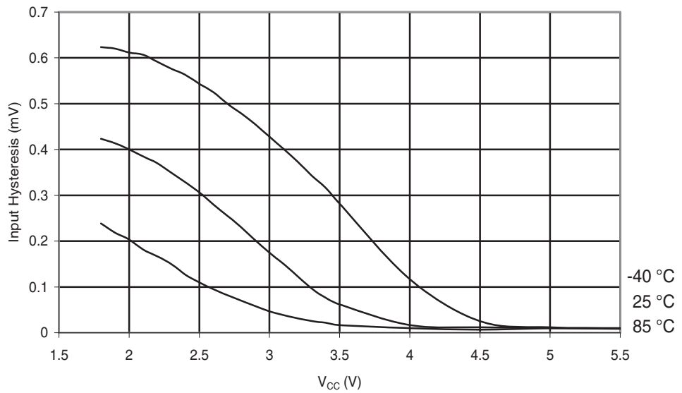
Figure 29-177. ATmega324PA: Reset Pin Input Hysteresis vs. V_{CC}
