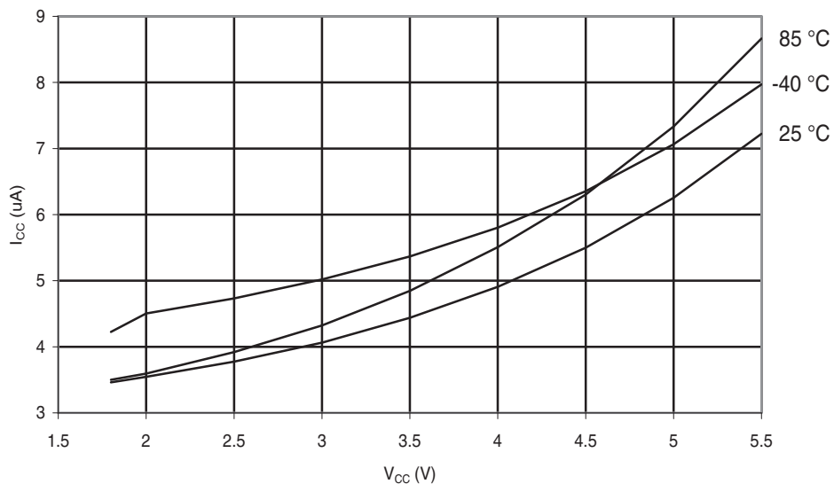
Figure 29-257. ATmega644PA: Power-down Supply Current vs. V_{CC} (Watchdog Timer Enabled).
