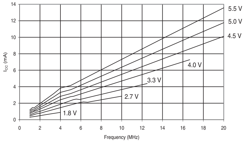
Figure 29-198. ATmega644A: Active Supply Current vs. Frequency (1 - 20MHz).
