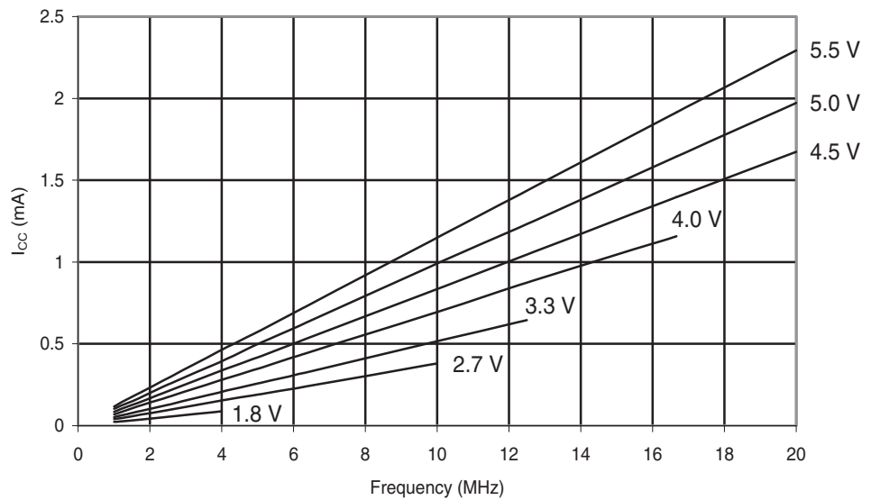
Figure 29-146. ATmega324A: Reset Supply Current vs. Frequency (1 - 20MHz)
