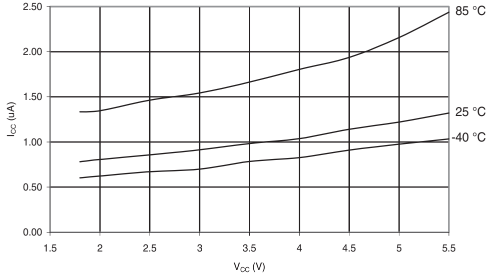
Figure 29-111. ATmega324A: Power-save Supply Current vs. V_{CC} (Watchdog Timer Disabled and 32kHz Crystal Oscillator Running).
