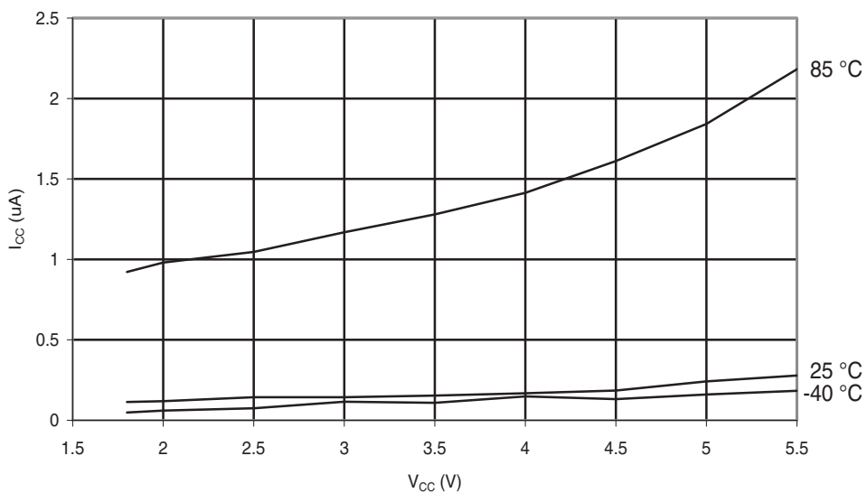
Figure 29-256. ATmega644PA: Power-down Supply Current vs. V_{CC} (Watchdog Timer Disabled).
