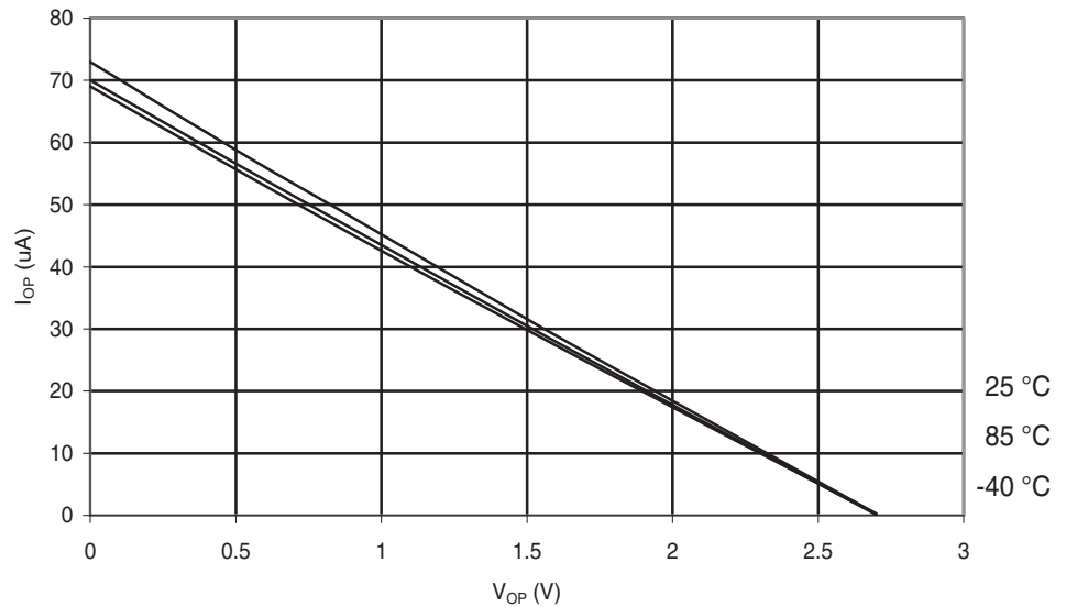
Figure 29-163. ATmega324PA: I/O Pin Pull-up Resistor Current vs. Input Voltage ( V_{CC} = 2.7V ).
