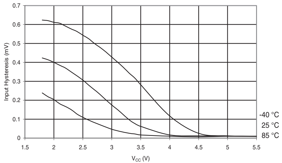
Figure 29-128. ATmega324A: Reset Pin Input Hysteresis vs. V_{CC}
