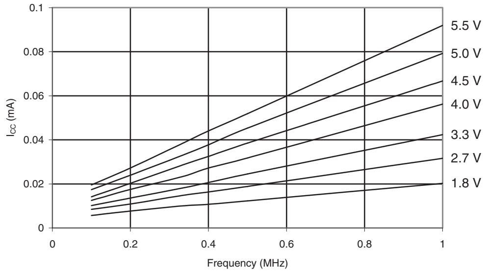
Figure 29-47. ATmega164A: Reset Supply Current vs. Low Frequency (0.1 - 1.0MHz).
