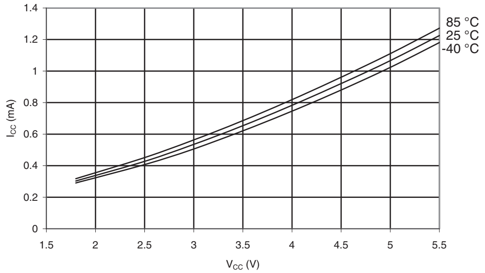
Figure 29-253. ATmega644PA: Idle Supply Current vs. V_{CC} (Internal RC Oscillator, 8MHz).
