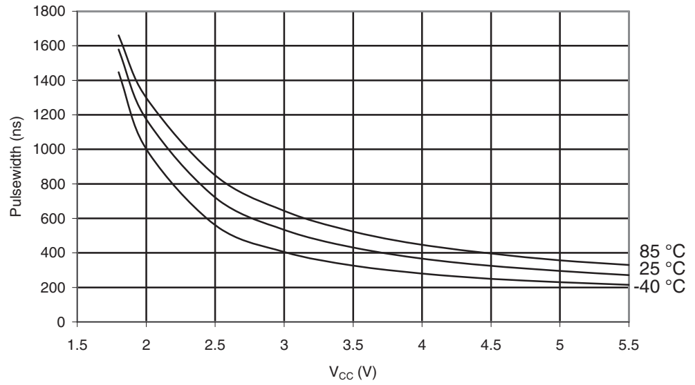
Figure 29-294. ATmega644PA: Minimum Reset Pulsewidth vs. V_{CC}
