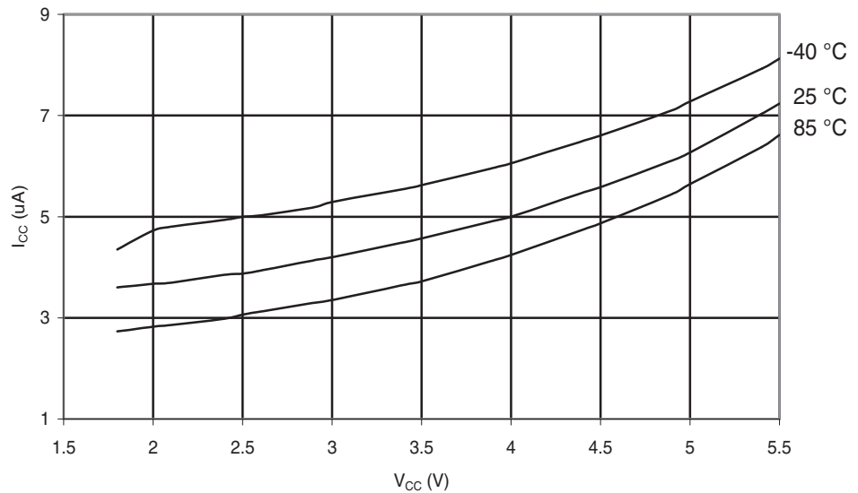
Figure 29-193. ATmega324PA: Watchdog Timer Current vs. V_{CC}
