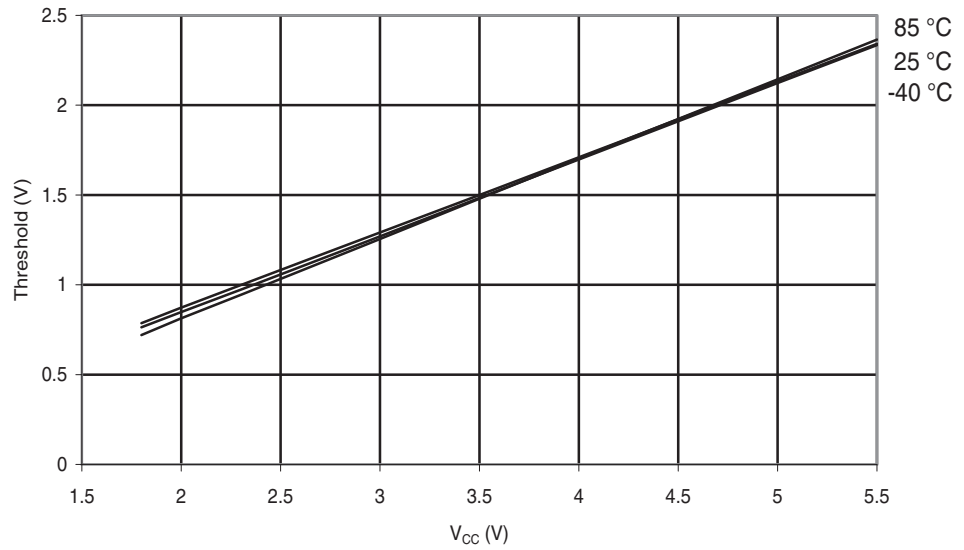
Figure 29-225. ATmega644A: Reset Pin Input Threshold vs. V_{CC} ( V_{IL} , I/O Pin Read as '0').
