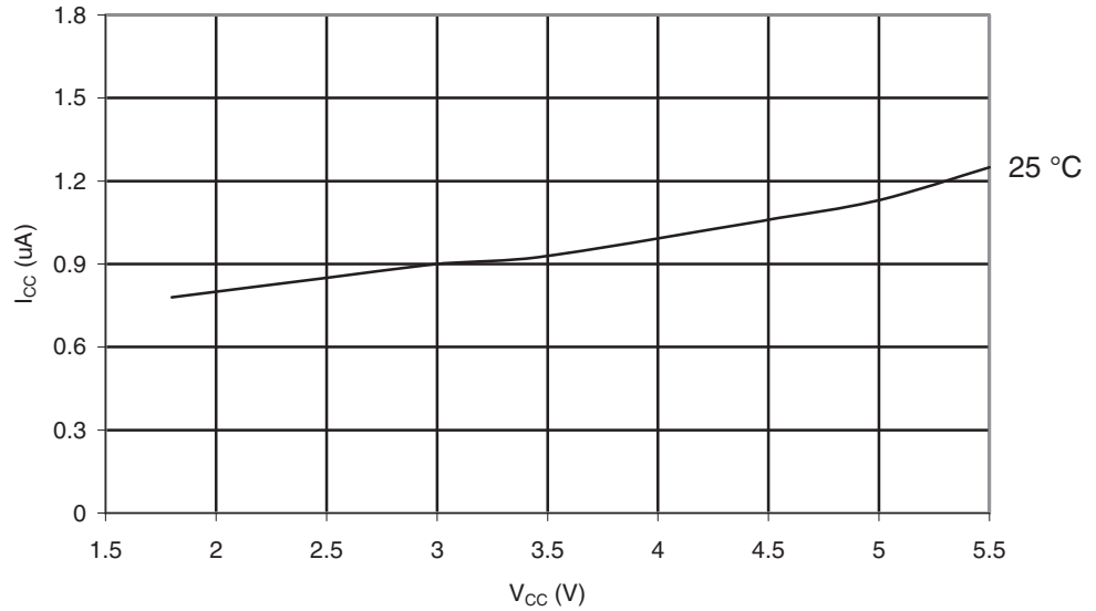
Figure 29-13. ATmega164A: Power-save Supply Current vs. V_{CC} (Watchdog Timer Disabled and 32kHz Crystal Oscillator Running).
