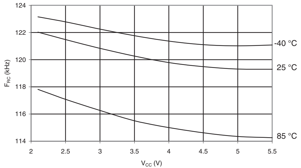
Figure 29-382. ATmega1284P: Watchdog Oscillator Frequency vs. V_{CC}
