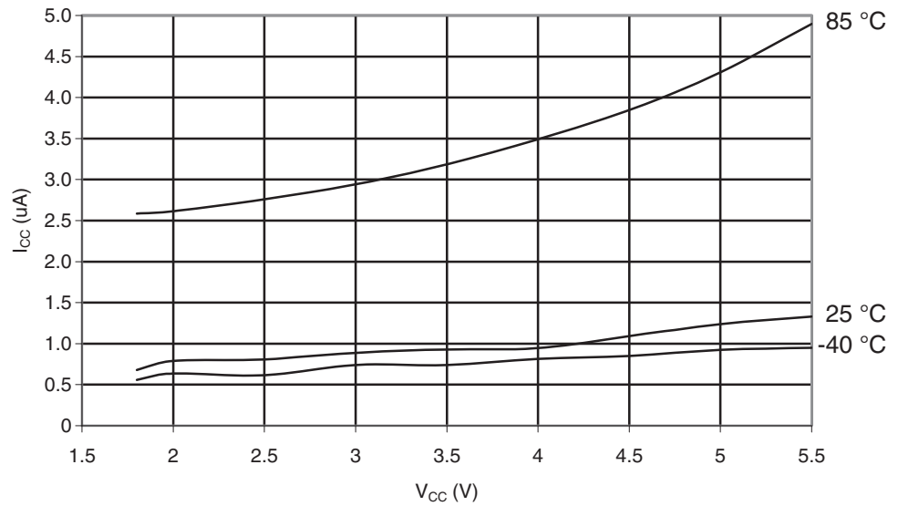
Figure 29-357. ATmega1284P: Power-save Supply Current vs. V_{CC} (Watchdog Timer Disabled and 32kHz Crystal Oscillator Running)
