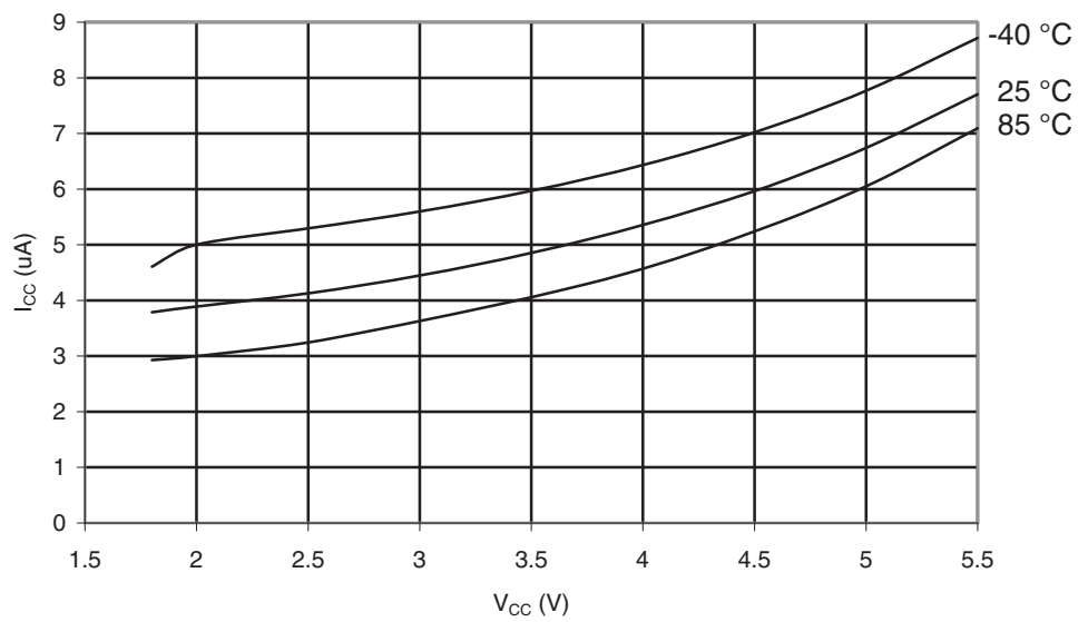
Figure 29-95. ATmega164PA: Watchdog Timer Current vs. V_{CC}
