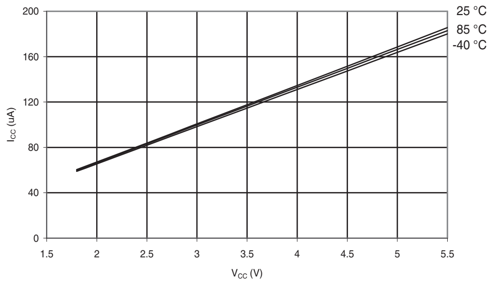
Figure 29-190. ATmega324PA: AREF External Reference Current vs. V_{CC}
