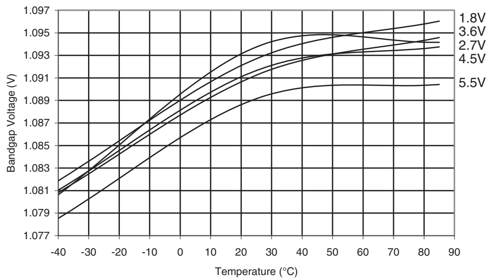
Figure 29-133. ATmega324A: Bandgap Voltage vs. Temperature
