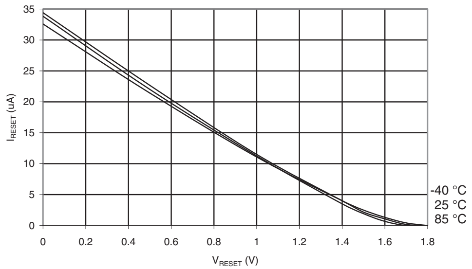
Figure 29-312. ATmega1284: Reset Pull-up Resistor Current vs. Reset Pin Voltage ( V_{CC} = 1.8V )
