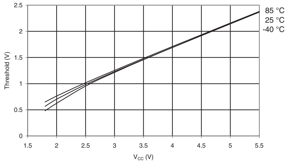
Figure 29-75. ATmega164PA: I/O Pin Input Threshold vs. V_{CC} ( V_{IL} , I/O Pin Read as '0').
