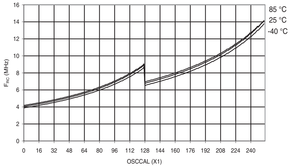
Figure 29-285. ATmega644PA: Calibrated 8MHz RC Oscillator vs. OSCCAL Value
