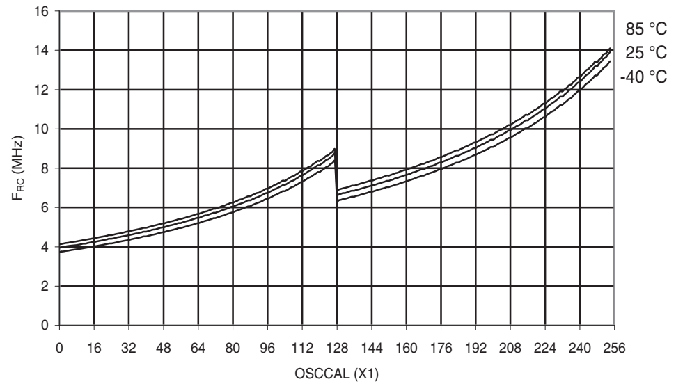
Figure 29-138. ATmega324A: Calibrated 8MHz RC Oscillator vs. OSCCAL Value
