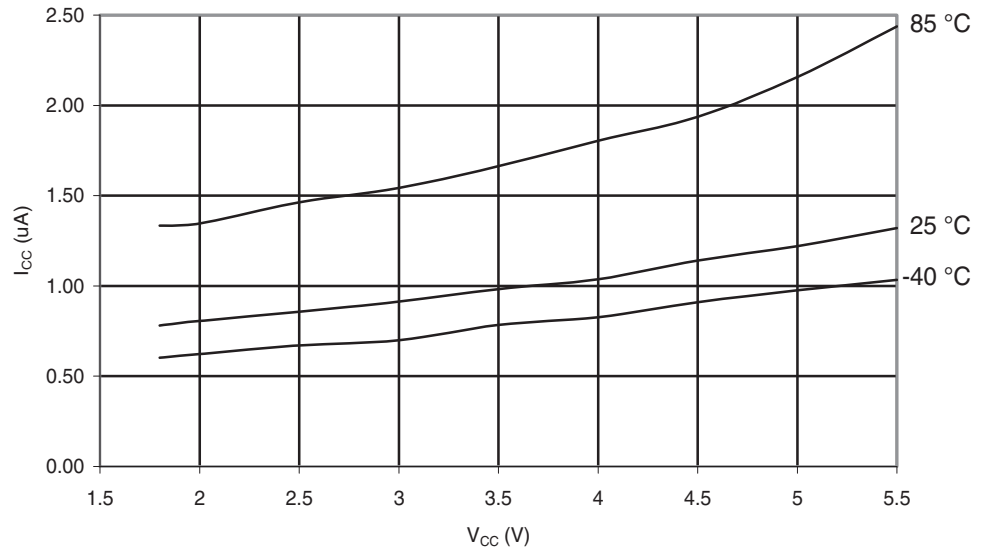
Figure 29-160. ATmega324PA: Power-save Supply Current vs. V_{CC} (Watchdog Timer Disabled and 32kHz Crystal Oscillator Running).
