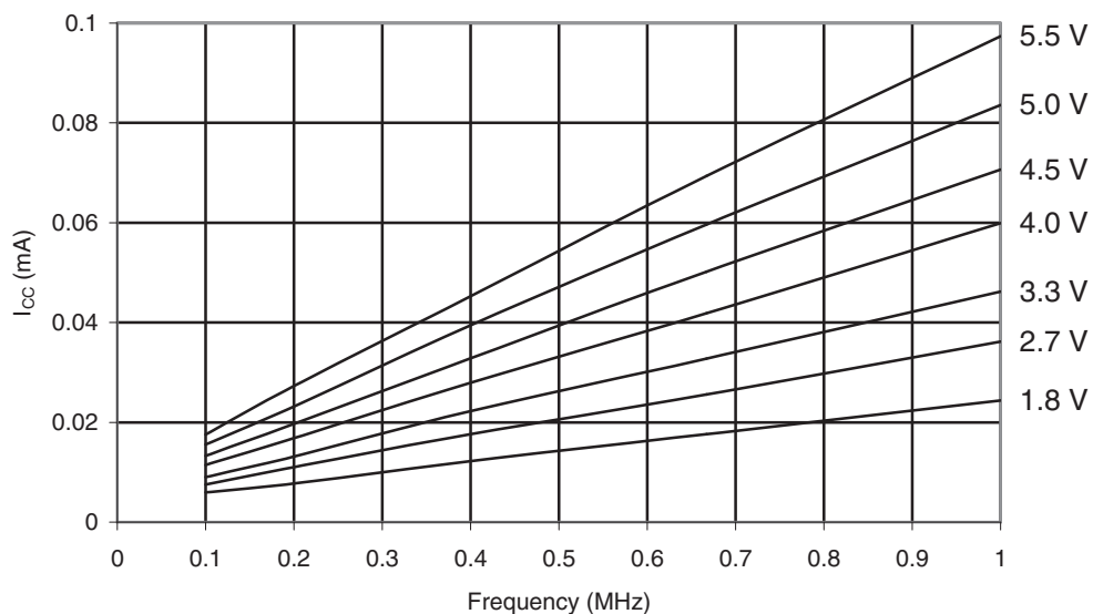
Figure 29-392. ATmega1284P: Reset Supply Current vs. Low Frequency (0.1 - 1.0MHz)
