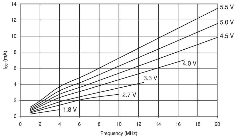
Figure 29-149. ATmega324PA: Active Supply Current vs. Frequency (1 - 20MHz).
