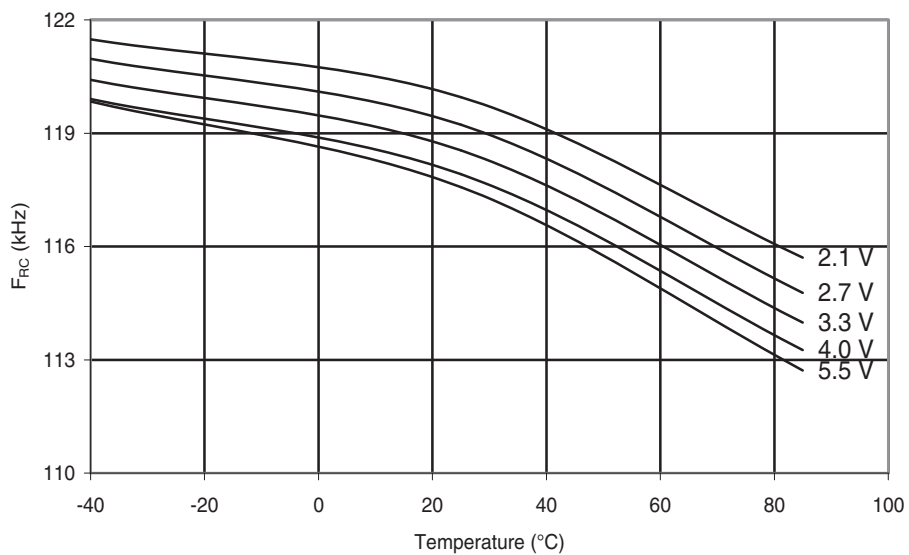
Figure 29-134. ATmega324A: Watchdog Oscillator Frequency vs. Temperature
