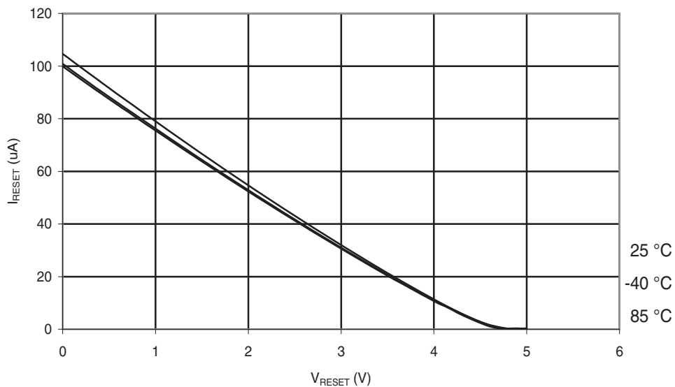
Figure 29-118. ATmega324A: Reset Pull-up Resistor Current vs. Reset Pin Voltage ( V_{CC} = 5V ).
