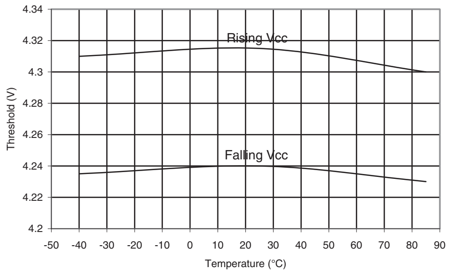
Figure 29-31. ATmega164A: BOD Threshold vs. Temperature ( V_{BOT} = 4.3V )
