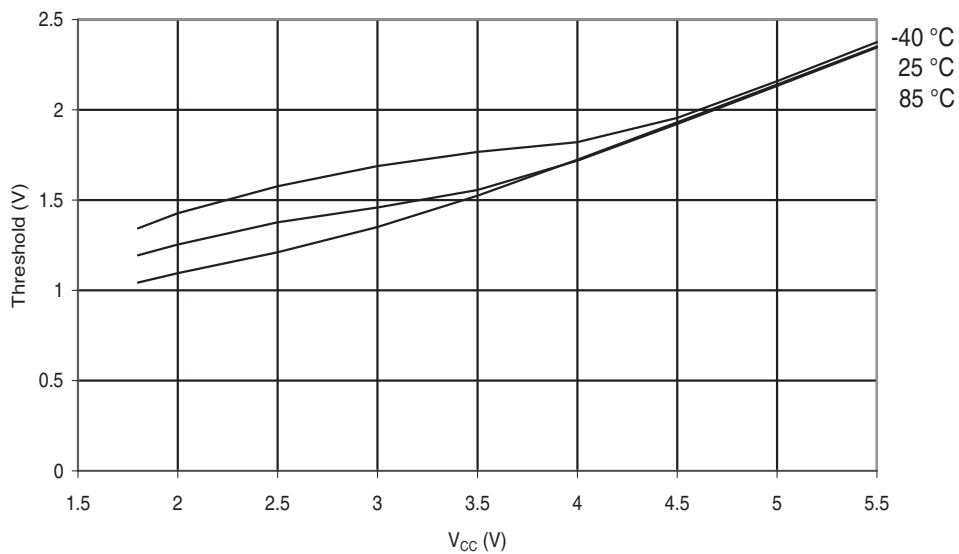
Figure 29-224. ATmega644A: Reset Pin Input Threshold vs. V_{CC} ( V_{IH} , I/O Pin Read as '1').
