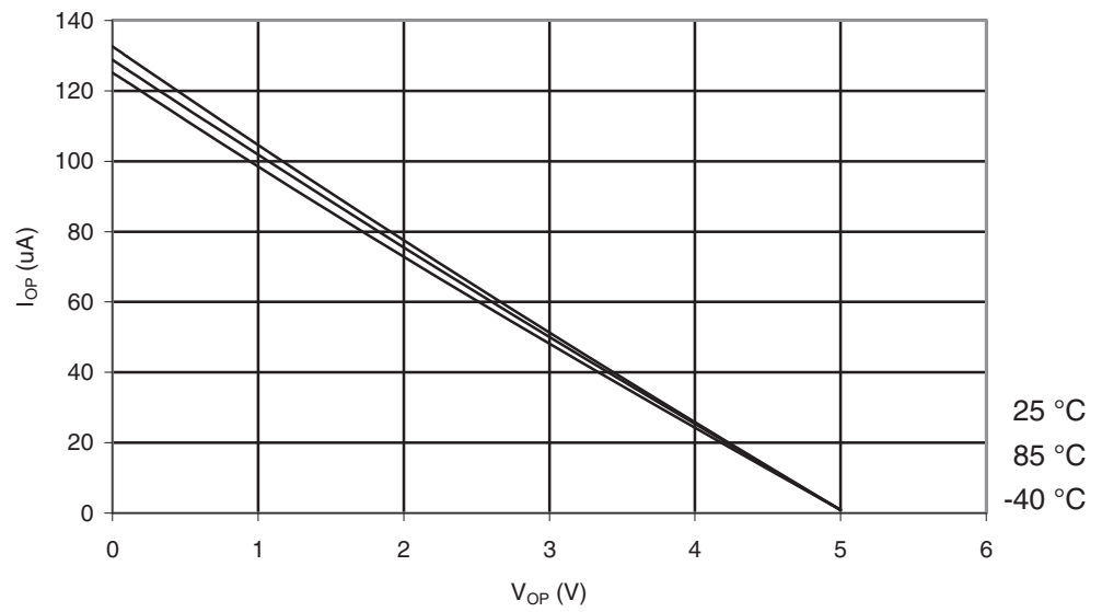
Figure 29-66. ATmega164PA: I/O Pin Pull-up Resistor Current vs. Input Voltage ( V_{CC} = 5V ).
