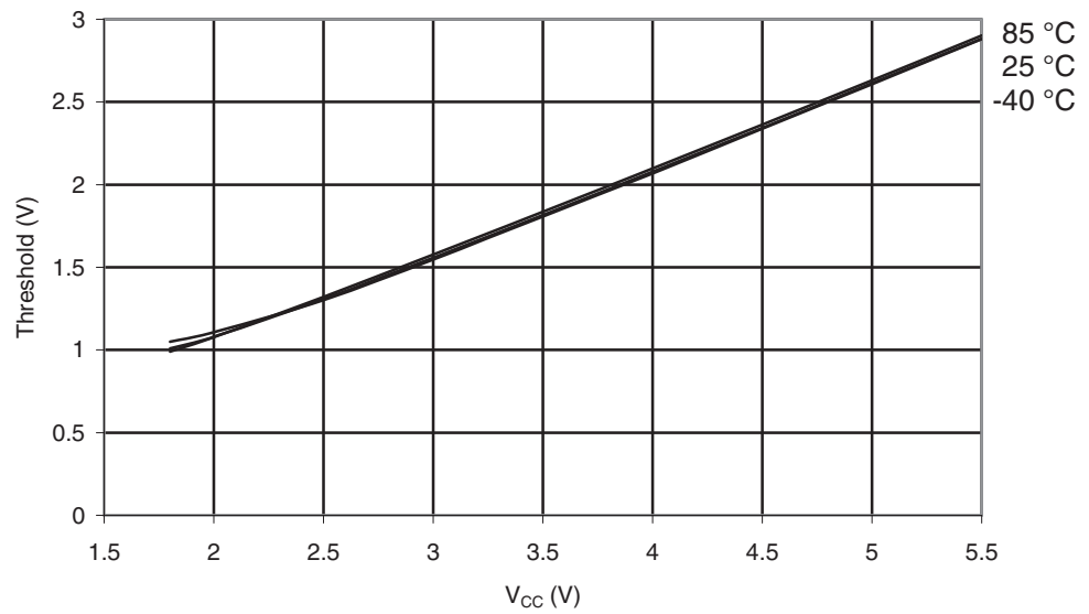
Figure 29-74. ATmega164PA: I/O Pin Input Threshold vs. V_{CC} ( V_{IH} , I/O Pin Read as '1').
