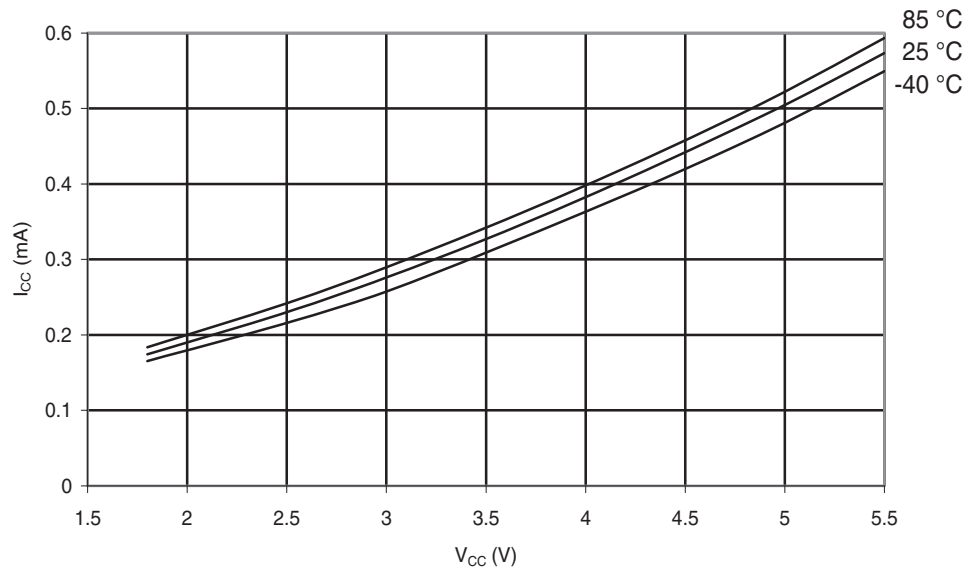
Figure 29-156. ATmega324PA: Idle Supply Current vs. V_{CC} (Internal RC Oscillator, 1MHz).
