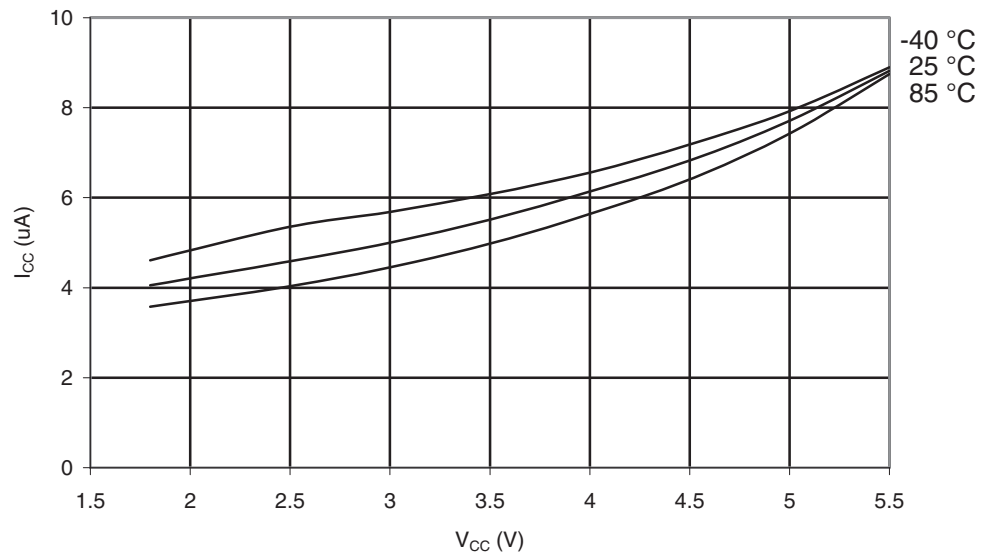
Figure 29-61. ATmega164PA: Power-down Supply Current vs. V_{CC} (Watchdog Timer Enabled).
