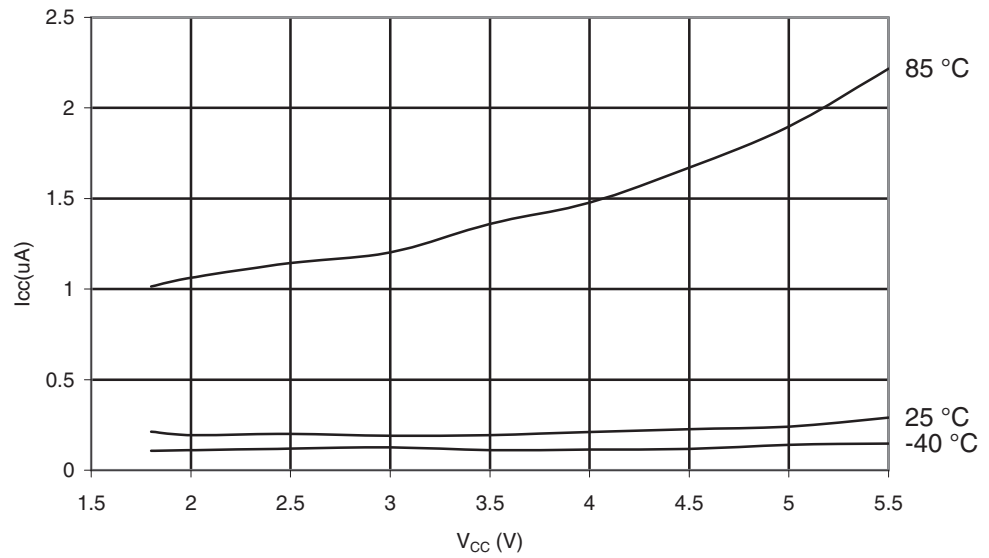
Figure 29-209. ATmega644A: Power-save Supply Current vs. V_{CC} (Watchdog Timer Disabled and 32kHz Crystal Oscillator Running)
