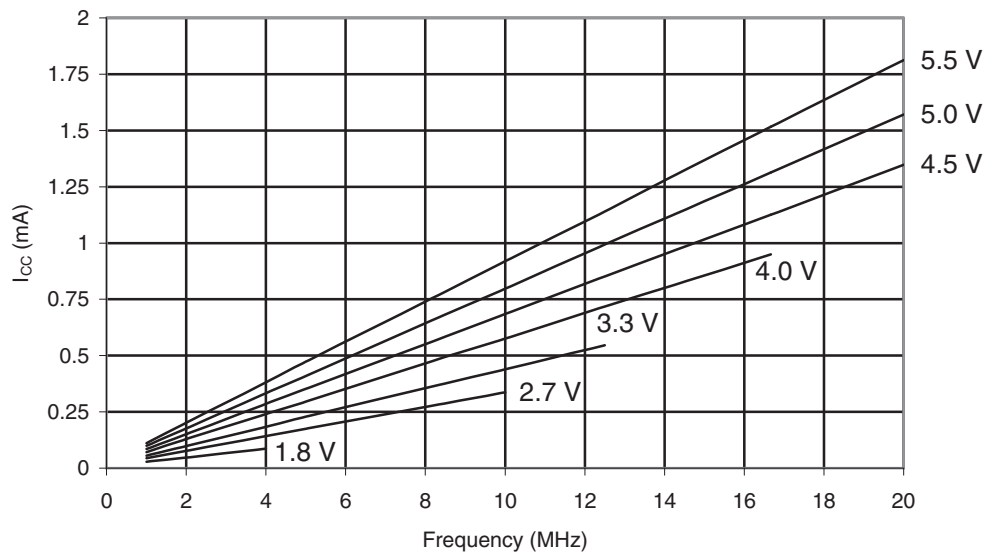
Figure 29-293. ATmega644PA: Reset Supply Current vs. Frequency (1 - 20MHz)
