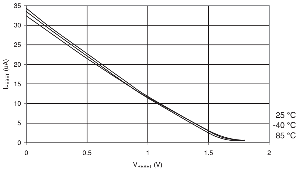
Figure 29-18. ATmega164A: Reset Pull-up Resistor Current vs. Reset Pin Voltage ( V_{CC} = 1.8V ).
