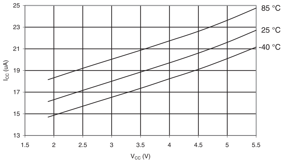
Figure 29-389. ATmega1284P: Brownout Detector Current vs. V_{CC}
