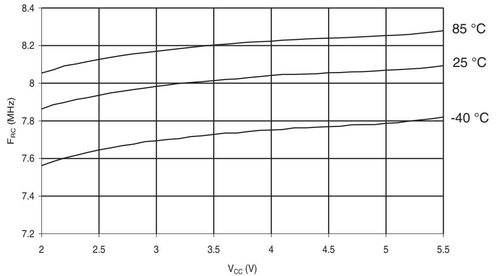
Figure 29-283. ATmega644PA: Calibrated 8MHz RC Oscillator vs. V_{CC}
