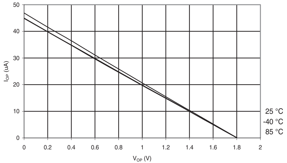
Figure 29-162. ATmega324PA: I/O Pin Pull-up Resistor Current vs. Input Voltage ( V_{CC} = 1.8V ).
