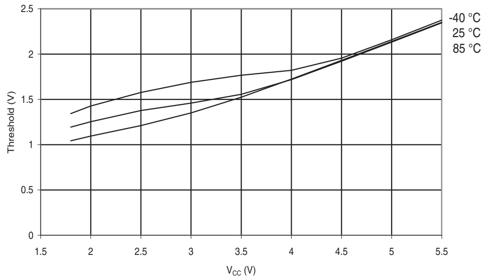
Figure 29-273. ATmega644PA: Reset Pin Input Threshold vs. V_{CC} ( V_{IH} , I/O Pin Read as '1').
