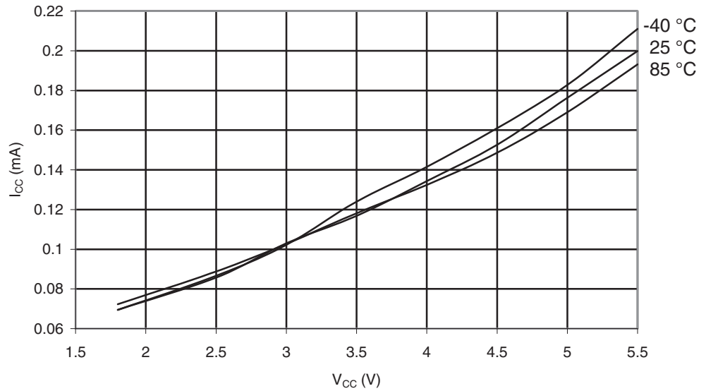
Figure 29-250. ATmega644PA: Active Supply Current vs. V_{CC} (Internal RC Oscillator, 128kHz).
