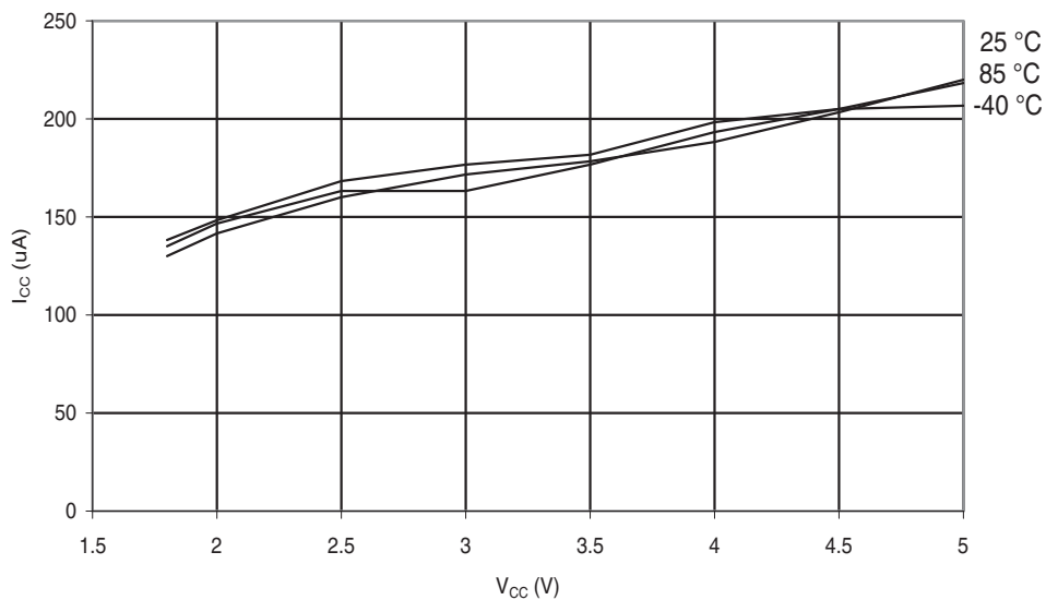
Figure 29-286. ATmega644PA: ADC Current vs. V_{CC} (AREF = AV_{CC} )
