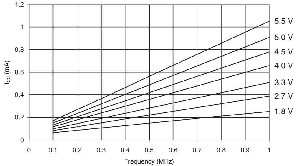
Figure 29-1. ATmega164A: Active Supply Current vs. Low Frequency (0.1 - 1.0MHz).
