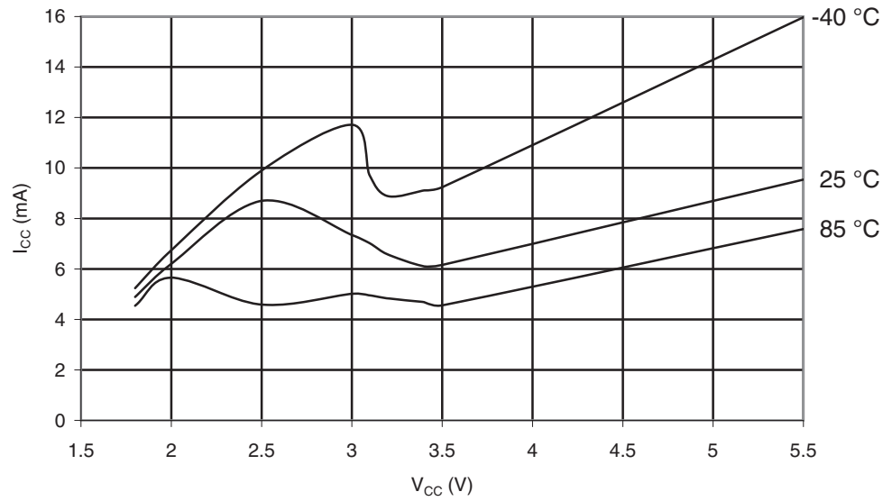
Figure 29-290. ATmega644PA: Programming Current vs. V_{CC}
