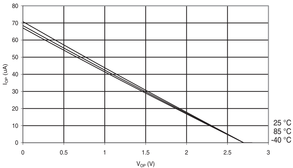
Figure 29-212. ATmega644A: I/O Pin Pull-up Resistor Current vs. Input Voltage ( V_{CC} = 2.7V ).
