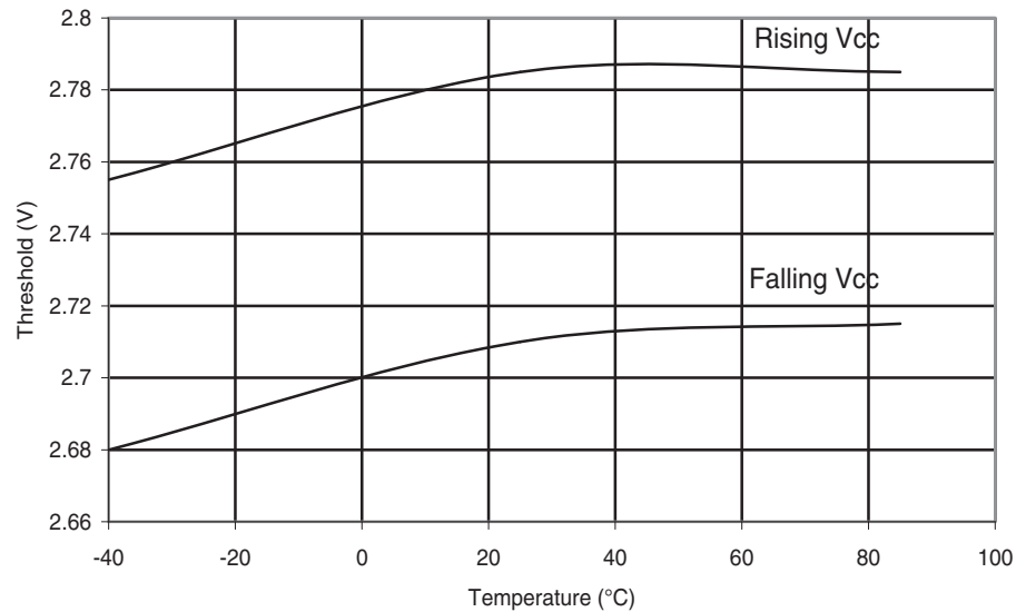
Figure 29-179. ATmega324PA: BOD Threshold vs. Temperature ( V_{BOT} = 2.7V )
