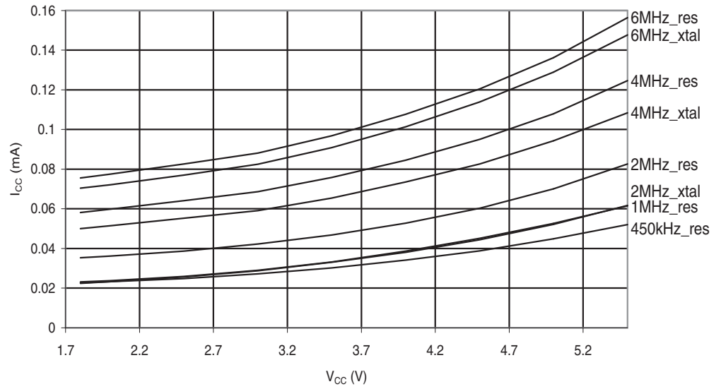
Figure 29-259. ATmega644PA: Standby Supply Current vs. V_{CC} (Watchdog Timer Disabled).
