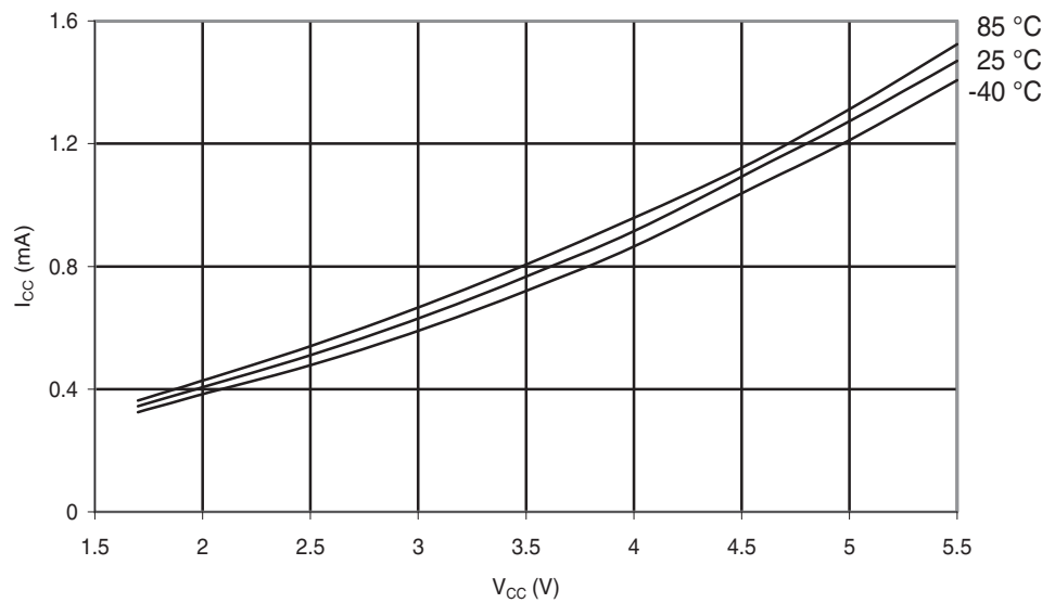
Figure 29-151. ATmega324PA: Active Supply Current vs. V_{CC} (Internal RC Oscillator, 1MHz).
