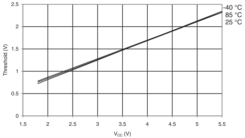
Figure 29-324. ATmega1284: Reset Pin Input Threshold vs. V_{CC} ( V_{IL} , I/O Pin Read as '0')
