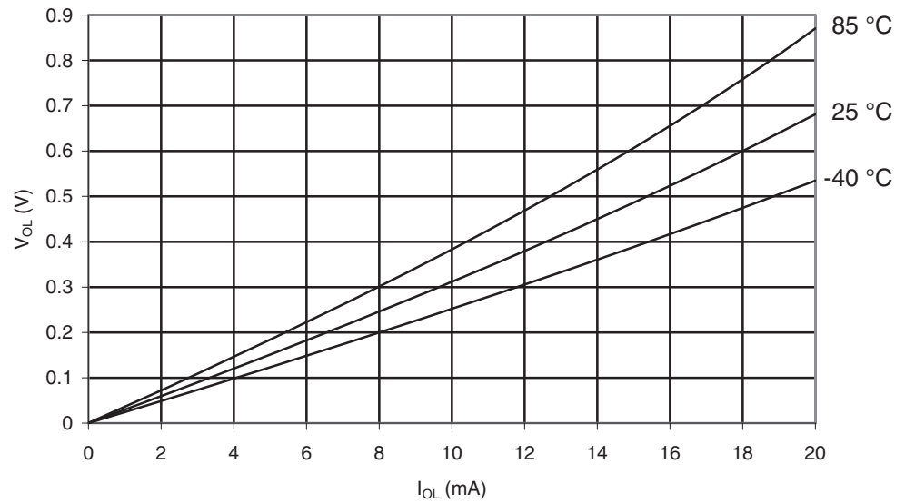
Figure 29-366. ATmega1284P: I/O Pin Output Voltage vs. Sink Current ( V_{CC} = 3V )
