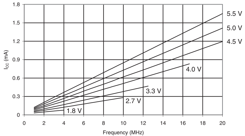
Figure 29-97. ATmega164PA: Reset Supply Current vs. Frequency (1 - 20MHz).
