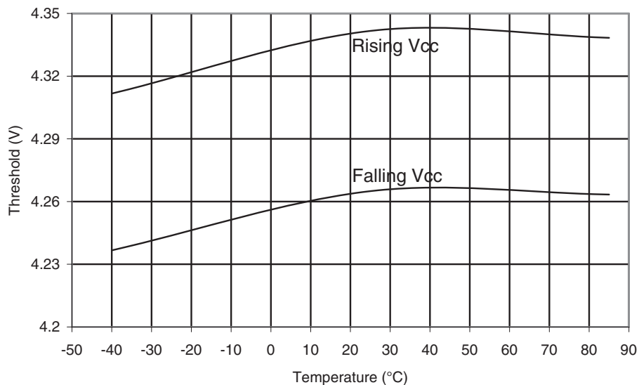
Figure 29-276. ATmega644PA: BOD Threshold vs. Temperature ( V_{BOT} = 4.3V )
