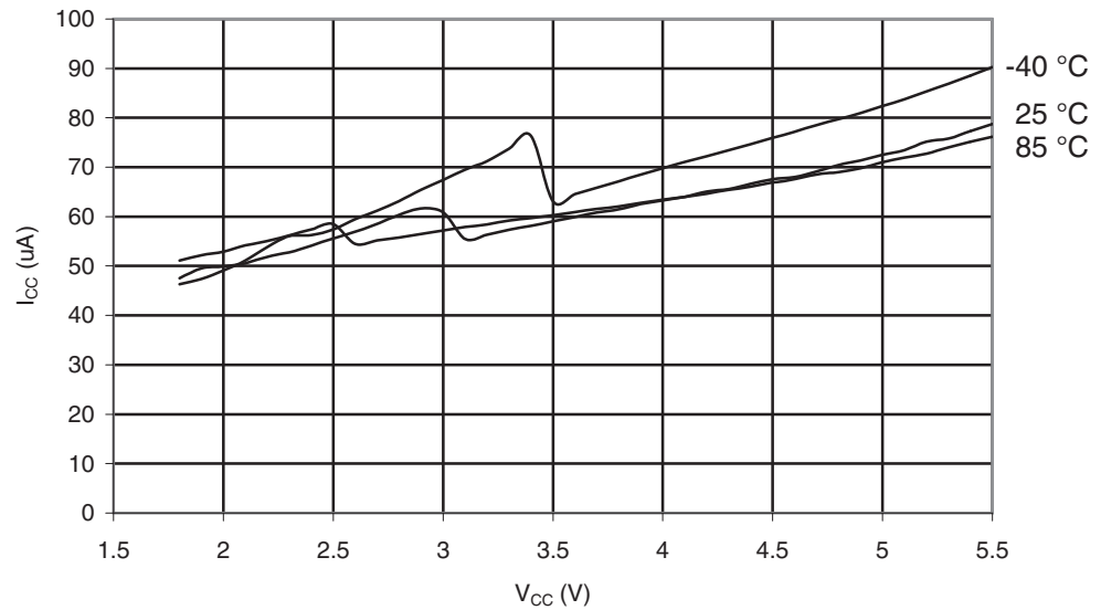
Figure 29-91. ATmega164PA: Analog Comparator Current vs. V_{CC}
