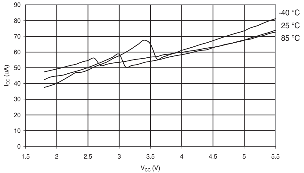
Figure 29-189. ATmega324PA: Analog Comparator Current vs. V_{CC}
