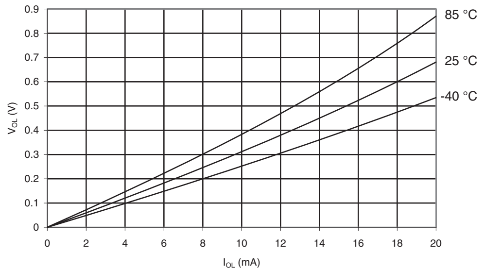
Figure 29-316. ATmega1284: I/O Pin Output Voltage vs. Sink Current ( V_{CC} = 3V )
