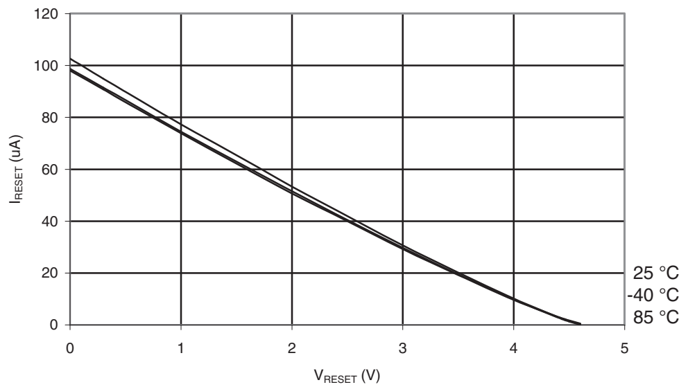
Figure 29-216. ATmega644A: Reset Pull-up Resistor Current vs. Reset Pin Voltage ( V_{CC} = 5V ).
