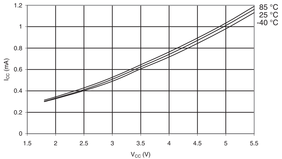
Figure 29-4. ATmega164A: Active Supply Current vs. V_{CC} (Internal RC Oscillator, 1MHz).
