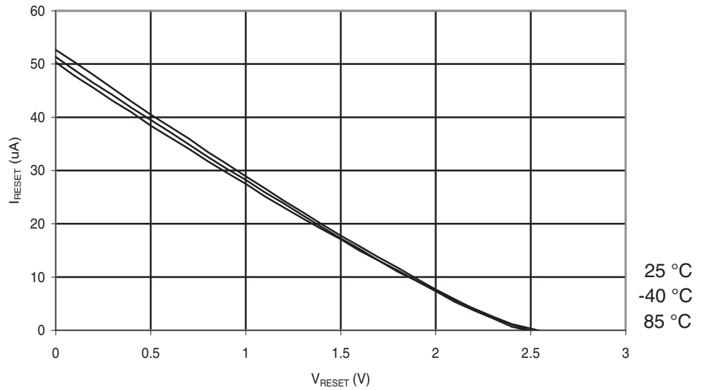
Figure 29-265. ATmega644PA: Reset Pull-up Resistor Current vs. Reset Pin Voltage ( V_{CC} = 5V ).
