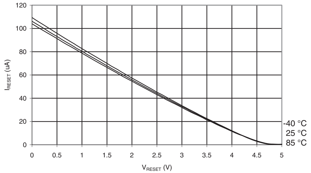
Figure 29-314. ATmega1284: Reset Pull-up Resistor Current vs. Reset Pin Voltage ( V_{CC} = 5V )
