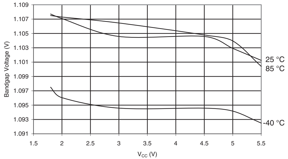
Figure 29-83. ATmega164PA: Calibrated Bandgap Voltage vs. V_{CC}
