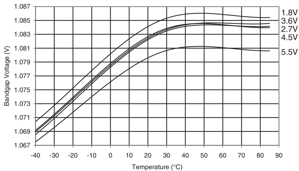
Figure 29-84. ATmega164PA: Bandgap Voltage vs. Temperature
