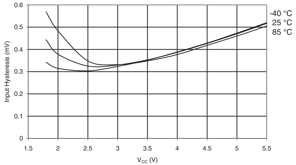
Figure 29-76. ATmega164PA: I/O Pin Input Hysteresis vs. V_{CC}
