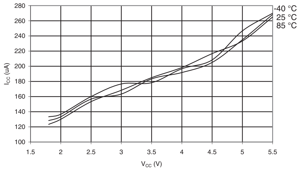
Figure 29-386. ATmega1284P: ADC Current vs. V_{CC} (AREF = AV_{CC} )
