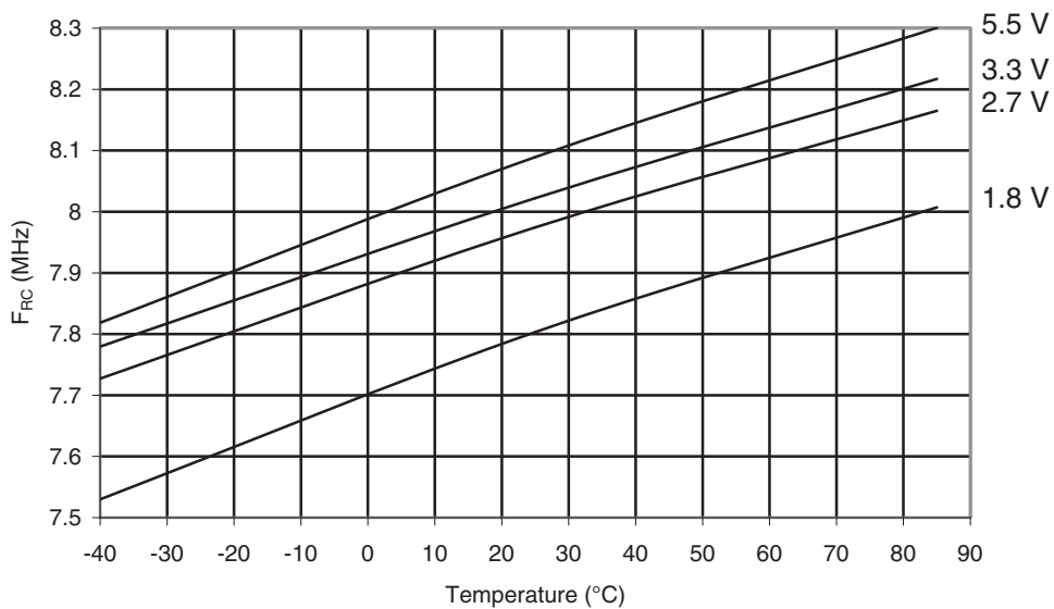
Figure 29-384. ATmega1284P: Calibrated 8MHz RC Oscillator vs. Temperature
