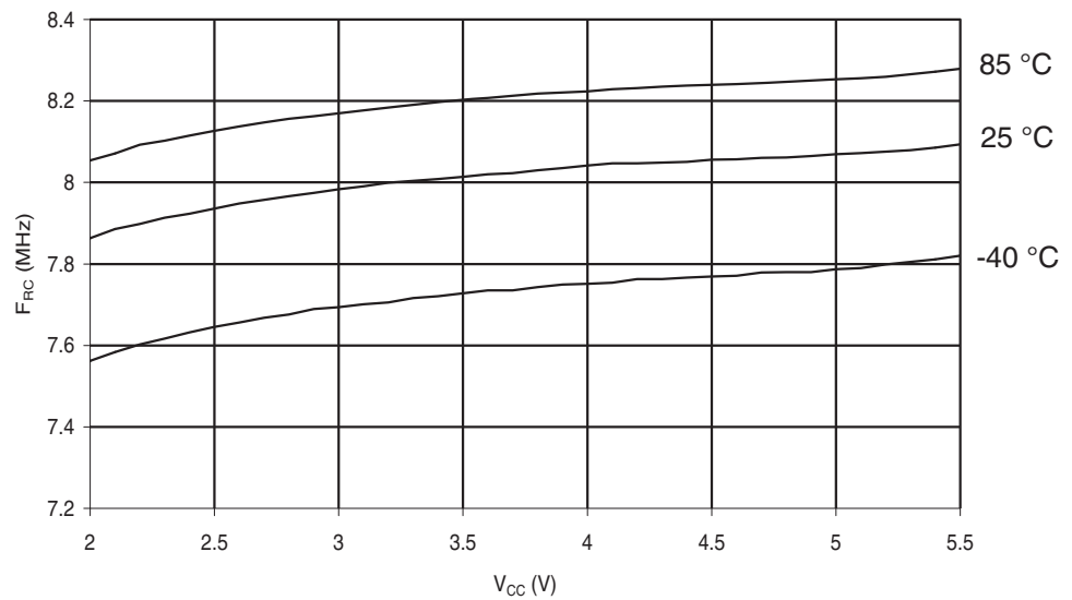
Figure 29-234. ATmega644A: Calibrated 8MHz RC Oscillator vs. V_{CC}
