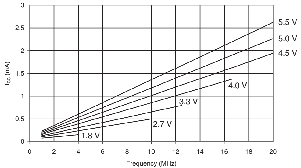
Figure 29-7. ATmega164A: Idle Supply Current vs. V_{CC} (1 - 20MHz).
