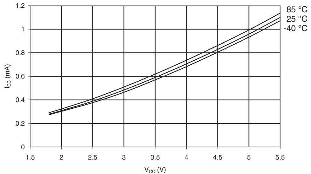
Figure 29-8. ATmega164A: Idle Supply Current vs. V_{CC} (Internal RC Oscillator, 8MHz).
