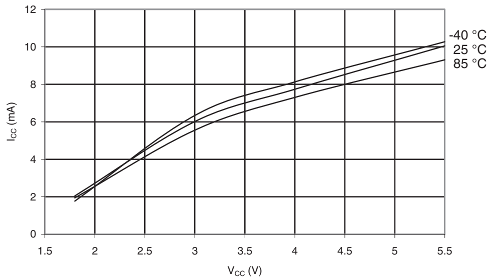
Figure 29-45. ATmega164A: Programming Current vs. V_{CC}
