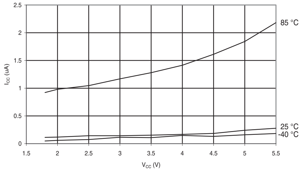
Figure 29-207. ATmega644A: Power-down Supply Current vs. V_{CC} (Watchdog Timer Disabled)
