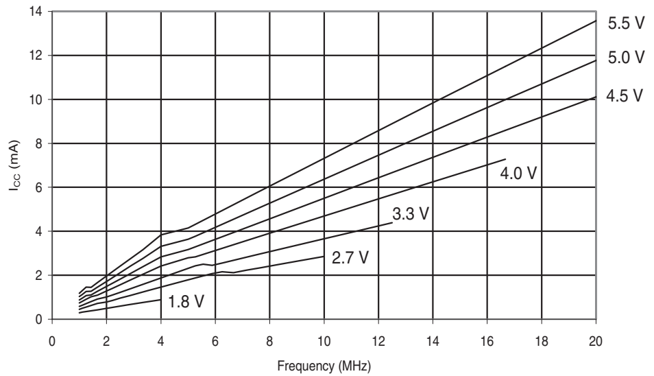
Figure 29-247. ATmega644PA: Active Supply Current vs. Frequency (1 - 20MHz).
