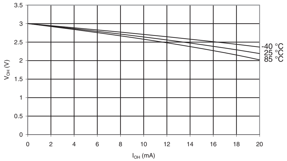
Figure 29-369. ATmega1284P: I/O Pin Output Voltage vs. Source Current ( V_{CC} = 3V )
