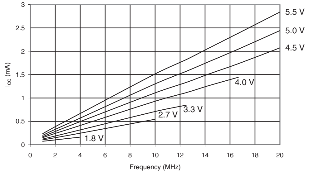
Figure 29-351. ATmega1284P: Idle Supply Current vs. Frequency (1 - 20MHz)
