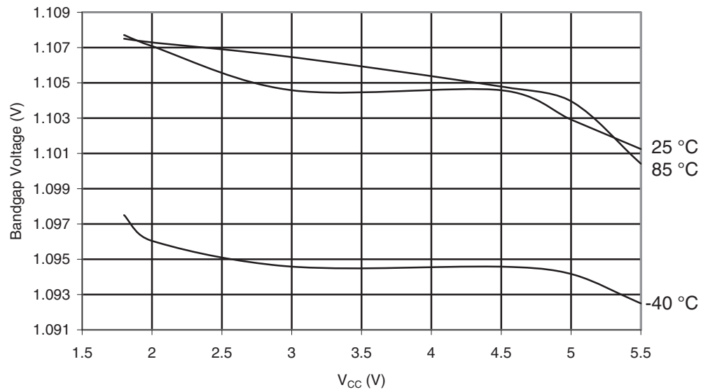
Figure 29-34. ATmega164A: Calibrated Bandgap Voltage vs. V_{CC}
