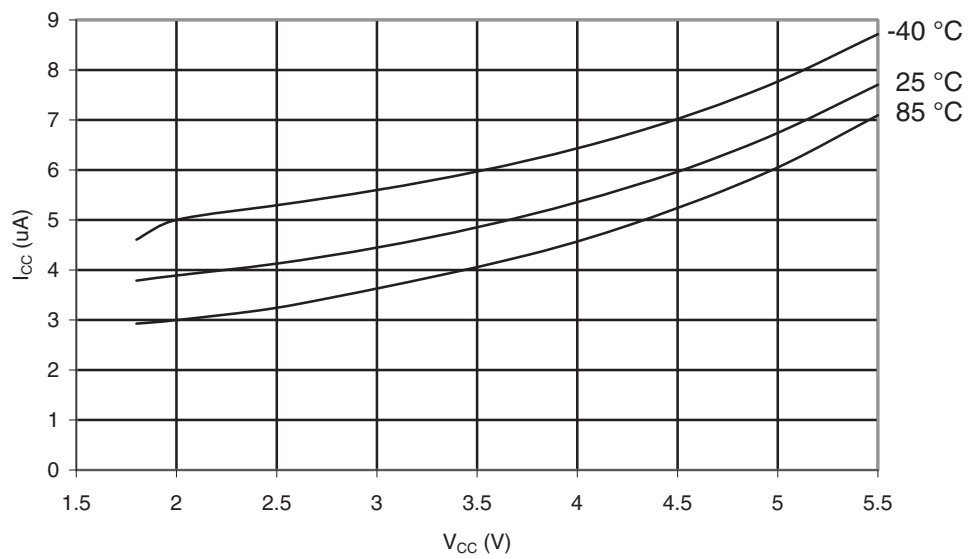
Figure 29-46. ATmega164A: Watchdog Timer Current vs. V_{CC}
