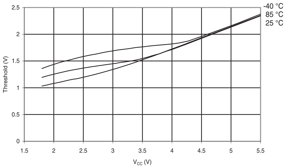
Figure 29-126. ATmega324A: Reset Pin Input Threshold vs. V_{CC} ( V_{IH} , I/O Pin Read as '1').
