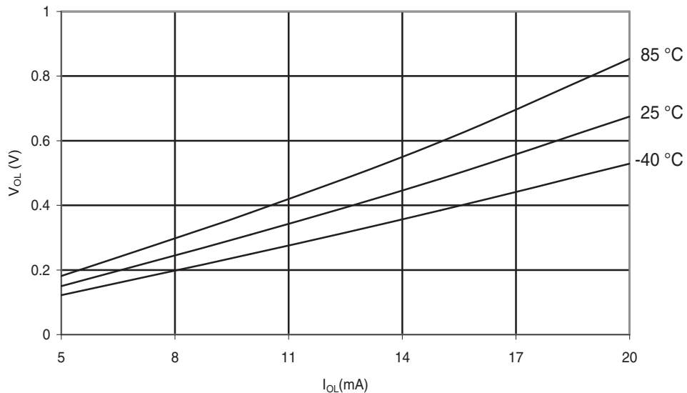
Figure 29-168. ATmega324PA: I/O Pin Output Voltage vs. Sink Current ( V_{CC} = 3V ).
