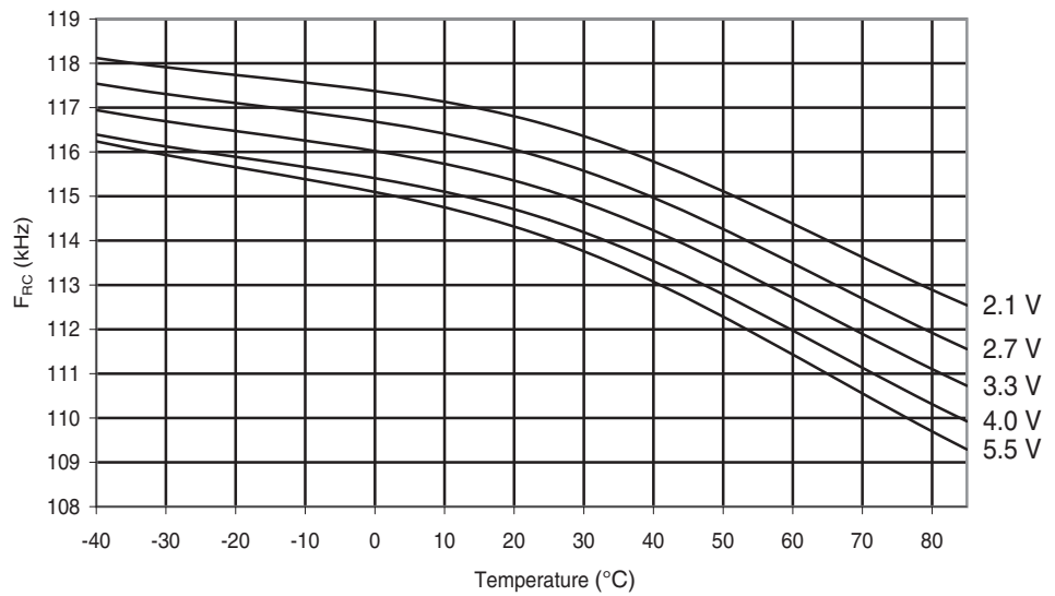
Figure 29-281. ATmega644PA: Watchdog Oscillator Frequency vs. Temperature
