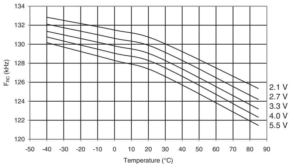
Figure 29-85. ATmega164PA: Watchdog Oscillator Frequency vs. Temperature
