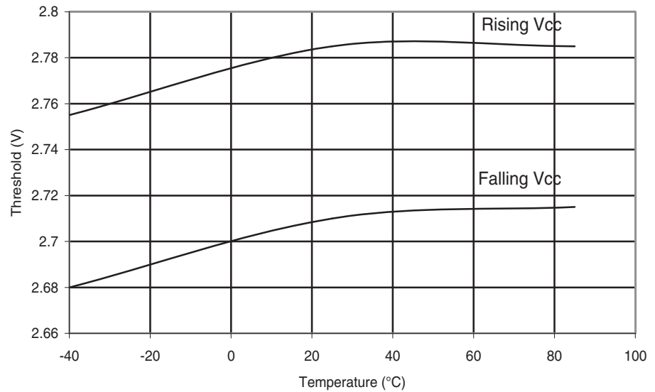
Figure 29-130. ATmega324A: BOD Threshold vs. Temperature ( V_{BOT} = 2.7V )
