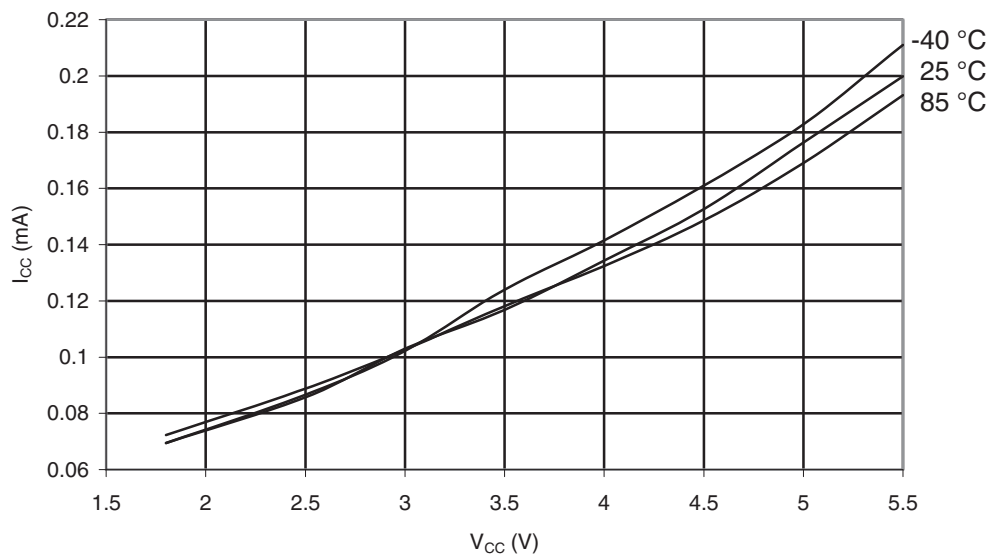
Figure 29-201. ATmega644A: Active Supply Current vs. V_{CC} (Internal RC Oscillator, 128kHz).
