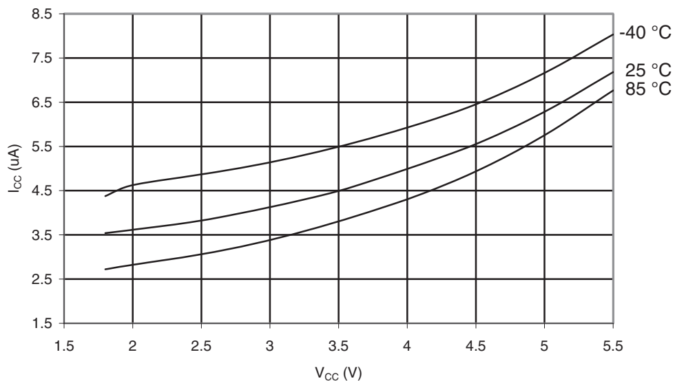
Figure 29-341. ATmega1284: Watchdog Timer Current vs. V_{CC}
