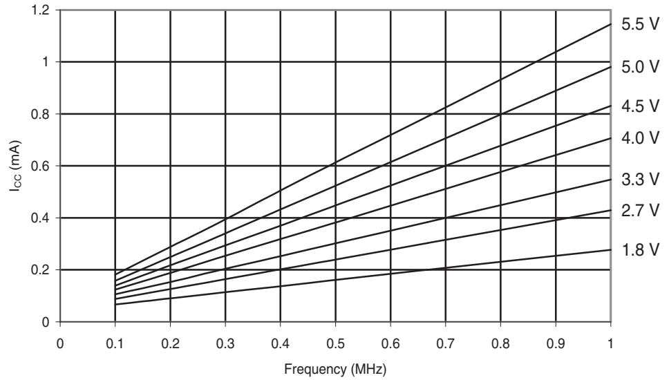
Figure 29-99. ATmega324A: Active Supply Current vs. Low Frequency (0.1 - 1.0MHz).
