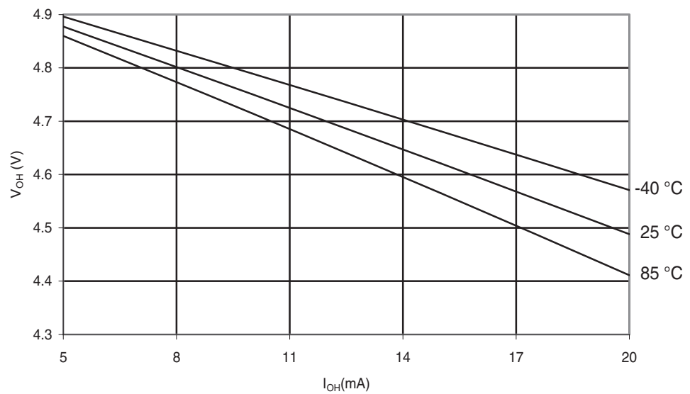
Figure 29-171. ATmega324PA: I/O Pin Output Voltage vs. Source Current ( V_{CC} = 5V ).
