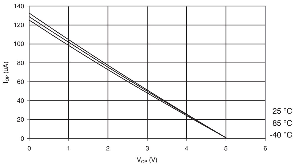
Figure 29-17. ATmega164A: I/O Pin Pull-up Resistor Current vs. Input Voltage ( V_{CC} = 5V ).
