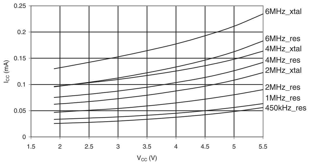
Figure 29-358. ATmega1284P: Standby Supply Current vs. V_{CC} (Watchdog Timer Disabled)
