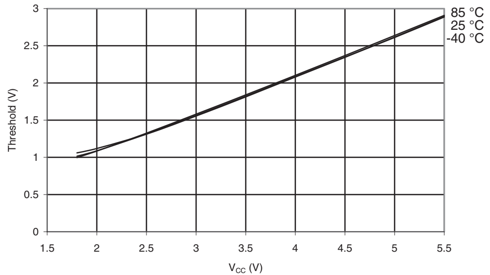
Figure 29-370. ATmega1284P: I/O Pin Input Threshold vs. V_{CC} ( V_{IH} , I/O Pin Read as '1')
