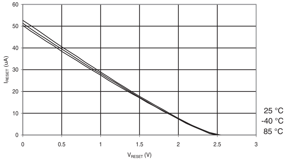
Figure 29-216. ATmega644A: Reset Pull-up Resistor Current vs. Reset Pin Voltage ( V_{CC} = 5V ).
