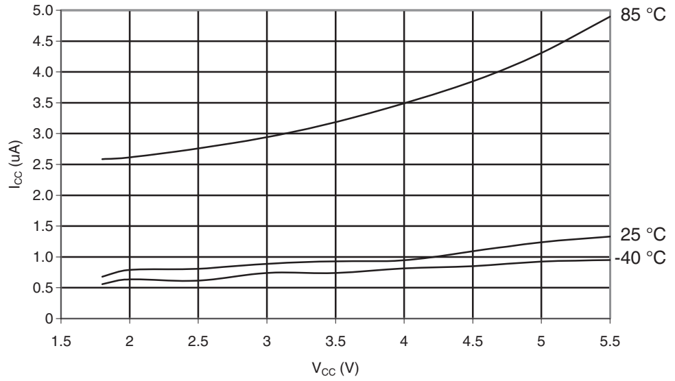
Figure 29-307. ATmega1284: Power-save Supply Current vs. V_{CC} (Watchdog Timer Disabled and 32kHz Crystal Oscillator Running)
