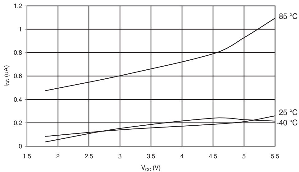
Figure 29-158. ATmega324PA: Power-down Supply Current vs. V_{CC} (Watchdog Timer Disabled).
