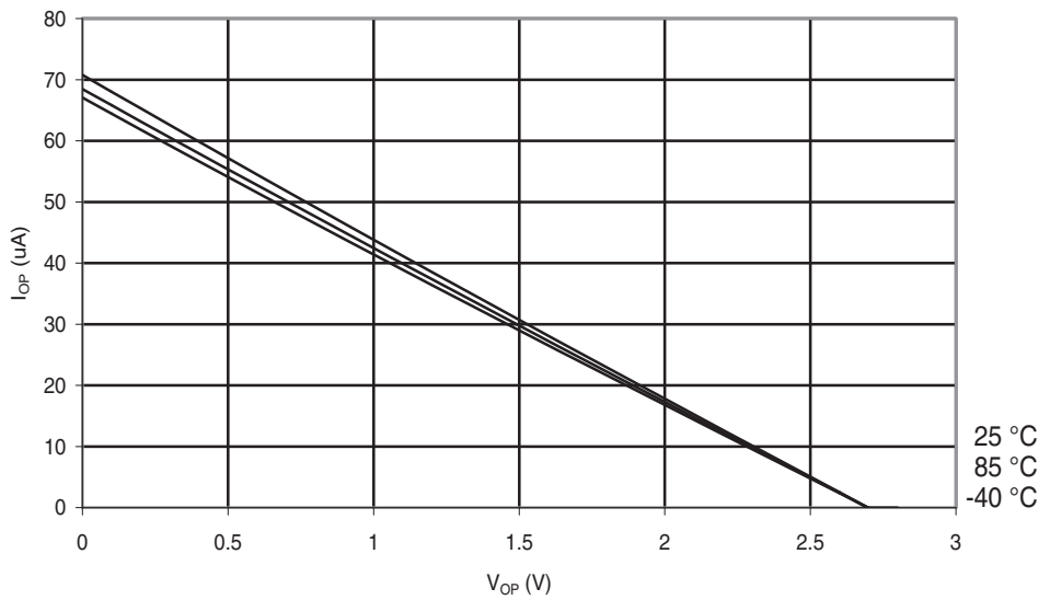
Figure 29-261. ATmega644PA: I/O Pin Pull-up Resistor Current vs. Input Voltage ( V_{CC} = 2.7V ).
