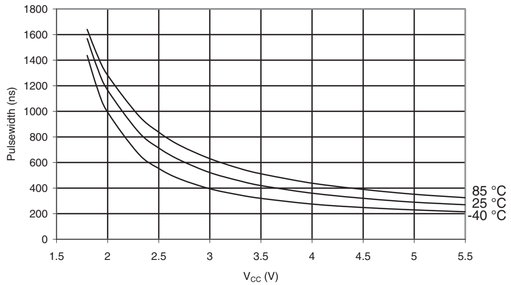
Figure 29-394. ATmega1284P: Minimum Reset Pulsewidth vs. V_{CC}
