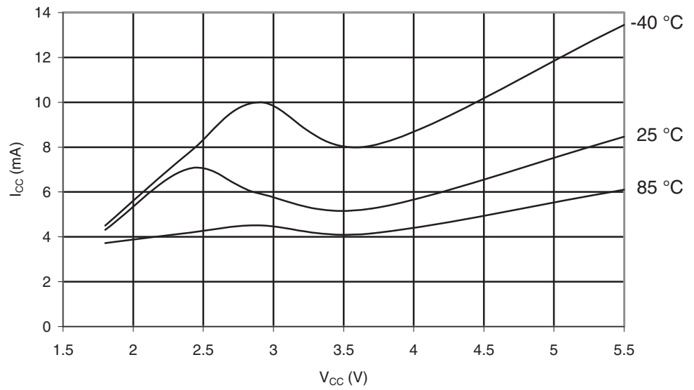
Figure 29-340. ATmega1284: Programming Current vs. V_{CC}
