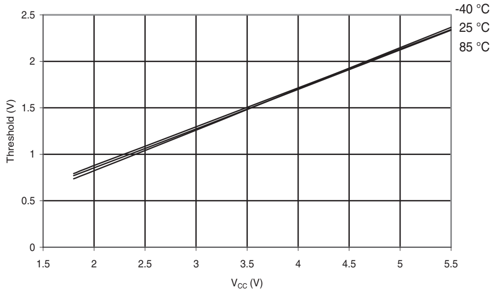
Figure 29-176. ATmega324PA: Reset Pin Input Threshold vs. V_{CC} ( V_{IL} , I/O Pin Read as '0').
