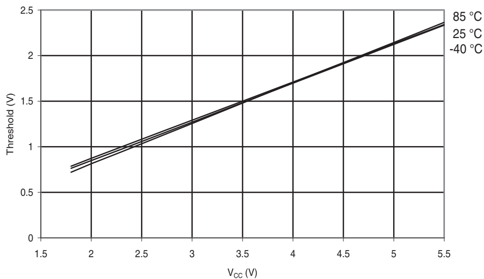
Figure 29-222. ATmega644A: I/O Pin Input Threshold vs. V_{CC} ( V_{IL} , I/O Pin Read as '0').
