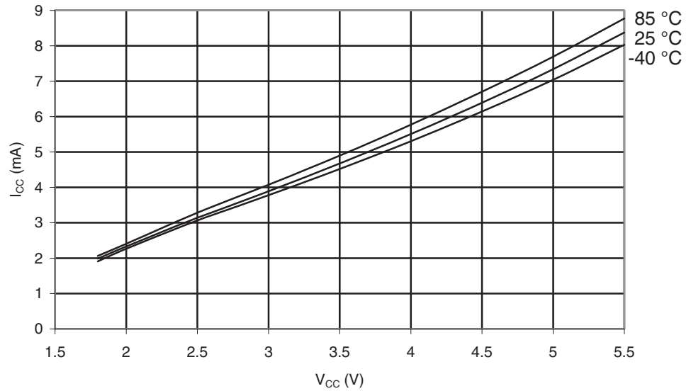
Figure 29-348. ATmega1284P: Active Supply Current vs. V_{CC} (Internal RC Oscillator, 1MHz)
