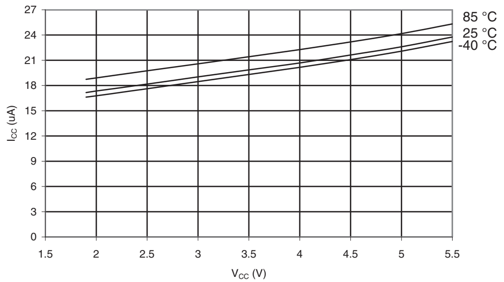
Figure 29-44. ATmega164A: Brownout Detector Current vs. V_{CC}
