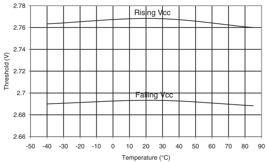
Figure 29-32. ATmega164A: BOD Threshold vs. Temperature ( V_{BOT} = 2.7V )
