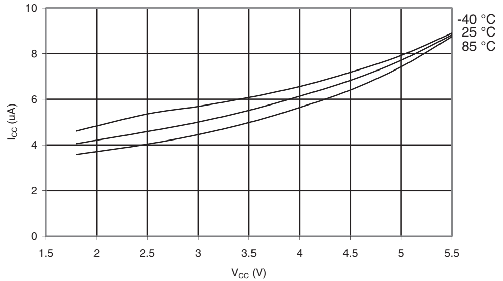
Figure 29-12. ATmega164A: Power-down Supply Current vs. V_{CC} (Watchdog Timer Enabled).
