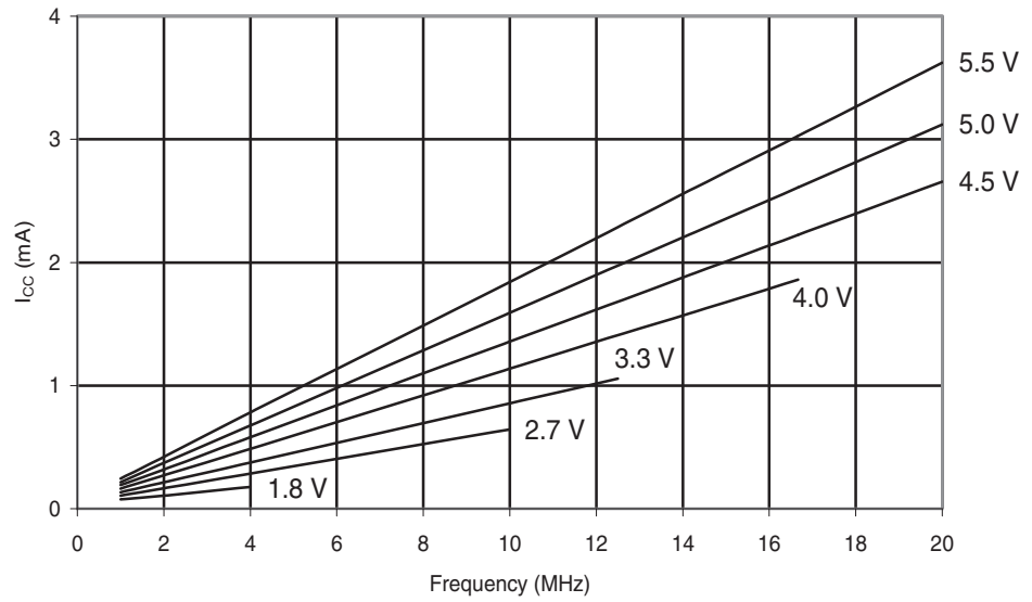
Figure 29-105. ATmega324A: Idle Supply Current vs. V_{CC} (1 - 20MHz).
