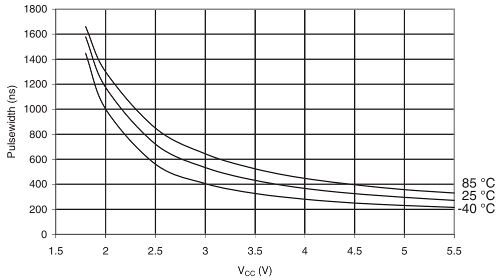
Figure 29-245. ATmega644A: Minimum Reset Pulsewidth vs. V_{CC}
