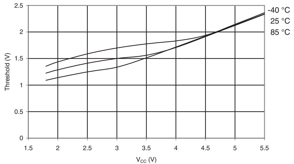
Figure 29-28. ATmega164A: Reset Pin Input Threshold vs. V_{CC} ( V_{IH} , I/O Pin Read as '1').
