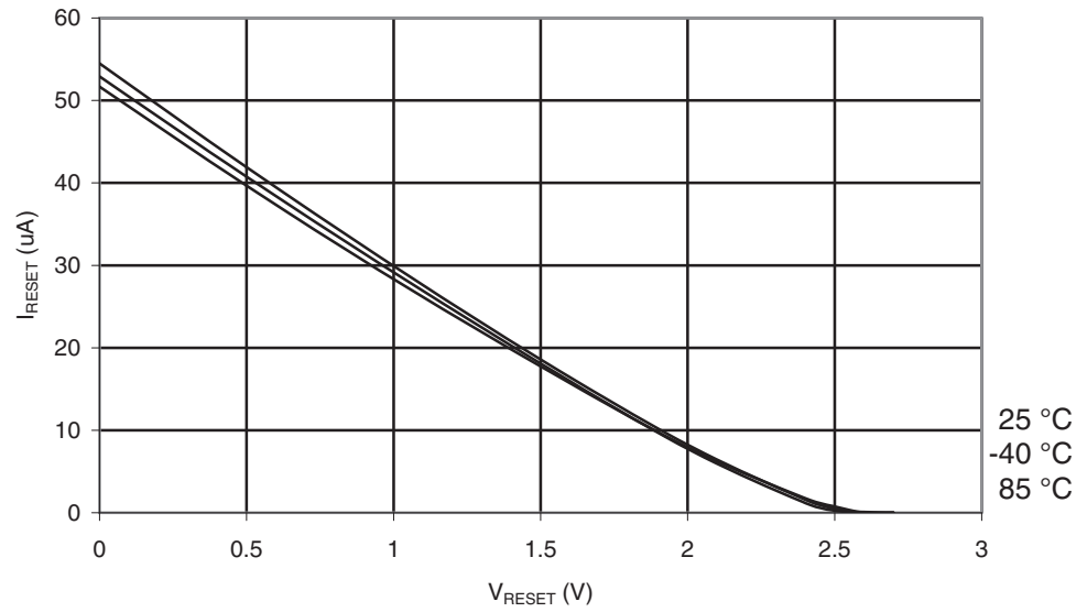
Figure 29-314. ATmega1284: Reset Pull-up Resistor Current vs. Reset Pin Voltage ( V_{CC} = 5V )
