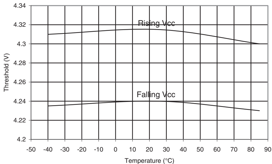
Figure 29-80. ATmega164PA: BOD Threshold vs. Temperature ( V_{BOT} = 4.3V )
