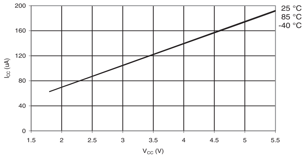
Figure 29-43. ATmega164A: AREF External Reference Current vs. V_{CC}
