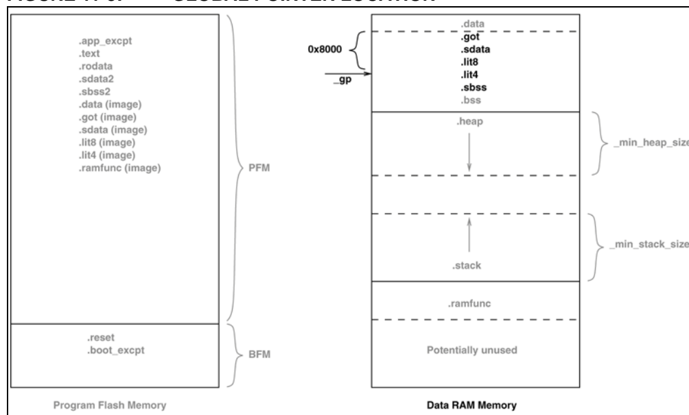
FIGURE 11-3: GLOBAL POINTER LOCATION
