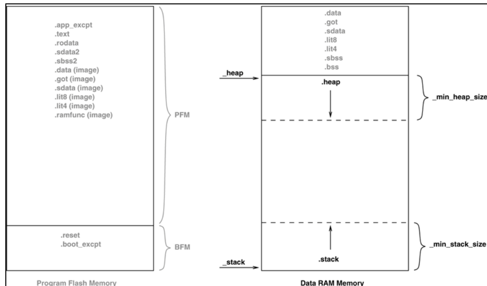
FIGURE 11-1: STACK AND HEAP LAYOUT
