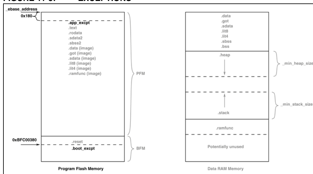
FIGURE 11-5: EXCEPTIONS
