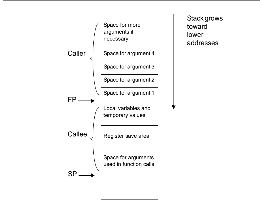
FIGURE 6-1: STACK FRAME
