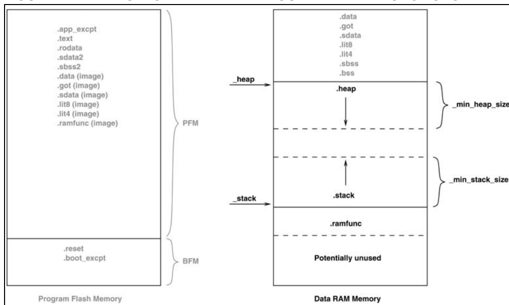
FIGURE 11-2: STACK AND HEAP LAYOUT WITH RAM FUNCTIONS
