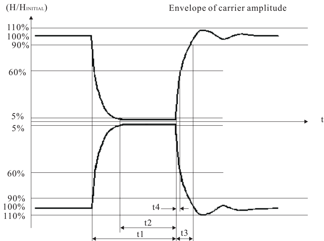
Figure 1 — Pulse shape
