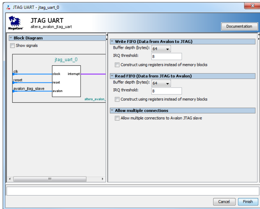
Figure 14. Define the JTAG UART interface.
