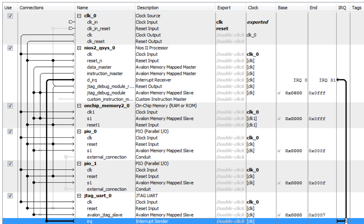
Figure 15. Connect the IRQ line from the JTAG UART to the Nios II processor.
